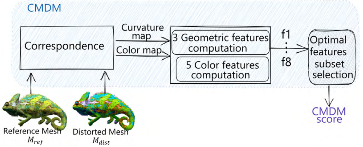
Figure 6.1: Overview of the proposed metric CMDM .
