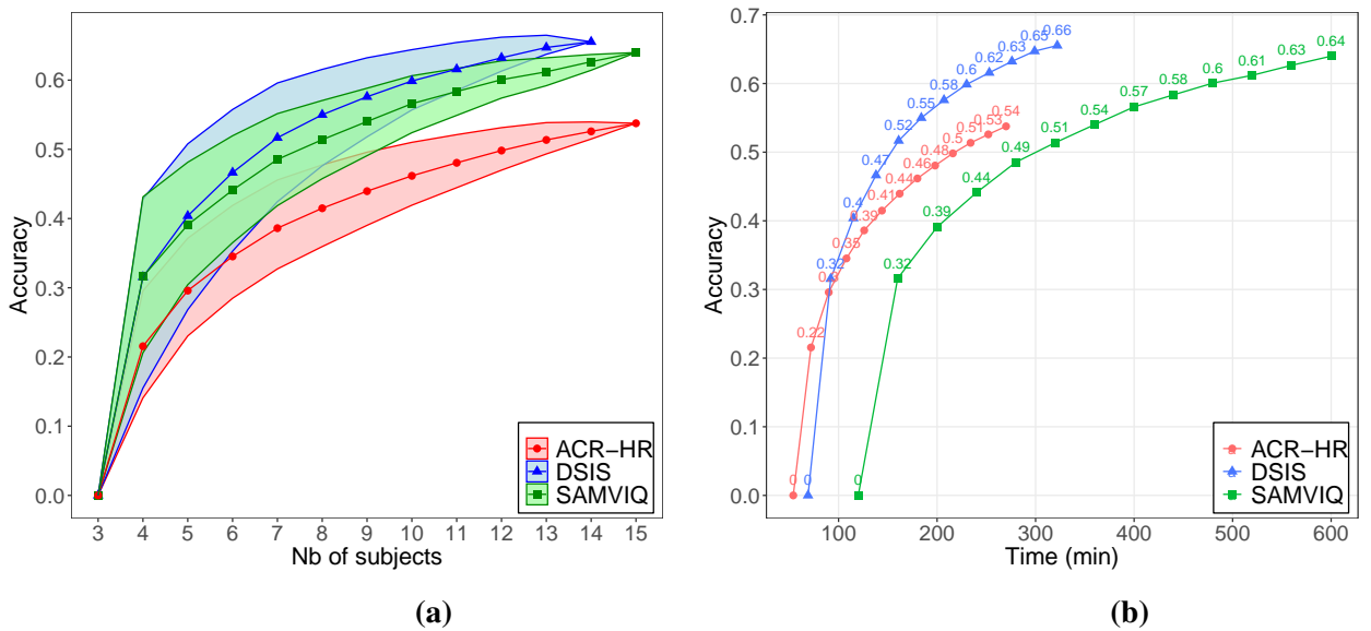
Figure 2.16: Variation of the accuracy according to the number of subjects (a) and time-effort (b) for the tested methodologies. The accuracy (y-axis) is defined as the percentage of pairs of stimuli whose qualities were assessed as statistically different. Curves represent mean values of these percentages and areas around curves represent 2.5th - 97.5th percentiles.
