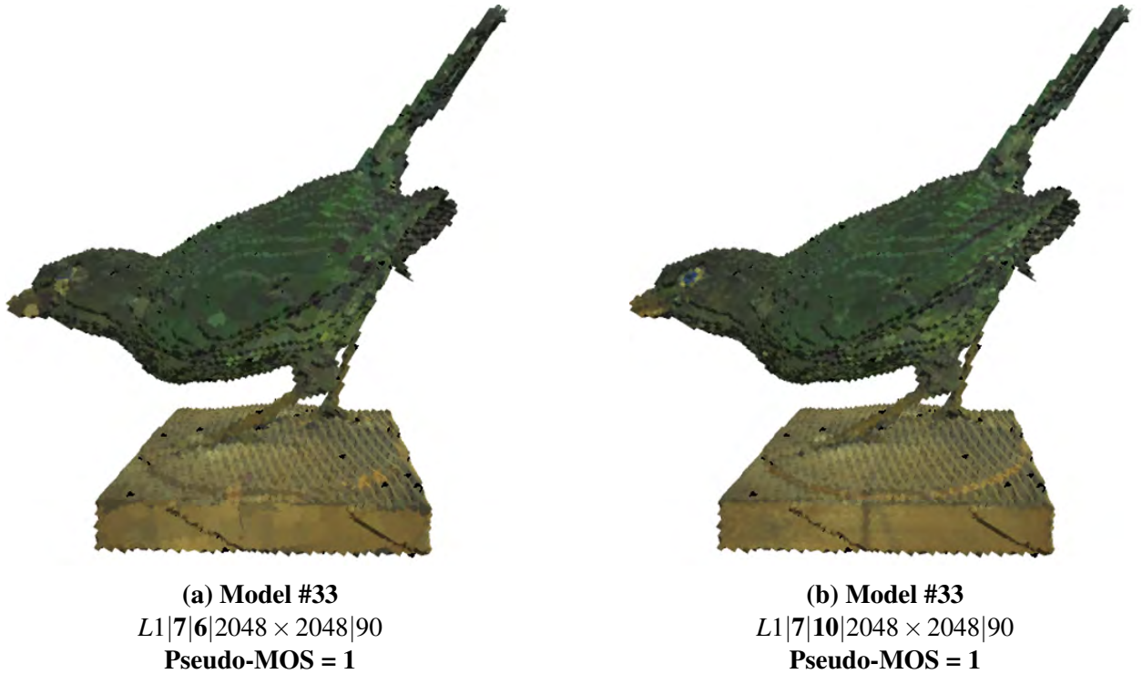
Figure 5.16: Visual example illustrating the interaction between the geometry and texture coordinate quantization regarding the perceived quality. Acronyms refer to the following combination of distortion parameters: LoD_{sim}L|qp|qt|T_S|T_Q .
