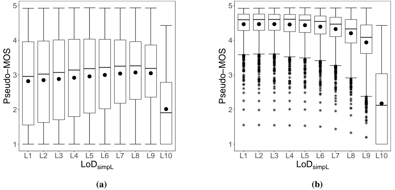
Figure 5.11: (a) Boxplots of MOSs obtained for the LoD simplification LoD_{simplL} . (b) Boxplots of MOSs obtained for the LoD simplification, but restricted to the least quantized models ( qp = 11 & qt = 10 ). Mean values are displayed as circles.
