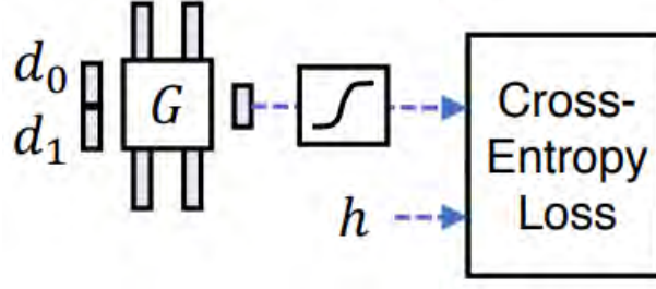
Figure 7.2: Training on 2AFC: a small network G is trained to predict perceptual judgment h from distance pair (d_0, d_1) . This figure is reprinted from [4].
