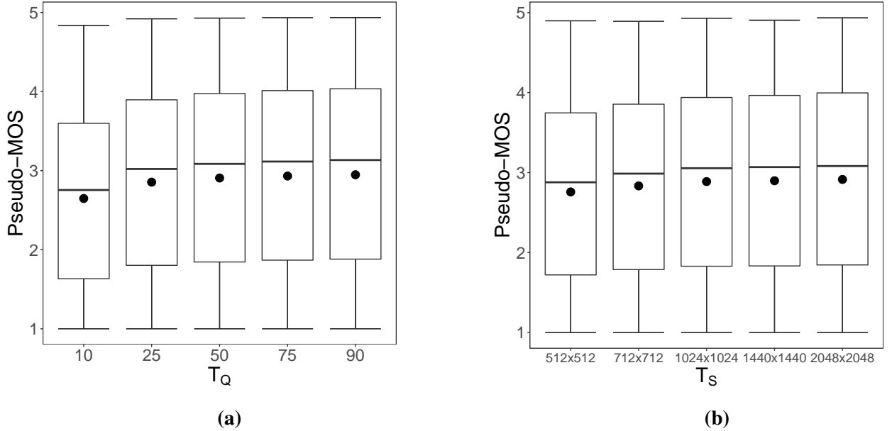
Figure 5.12: Boxplots of MOSs obtained for the texture (a) compression T_Q and (b) sub-sampling T_S . Mean values are displayed as circles.
