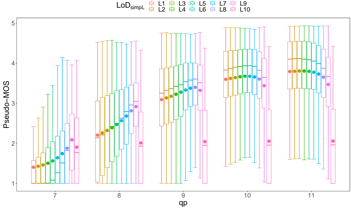
Figure 5.13: Boxplots of MOSs illustrating the interaction between the LoD simplification LoD_{simplL} and the quantization of the model's positions qp .
