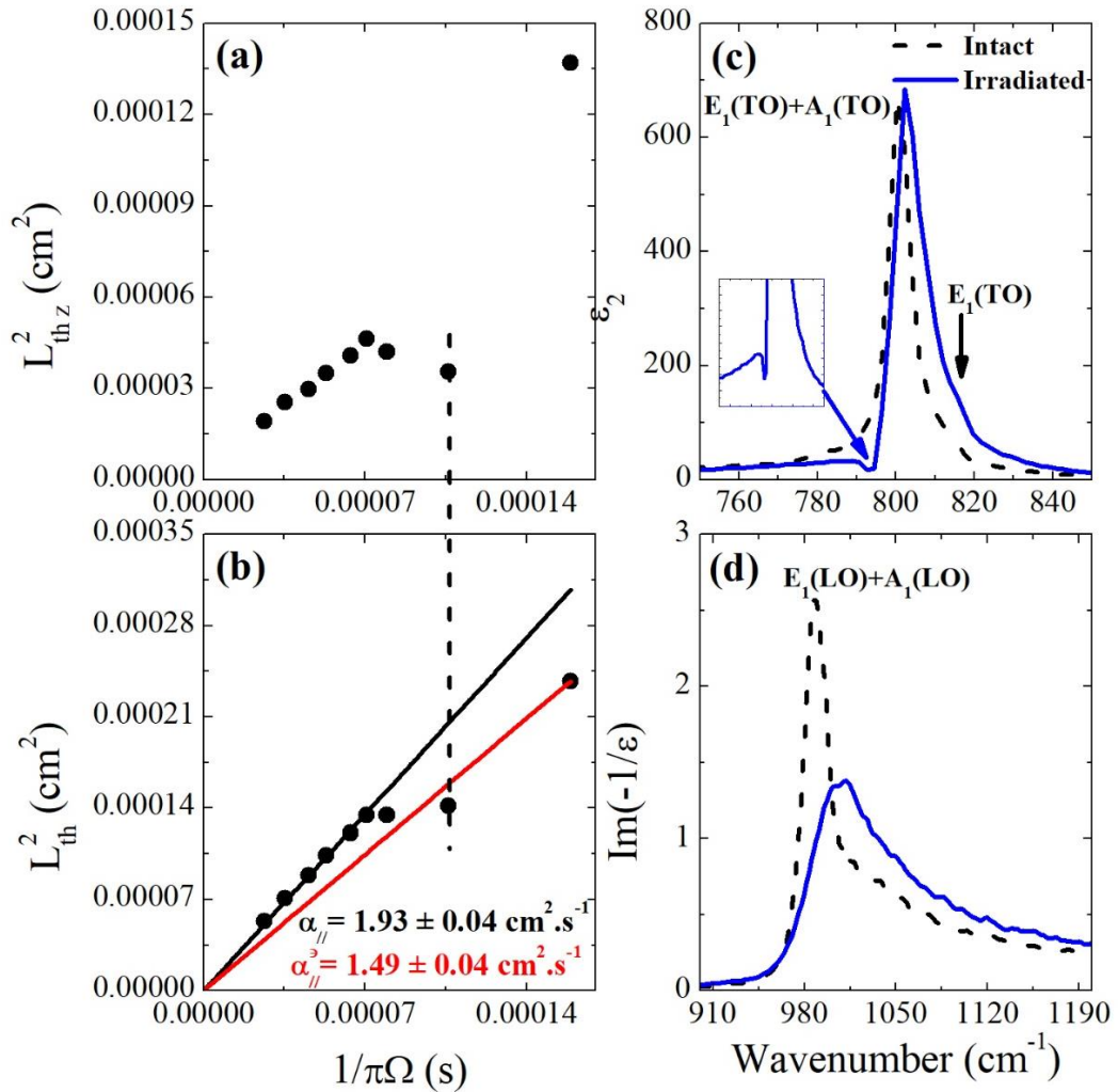
Figure 4.7 Infrared analysis of 4H-SiC substrate irradiated with protons at 3MeV with a dose of 2.0 \times 10^{16} H^+ ions/cm 2 . (a) Square of cross-plane thermal diffusion length L_{th,z}^2 vs. the inverse of the heating beam modulation frequency. (b) Square of in-plane thermal diffusion length L_{th}^2 vs. the inverse of the heating beam modulation frequency. The slopes of the straight line passing through origin that best fit the data points give the in-plane thermal diffusivity for high and low heating beam modulation frequencies. The uncertainties are determined by the experiment sensitivity and the scatter in the data points. The vertical dashed line is introduced to highlight the fact that L_{th,z}^2 and L_{th}^2 undergo the strongest deviation from the linear behavior for the same modulation frequency. (c) Imaginary parts of the infrared dielectric functions of intact 4H-SiC and the irradiated sample. (d) Imaginary parts of the inverse of the negative of the dielectric functions of intact 4H-SiC and the irradiated sample.
