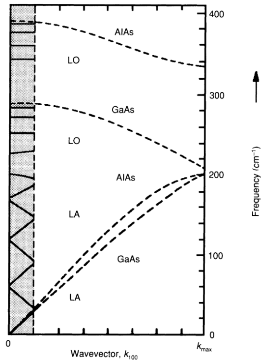
Figure 1.7 Dispersion relations for the LO and LA phonons in bulk GaAs and AlAs. LO phonons don't propagate throughout a GaAs-AlAs superlattice, however, LA phonons do. The shaded space shows folded dispersion curves for a superlattice whose period is far larger than the lattice spacing. [16]
