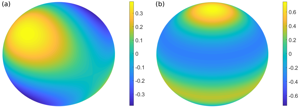
Figure 33: Examples of spherical harmonic functions. (a) \psi_{2,1} (b) \psi_{3,0}
