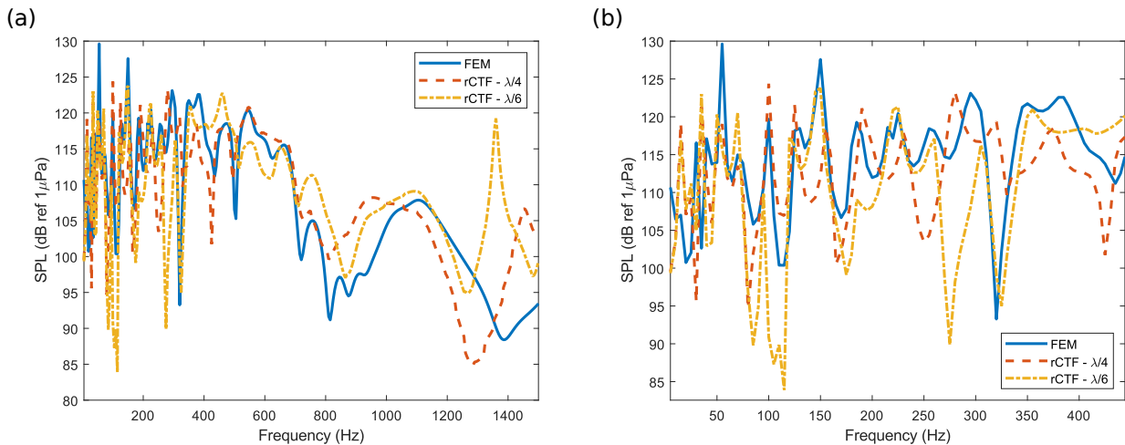
Figure 92: Evaluation of the influence of the criterion for the size of the segments when removing the full patch. (a) Results in the whole frequency range. (b) Zoom in the low frequency range.
