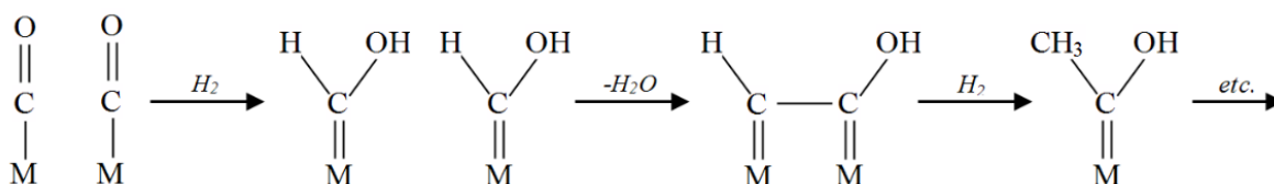
Figure 1.15. Chain growth pattern in CO insertion mechanism, R represents H or alkyl group.
