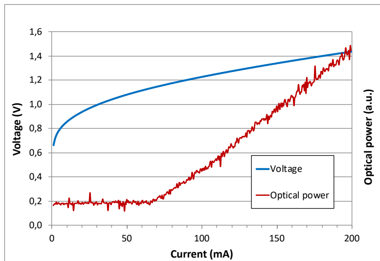
Figure 110. DFB laser electrical and optical characterization. The optical power was collected from the monitor optical port.
