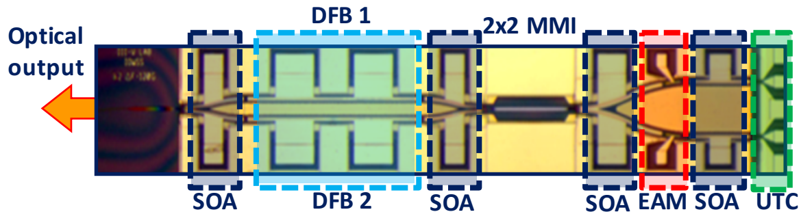
Figure 132. Picture of the IPHOS PIC with the different monolithically integrated devices
