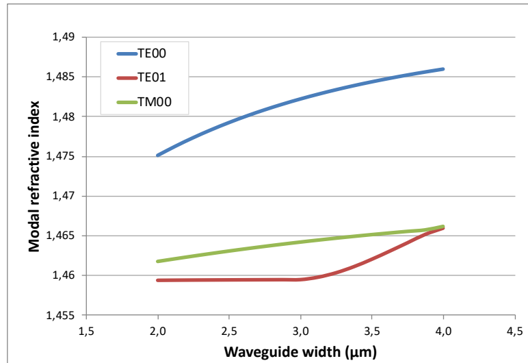
Figure 33. Simulation of effective refractive indices of the two first TE ( TE_{00} , TE_{01} ) modes and the first TM ( TM_{00} ) mode of a 90nm thick waveguide. The single mode cut-off width is below 3 \mu\text{m} . Silica index is 1.46.
