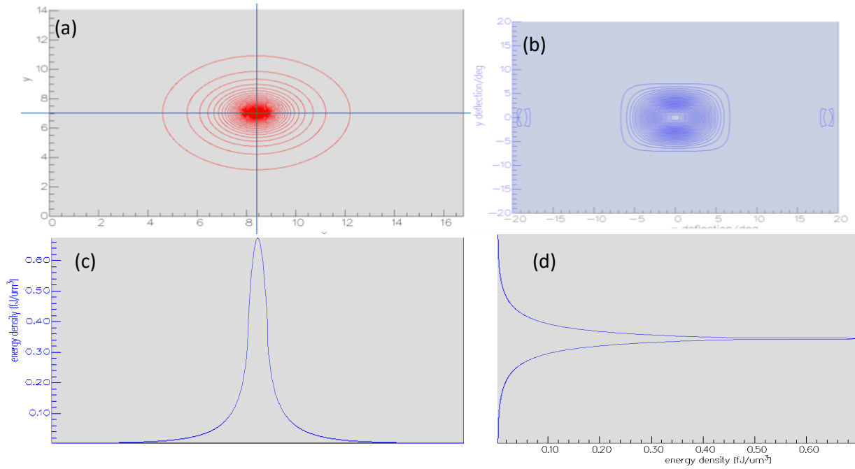
Figure 41. FIMMWAVE simulation of the computed optical mode (a) and mode divergence (b) for a 90 nm * 800 nm waveguide. Figures (c) and (d) show the horizontal and vertical cut of the modal intensity profile.
