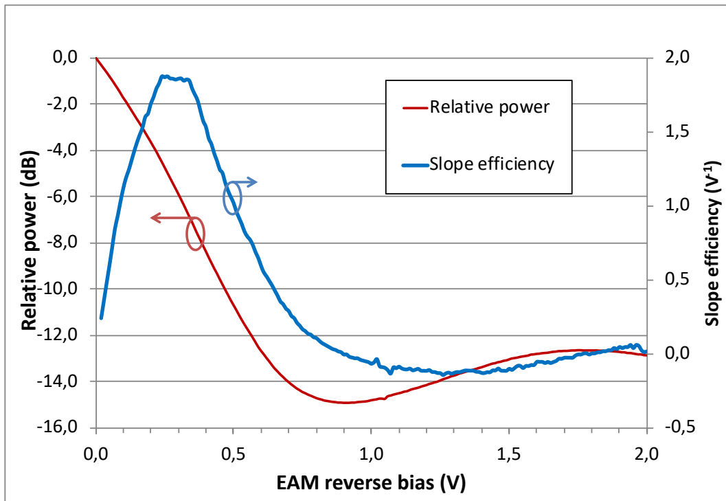
Figure 118. Measured relative power and slope efficiency of the devices produced with this fabrication run.
