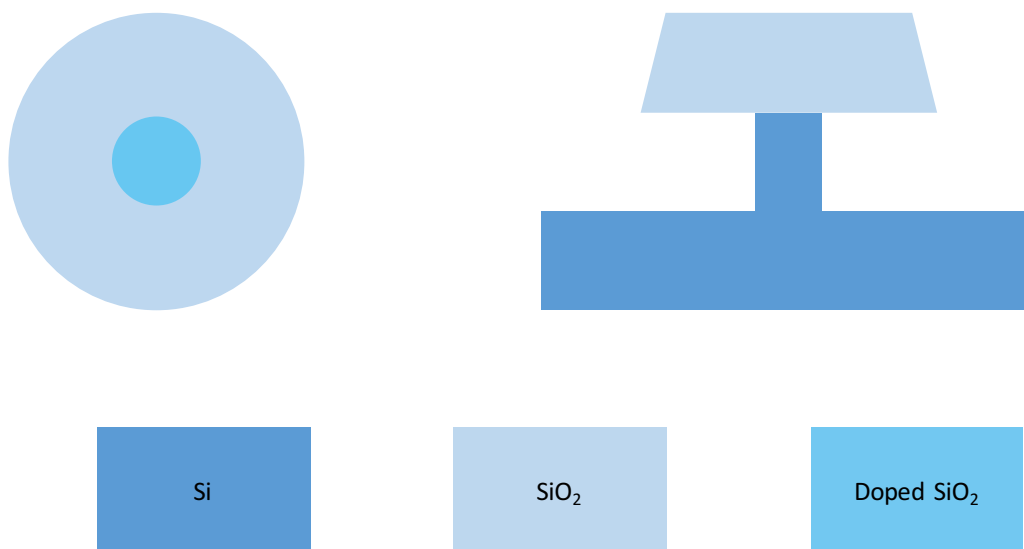
Figure 25. Silica-based waveguides described throughout the paragraph. Left: channel waveguide. Right: suspended silica waveguide on silicon pillar. Bottom: color code for the different materials
