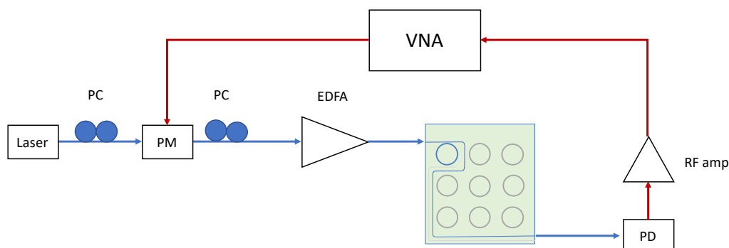
Figure 143. Measurement setup for phase modulation measurement on the through
