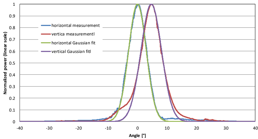
Figure 75. Far field divergence profile of a 800nm wide SSC for horizontal and vertical cut. The mode size extracted from the gaussian fit is 9.4 \mu\text{m} \times 8 \mu\text{m} .
