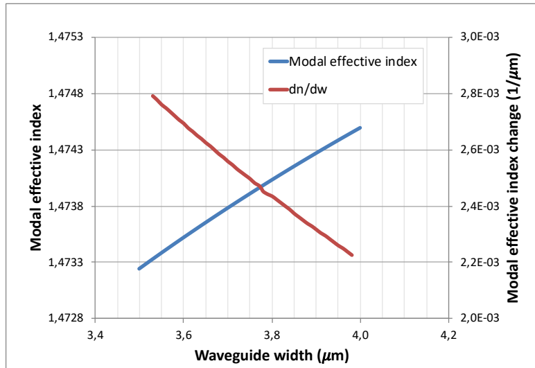
Figure 45. Simulated modal effective index with waveguide width for Bragg grating design.
