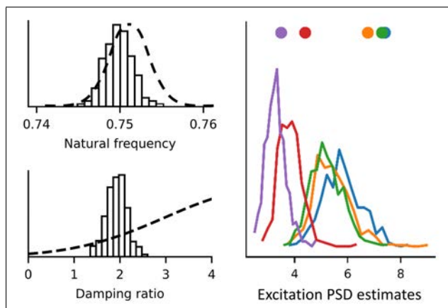
Figure 5.5 Posterior density distributions for the damping \xi , frequency f_0 and modal excitation \alpha_{1...5}^2 . Left : the histograms represent the sampled posterior while the dashed line represent the priors. The densities are normalized such that they can be presented jointly. Left and right : the bullets symbolize the theoretical values
