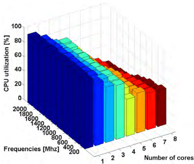
Figure 4.11 – GPP utilization as a function of the number of active cores and the processing frequencies (platform: Odroid-xu3, video sequence: kimono, bitrate: 1831 Kbps, frame rate: 25 Hz, resolution: 1080p)
