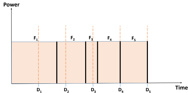
Figure 2.12 – Average workload-based DVFS
