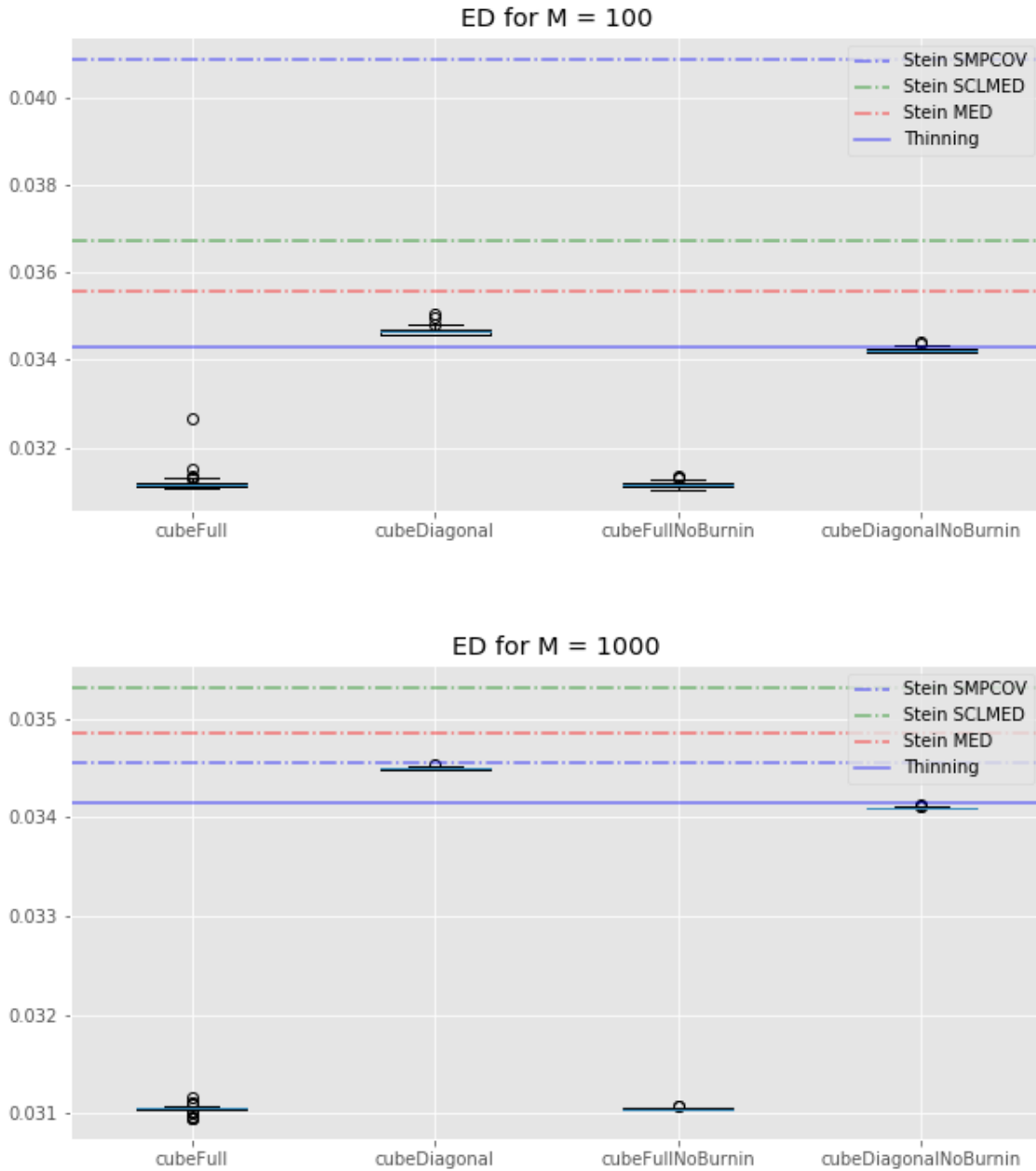
Figure 4.4.: Lotka-Volterra example: boxplots of the energy distance for all the cube method variations, the KSD method for three kernels and the usual thinning method. Top: M = 100 . Bottom: M = 1000 .
