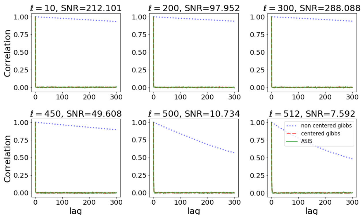
Figure C.1.: Examples of autocorrelations for EE components for full sky experiment, Section 3.7.1.
