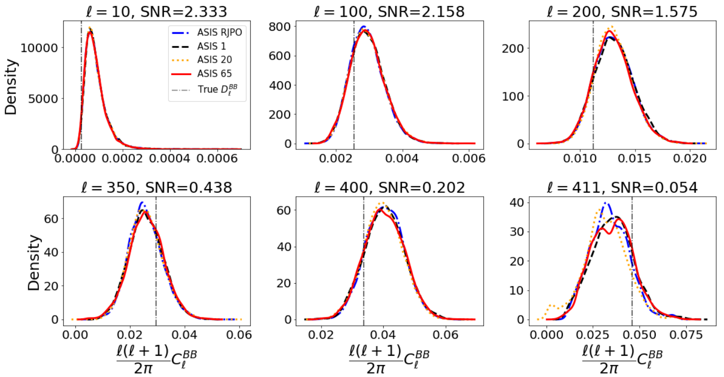
Figure C.8.: Kernel density estimation of marginals for a sample of multipoles for BB components for cut-sky experiment, Section 3.7.2.
