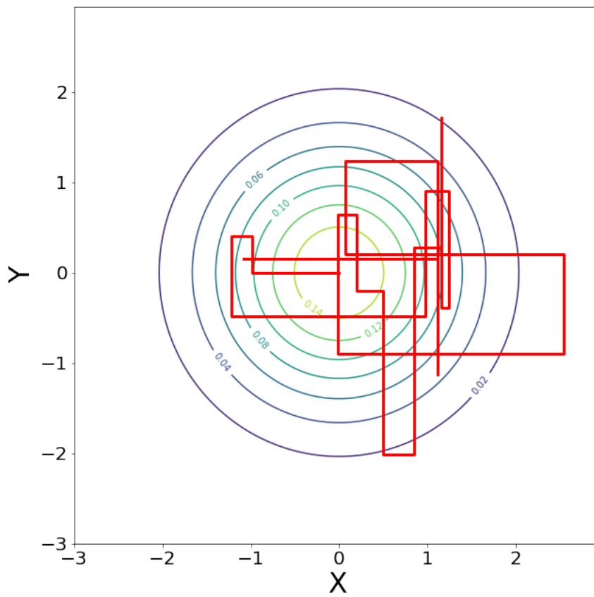
Figure B.1.: Trace plot, in red, of the Gibbs sampler targeting the joint distribution of (X, Y) for \rho = 0 , described in Appendix B. The circles are the level sets of the normal distribution.
