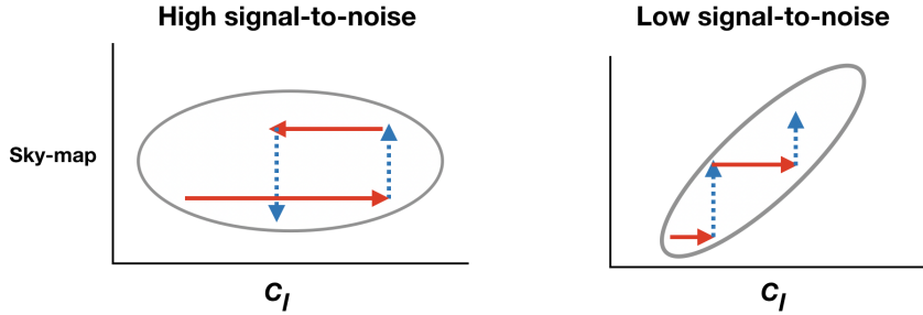
Figure 3.2.: Example of a sequence of consecutive samples of the Gibbs sampler in the centered parametrization. For low signal-to-noise power spectrum coefficients, shown in the right panel, the sky map and the power spectrum are strongly correlated. This leads to the bad mixing of the algorithm in this regime and a large number of samples is needed to explore the posterior for such components. This is not the case of the high signal-to-noise components shown in the left panel. Here, the correlations are small and the resulting mixing of the algorithm is good with many fewer samples needed to explore the posterior. In both panels the red plain arrows depict sampling of the power spectrum given the sky map and the blue dotted arrows sampling the sky map given the power spectrum.
