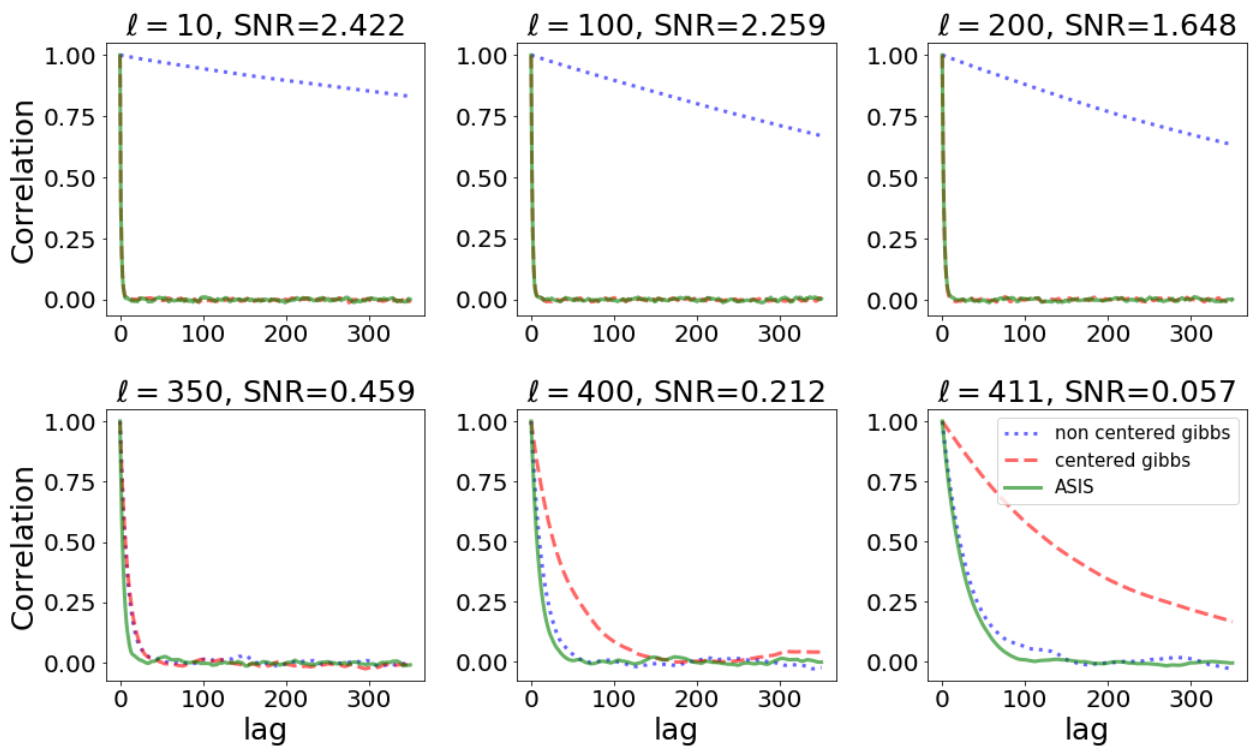
Figure C.2.: Examples of autocorrelations for BB components for full sky experiment, Section 3.7.1.
