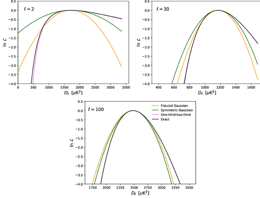
Figure 2.5.: Plot of the true likelihood of D_\ell = \frac{\ell(\ell+1)}{2\pi} C_\ell and different likelihood approximation. We assume full sky observation and no noise. This figure is taken from Gerbino et al. (2020)
