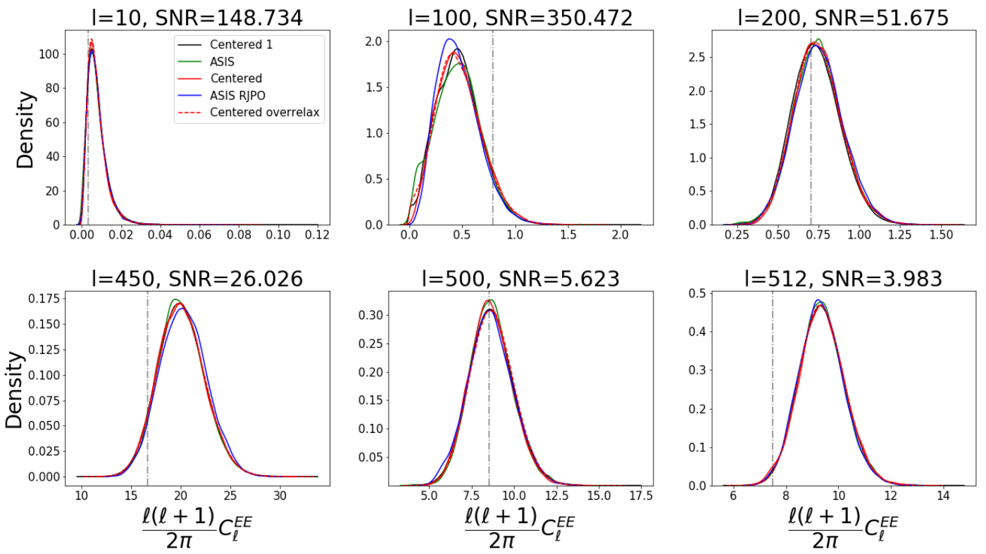
Figure C.11.: Kernel density estimation of the posterior density on EE cut-sky experiment, Section 3.7.3.
