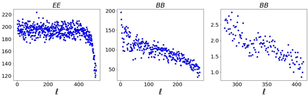
Figure 3.8.: Ratios of Integrated Autocorrelation Time against multipole of non centered Gibbs on interweaving. Note that the BB components are split in two graphs for readability, because of the very broad range of scales.
