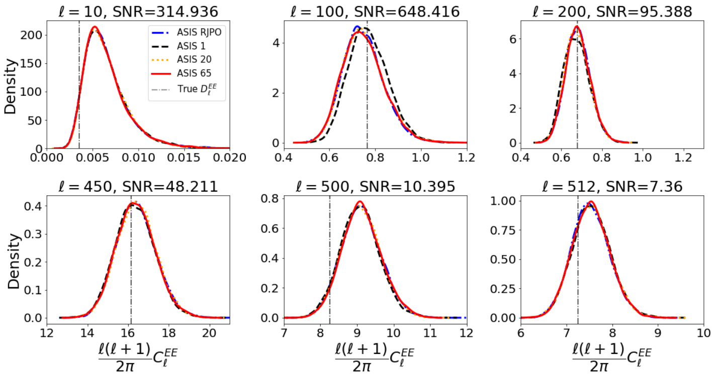
Figure C.7.: Kernel density estimation of marginals for a sample of multipoles for EE components for cut-sky experiment, Section 3.7.2.
