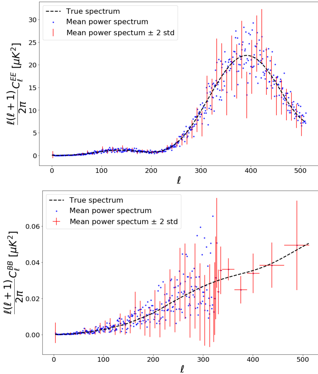
Figure 3.14.: An example of the constraints on the power spectra derived using the Centered overrelax algorithm in the case of the ground-based experiment discussed in the text. The black dashed lines show the true input spectra. The blue points show the best power estimates in each bin equal to the mean power computed over the generated chains. The vertical bars of the crosses correspond to the mean plus/minus one standard deviation, and the horizontal bars the corresponding bins in \ell . We only plot the crosses for one every ten multipoles on the non binned part. We plot the crosses for every multipole on the binned part. The top panel shows the EE power spectrum and the bottom – the BB one. The input CMB maps assumed the standard cosmological model with the assumed tensor-to-scalar ratio r = 0.001 .
