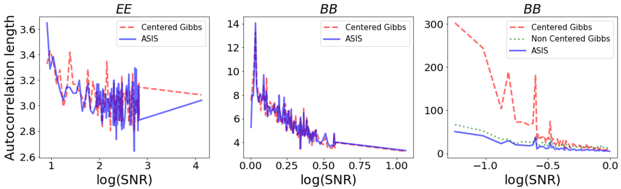
Figure 3.6.: Integrated autocorrelation time against \log(\text{SNR}) for each algorithm. The BB components are split into two graphs for readability, because of the very different scales.
