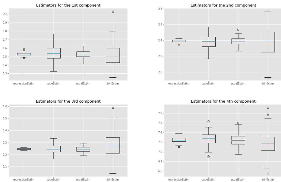
Figure 4.5.: Truncated normal example: box-plots over 100 independent replicates of each estimator; see text for more details.
