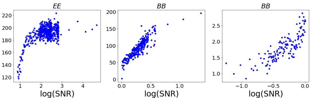
Figure 3.10.: Ratios of Integrated Autocorrelation Time against signal-to-noise ratio for non centered Gibbs on interweaving. Note that the BB components are split in two graphs for readability, because of the very different scales.
