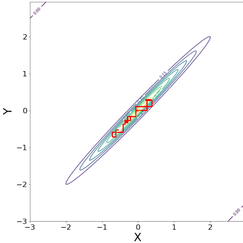
Figure B.2.: Trace plot, in red, of the Gibbs sampler targeting the joint distribution of (X, Y) for \rho = 0.99 , described in Appendix B. The circles are the level sets of the normal distribution.
