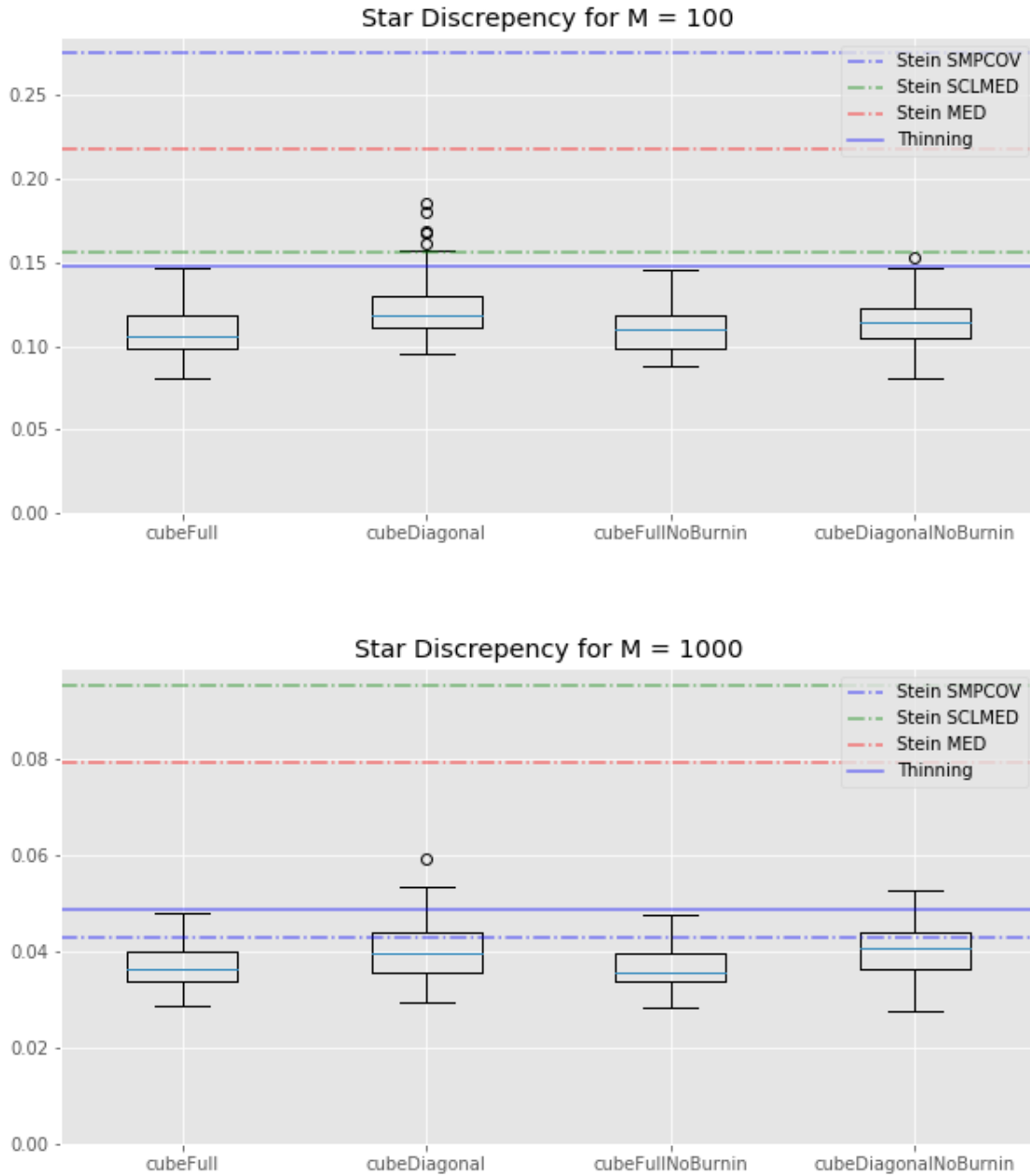
Figure 4.3.: Lotka-Volterra example: box-plots of the star discrepancy for all the cube method variations, the KSD method for three kernels and the usual thinning method. Top: M = 100 . Bottom: M = 1000 .
