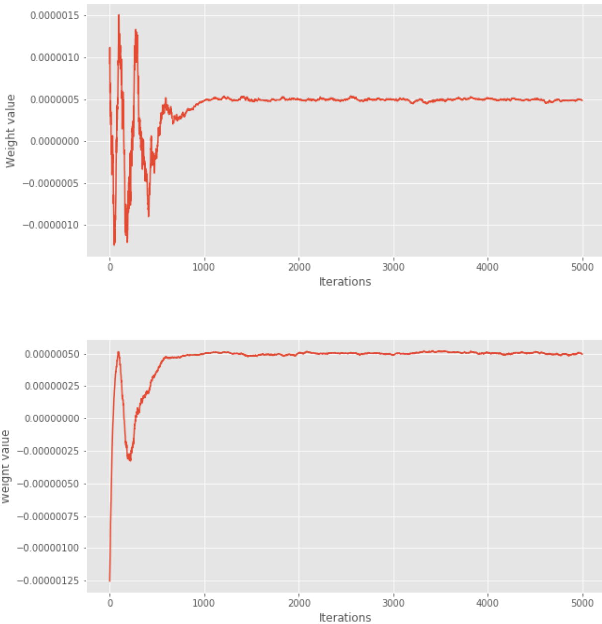
Figure 4.1.: Lotka-Volterra example: first 5000 weights of the cube methods, based on full (top) or diagonal (bottom) set of covariates.
