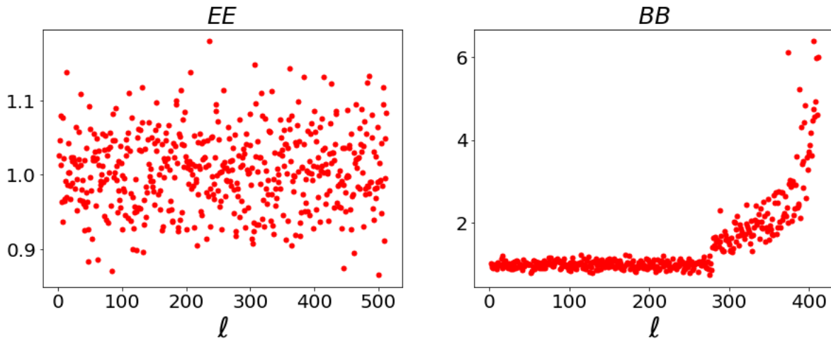
Figure 3.7.: Ratios of Integrated Autocorrelation Time against multipole. Numerator: centered Gibbs. Denominator: interleaving. A ratio superior to 1 indicates that centered Gibbs is performing better than interleaving in terms of autocorrelation time.
