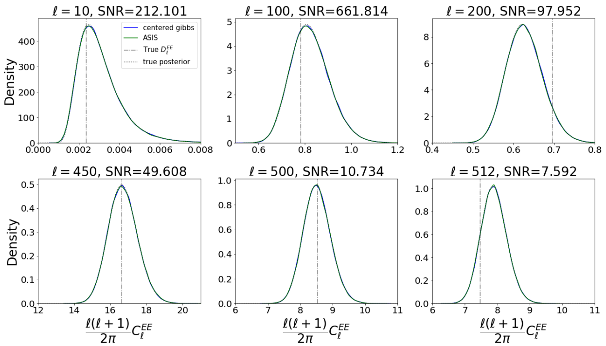
Figure C.3.: Examples of kernel density estimation of histograms for EE components for full sky experiment, Section 3.7.1. For readability and since the mixing of the non centered Gibbs is bad, we don't include its histograms on this figures.
