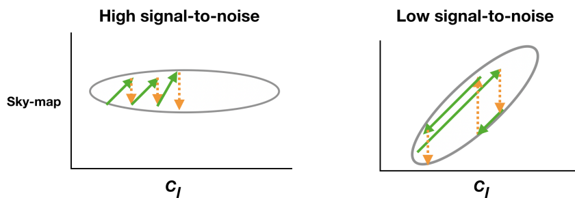
Figure 3.4.: Example of a sequence of samples of the non-centered Gibbs sampler. For low signal-to-noise power spectrum components, the sky map and the power spectrum are strong correlated, right panel. This is not the case of the high signal-to-noise components, left panel. The green plain arrows depict sampling the power spectrum given the sky map and the orange dotted arrows the sky map given the power spectrum. As shown, the non-centered Gibbs sampler explores the high signal-to-noise components much less efficiently, left panel, than the low signal-to-noise components, right panel.
