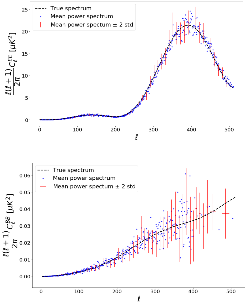
Figure 3.12.: Comparison of posterior power spectrum to the true power spectrum for the LiteBird-like experiment. The blue points correspond to the mean power spectrum. The top and bottom of the horizontal bars of the crosses correspond to the mean plus/minus two standard deviation. The horizontal bars correspond to the \ell range spanned by the binning scheme. We only plot the crosses for one every ten multipoles on the non binned part. On the binned part, we only plot the crosses for one every two multipoles. The panels show EE (top) and BB (bottom) power spectra.
