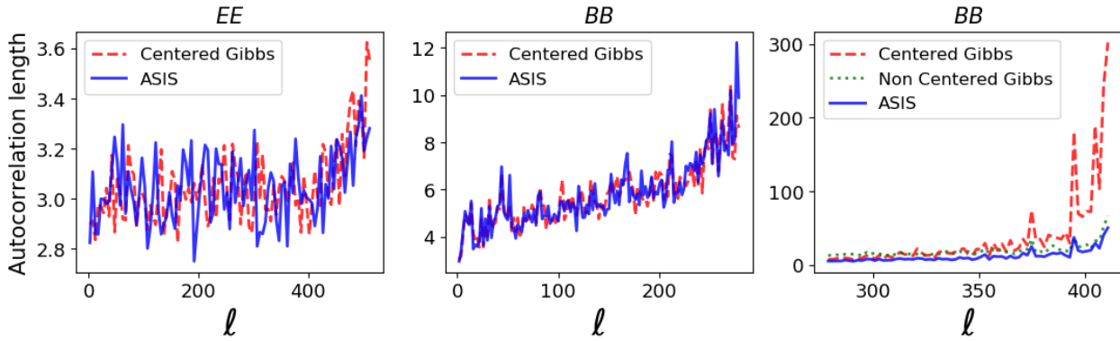
Figure 3.5.: Integrated autocorrelation times against multipole for each algorithm. The BB components are split into two graphs for readability, because of the broad range of scales they cover.
