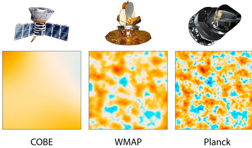
Figure 2.3.: Evolution of the resolution through the missions. The missions are in chronological order from left to right. We can notice the increasing resolution. This is a NASA/JPL-Caltech/ESA illustration. Link: https://photojournal.jpl.nasa.gov/catalog/PIA16874
