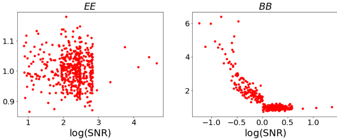
Figure 3.9.: Ratios of Integrated Autocorrelation Time against log signal-to-noise ratio of centered Gibbs on interweaving.
