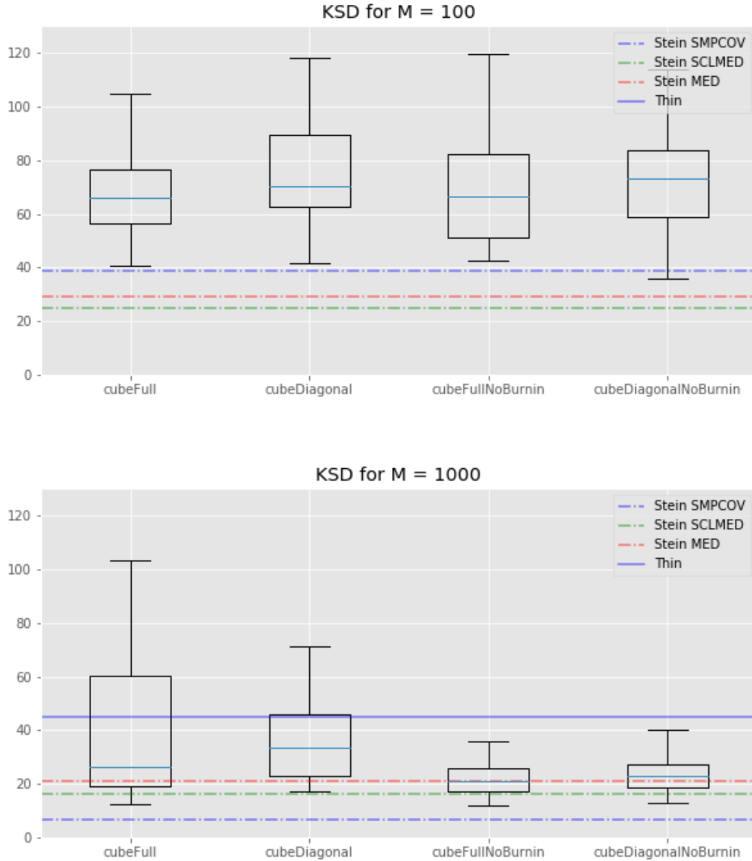
Figure 4.2.: Lotka-Volterra example: box-plots of the kernel Stein discrepancy for all the cube method variations, the KSD method for three kernels and the usual thinning method. Top: M = 100 . Bottom: M = 1000 . (In the top plot, standard thinning is omitted to improve clarity, as corresponding value is too high.)
