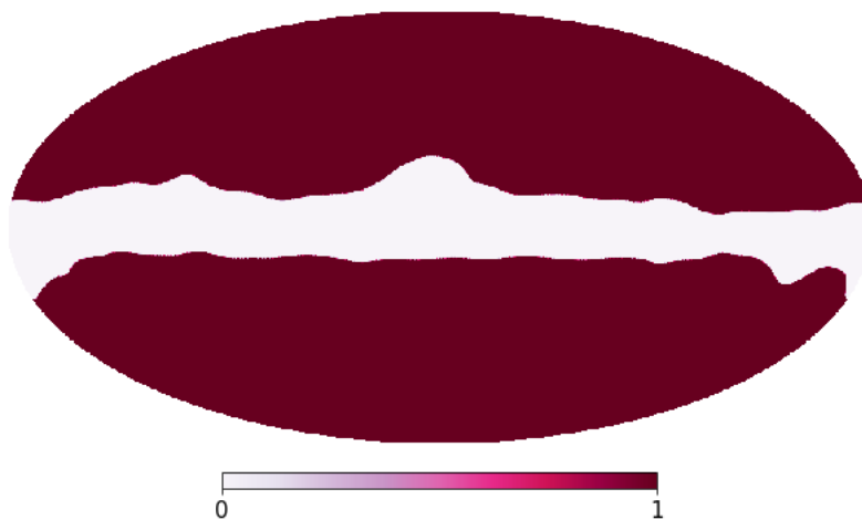
Figure C.5.: Planck sky mask used for the first cut sky experiment described in Section 3.7.2. This mask covers roughly 80% of the sky.
