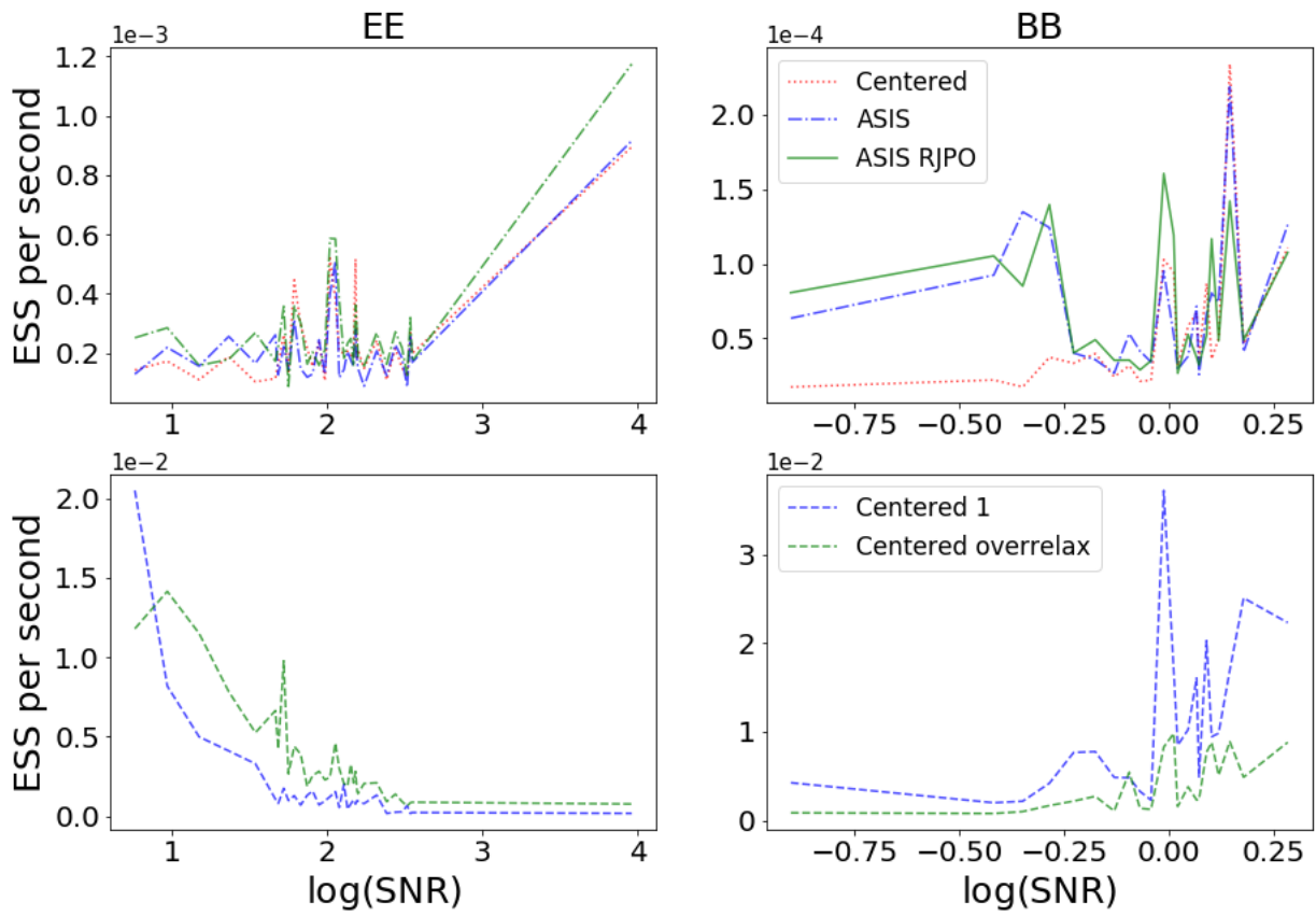
Figure 3.13.: Effective Sample Size per second against \log(\text{SNR}) for each algorithm. For the sake of clarity, we plot the results for the Centered 1 case, separately.
