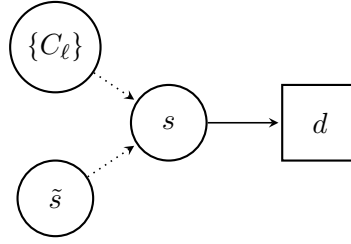
Figure 3.3.: Directed acyclic graph of the model in equation (3.13). Circles and squares represent unobserved and observed variables respectively. Plain arrows represent stochastic dependence. Dashed arrows represent deterministic dependence.
