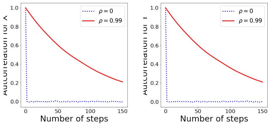
Figure B.3.: Autocorrelation plots of the Gibbs sampler, described in Appendix B, for X and Y and for \rho = 0 and \rho = 0.99 .
