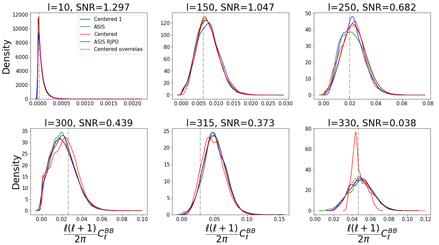
Figure C.12.: Kernel density estimation of the posterior density on BB for cut-sky experiment, Section 3.7.3.
