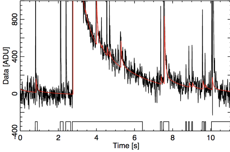
Figure 2.4.: Example of time-ordered data of a detector, that is, the value of the detector against time. Every time a particle hits the detector, its temperature increases and it takes some time to cool down. We fit a template to these spikes and remove them. The remaining fluctuations are the CMB signal and the noise. This figure comes from Ade et al. (2014a).
