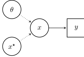
Figure 2.2.: Directed acyclic graph of the non centered parametrization.
