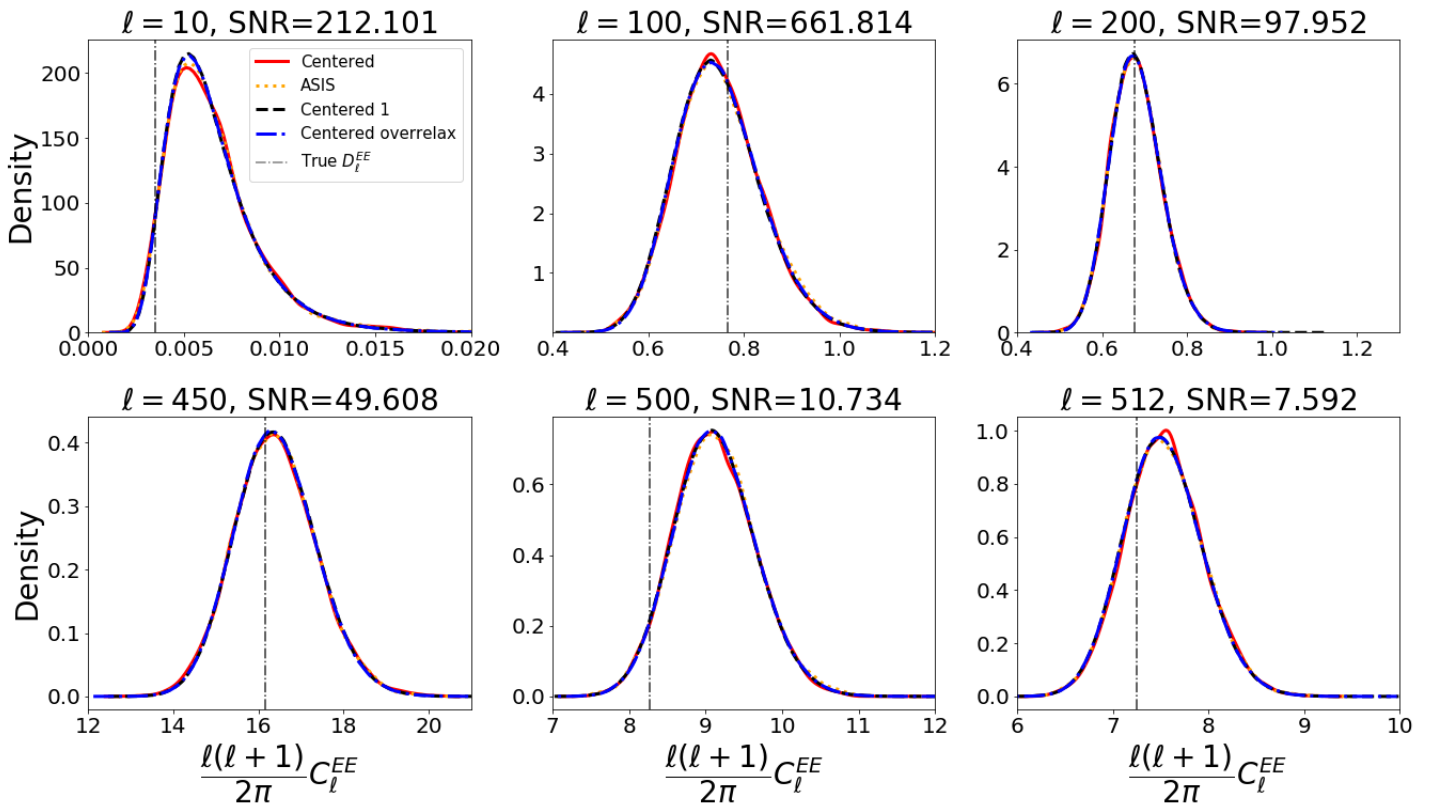
Figure C.9.: Kernel density estimation of marginals for a sample of multipoles for EE components for cut-sky experiment, Section 3.7.2.
