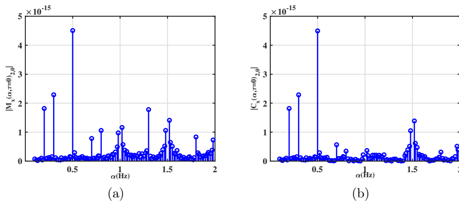
Figure 3.25: Second-order cyclic statistics of the reflected signal with small number of samples 601: (a) cyclic temporal moment; (b) cyclic temporal cumulant
