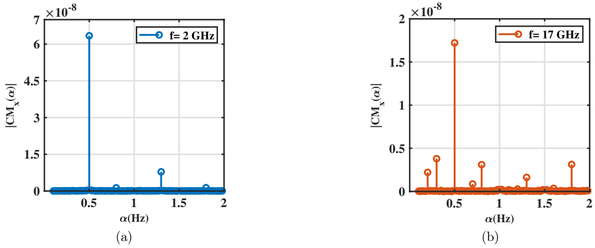
Figure 5.48: The cyclic mean |CM_x(\alpha)| of the reflected signal for the frequency system 2 GHz and 17 GHz
