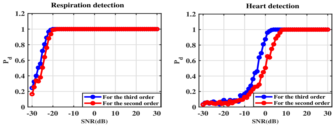
Figure 3.38: Probability of detection of respiration and heartbeat as a function of SNR
