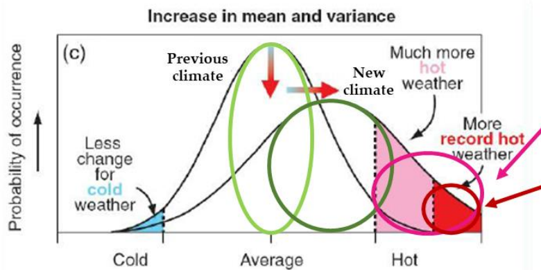
Figure 29 - Mitigation, adaptation and resilience to future climate changed induced temperatures, adapted from (Folland et al., 2001) and (Alessandrini et al., 2019)
