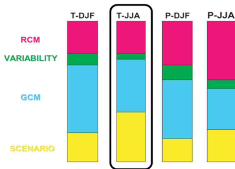
Figure 26 - Relative contribution to the uncertainty in the simulation of climate change over Europe originating from various sources: RCMs (8 models), internal variability of GCMs, GCMs (4 models), scenarios (2 used). T is the temperature and P is the precipitation. DJF is winter and JJA is summer. The highlighted column is the summer temperature (Giorgi, 2006)
