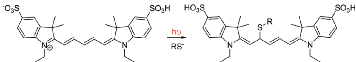
Figure 3.11: Mechanism of Cy5 fluorophore blinking in low oxygen environment in a STORM experiment. The thiol ( RS^- ) reacts with the bridge of Cy5 and breaks its conjugated electron system and creates the dark state of Cy5. Figure from [186]
