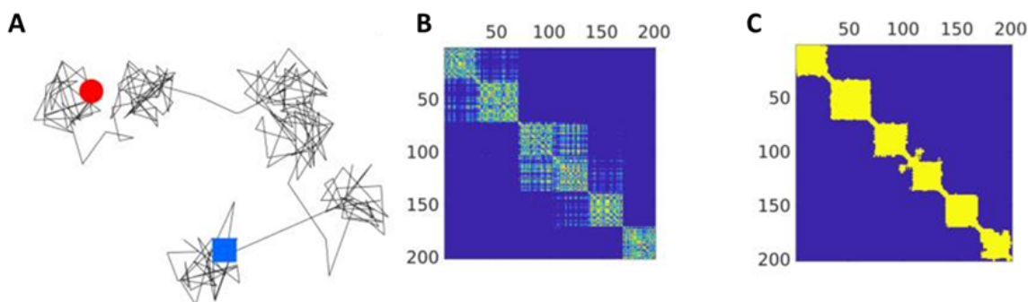
Figure 5.8: (A) Simulated 2D trajectory where the motion alternates between confined and free Brownian motion. (B) The distance matrix was created from the trajectory in (A). (C) The binary matrix was created by convolving the distance matrix with a normalized and constant square 5 \times 5 matrix and by then applying a threshold to the matrix values. Figure extracted from [253]
