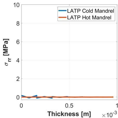
(c) Radial stress distribution.
