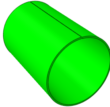
(b) Distortions of [\pm 90^\circ]_6 tube manufactured with a cold mandrel using a deformation scale factor of 1.3.
