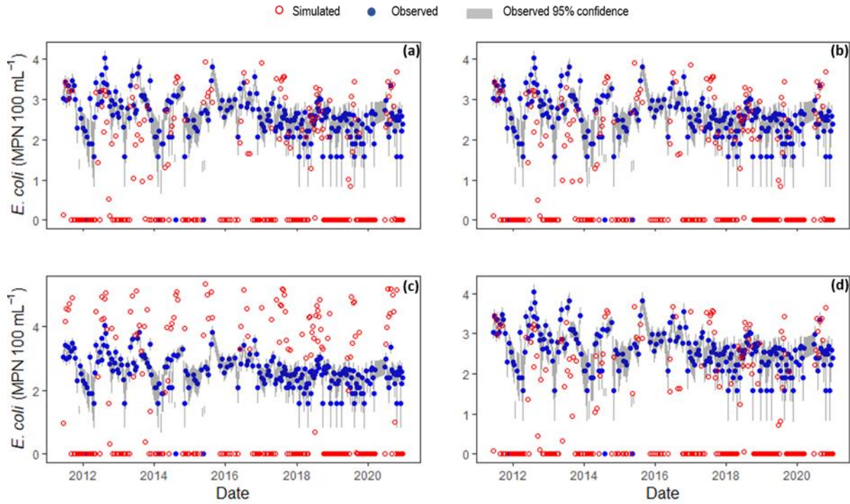
Figure 37: Observed and simulated [ E. coli ] (MPN 100 mL -1 ) at the NK20 station from May 2011 to December 2020: Log-transformed comparison with (a) the original SWAT bacteria module; (b) the resuspension release processes; (c) the resuspension release processes and regrowth; (d) the resuspension release processes and hyporheic exchange.
