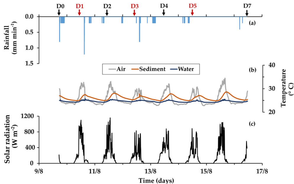
Figure 26: Temporal variations of environmental variables in the headwater wetland of the Houay Pano catchment, northern Lao PDR, 9–16 August 2019: (a) Rainfall (mm min -1 ); (b) Temperatures (° C) recorded in the swamp sediment, in the swamp water, and in the air; (c) solar radiation (W m -2 ). The vertical black arrows above the upper y axis represent the days of sampling to measure turbidity and [ E. coli ] and the red arrows represent the days of sampling to measure [DOC] and [TSS] in addition to turbidity and [ E. coli ].
