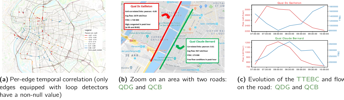
Figure 4.17: Per-edge temporal correlation between EBC and flow (a) and zoom on a specific region (b,c).
