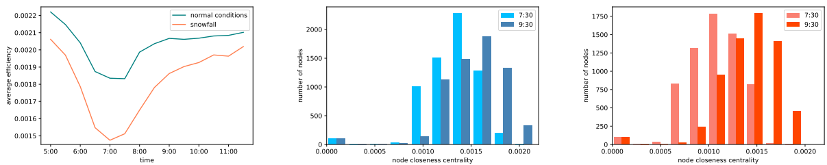
(a) AE under normal conditions and in pres- (b) NCC evolution under normal conditions (c) NCC evolution in presence of disruption ence of a snowfall
