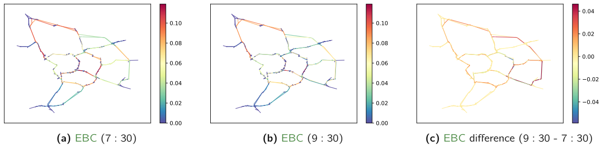
Figure 3.9: EBC spatial distribution at 7 : 30 am (a), at 9 : 30 am (b) and the difference between 9 : 30 am and 7 : 30 am (c) for the peri-urban transport network.
