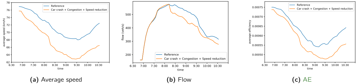
Figure 3.18: Global evolution of the average speed (a), the flow of vehicles (b), and the AE under normal conditions and in presence of the three previously described disruptions at the same time.
