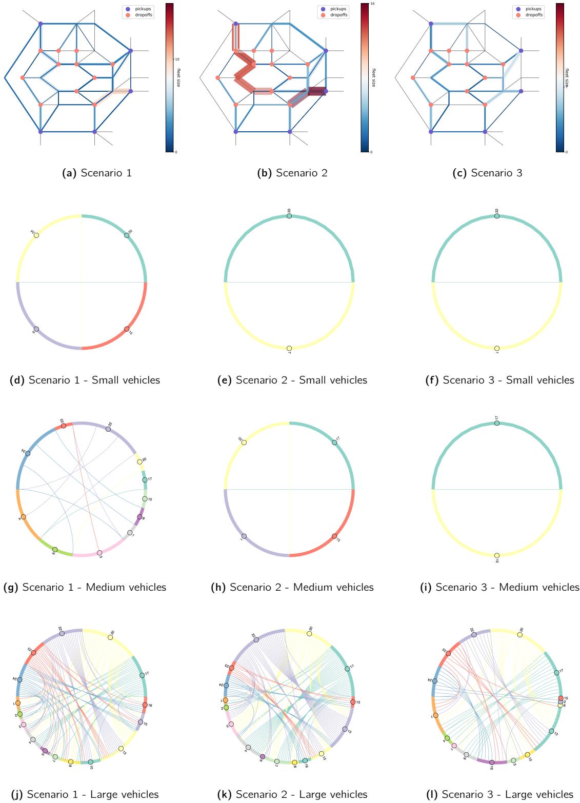
Figure 5.16: Fleet size and its distribution ( z_{ijk}^w ) between optimal pick-ups (purple nodes/labels) and drop-offs (light-red nodes/labels) for the 3 stochastic scenarios.
