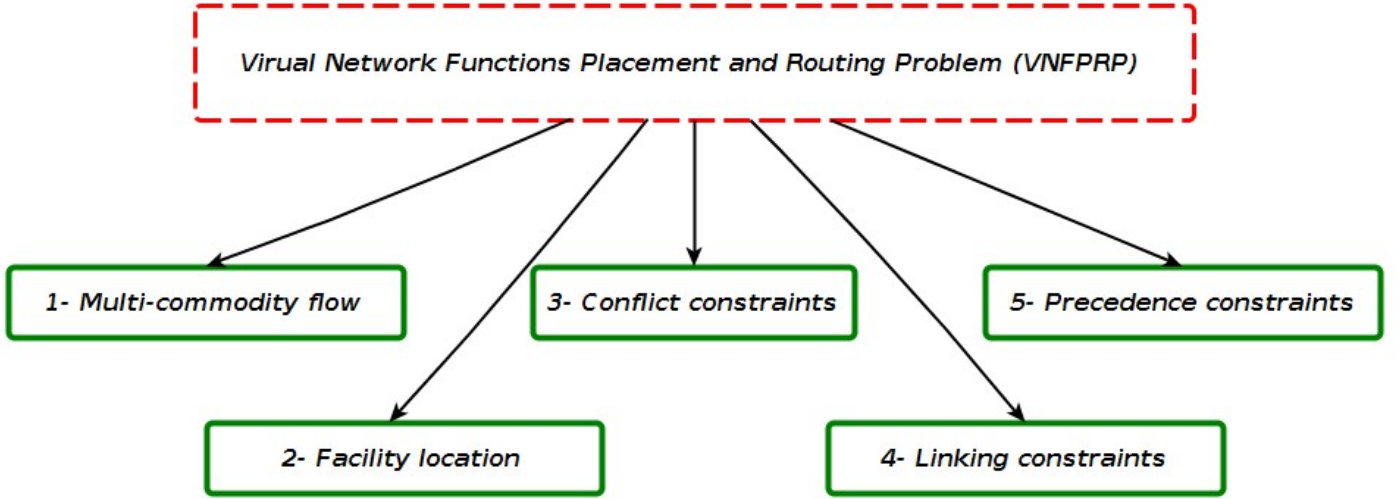
Figure 2.1: VNFPRP is composed of multiple subproblems and constraints.
