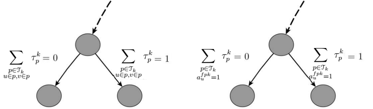
Figure 4.3: Branching scheme for Dantzig-Wolfe formulation.
