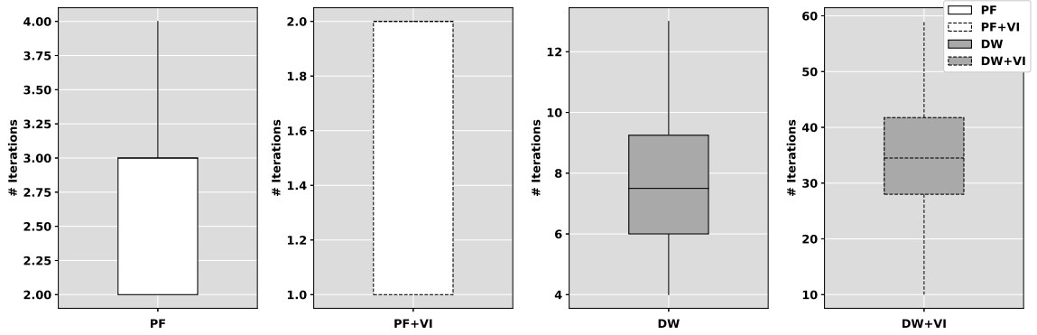
Figure 4.15: Number of generated iterations by PF and DW formulation with and without valid inequalities.
