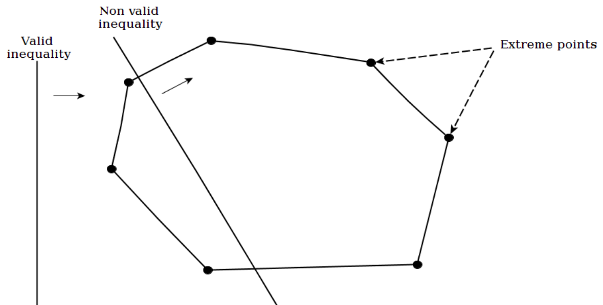
Figure 1.2: Example of valid and non valid inequalities and extreme points
