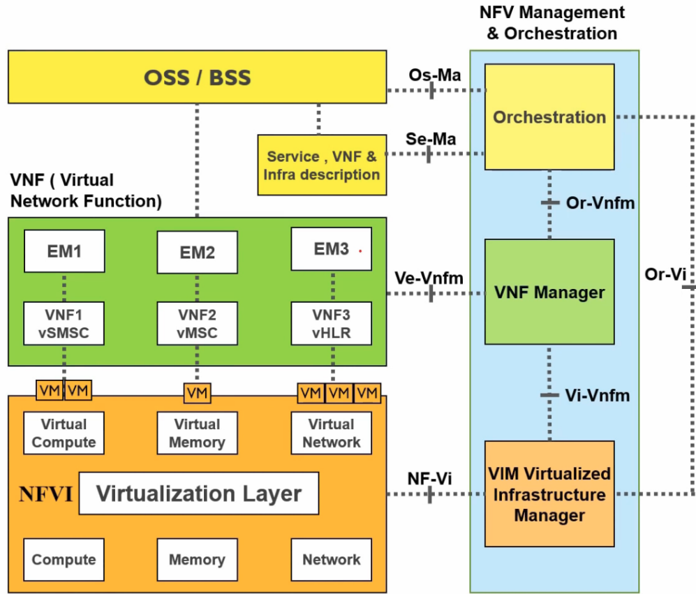
Figure 1.8: NFV Architecture [4]
