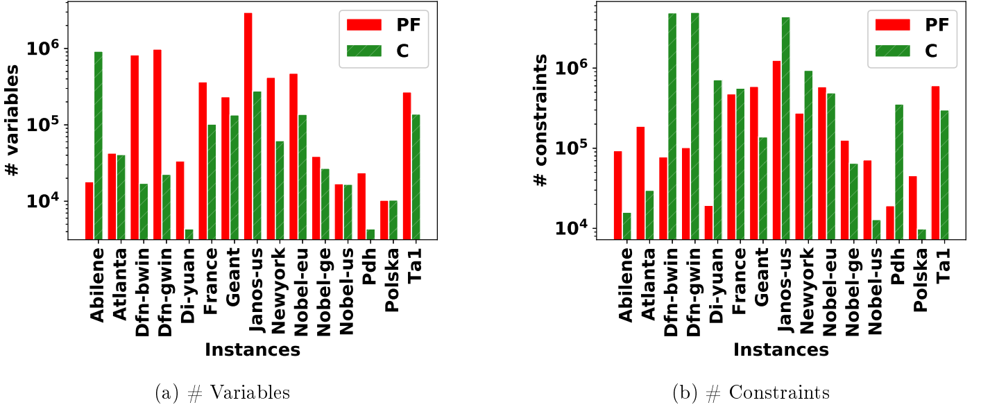
Figure 3.1: Comparison between the path-based MILP formulation and the compact MILP formulation with respect to the number of variables and constraints.
