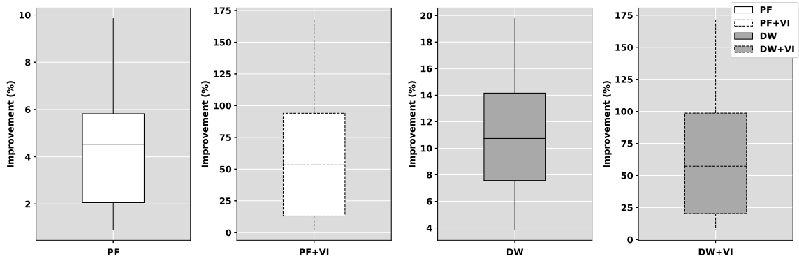
Figure 4.12: Relative improvement of LP-relaxation bounds of \mathcal{C} formulation by using PF and DW formulation with and without valid inequalities.
