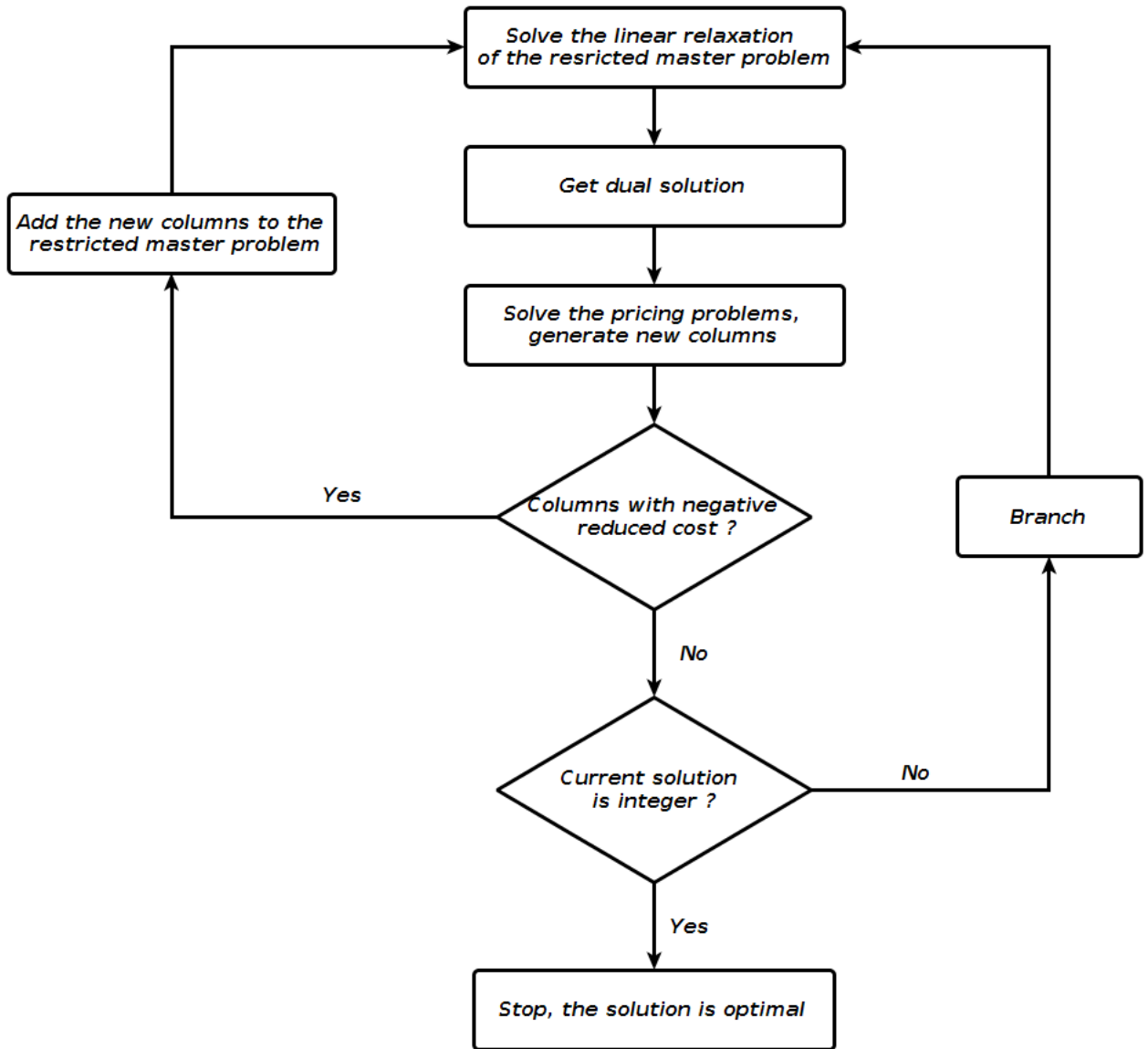
Figure 4.4: Branch-and-Price algorithm.
