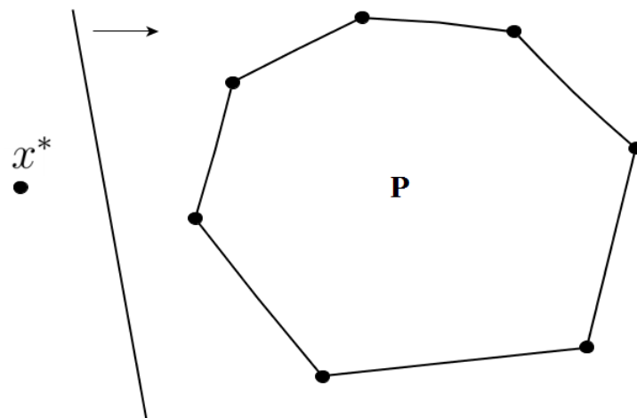
Figure 1.3: A hyper-plane separating x^* and P
