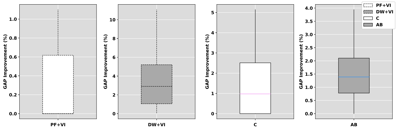
Figure 4.17: Gap improvement comparison between the path formulation, Dantzig-Wolfe formulation, the compact formulation and the Automatic Benders of Cplex.
