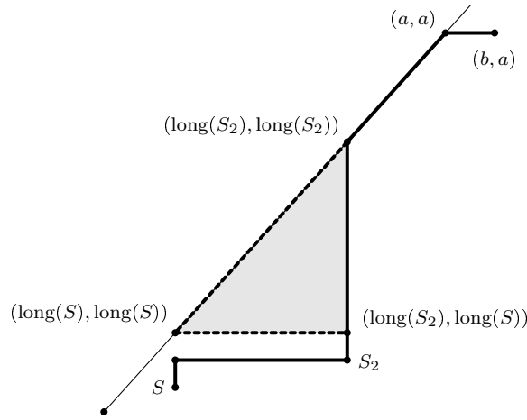
Figure 10.4 – The easiest path via which the rectangle S can grow first to S_2 , and then to R , in Case 2 of Claim 5. In the proof, the lower two thick segments are replaced with the lower dashed one, and Lemma 10.2.10 is applied to the shaded triangle.
