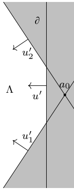
Figure 7.2 – The open domain \partial defined in (7.1) is shaded, while its complement \Lambda is not. The lines are the boundaries of the three half-planes defining \partial . Note that if a_0 \notin \mathbb{H}_{u'} , then \Lambda becomes simply a cone.
