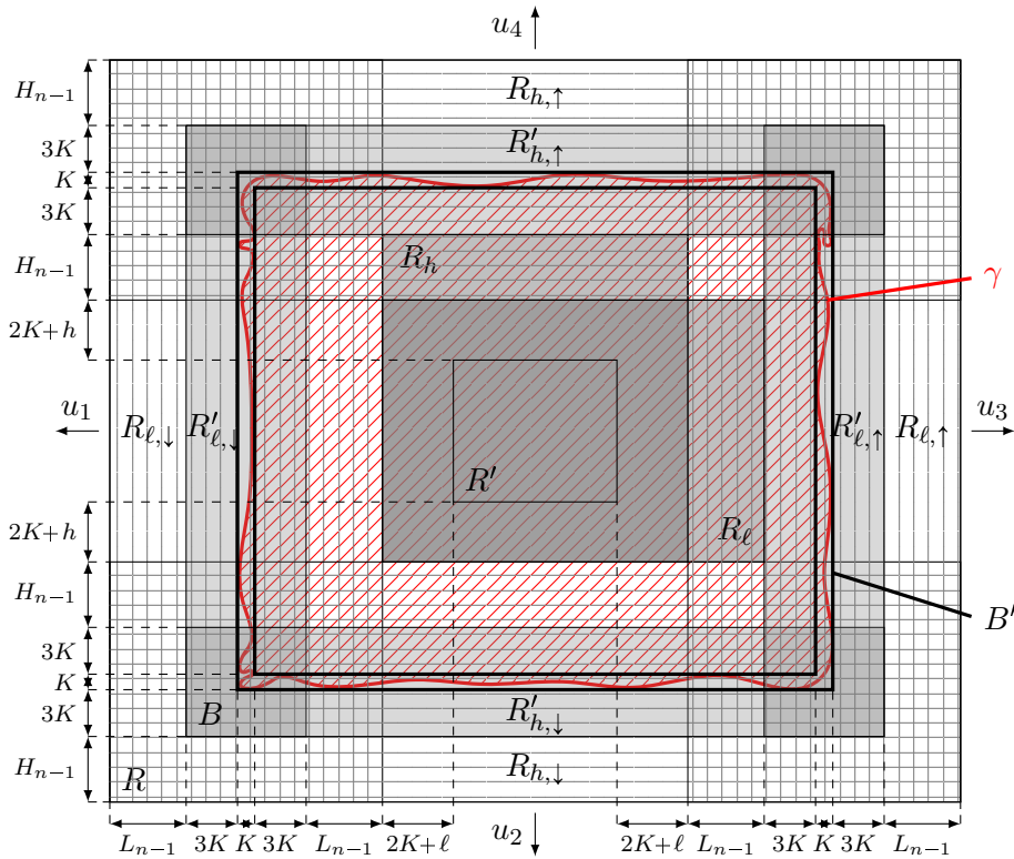
Figure 8.1 – The setting of the proof of Lemma 8.1.11. For the figure we assume that u_3 = 0 and u_4 = \pi/2 . B' is the frame with thickened boundary, R_\ell and R_h are the overlapping regions in dark gray. The regions R'_{\ell,\downarrow} , R'_{h,\downarrow} , R'_{\ell,\uparrow} and R'_{h,\uparrow} are in lighter gray and the frame formed by their union is B . The horizontally (resp. vertically) hatched regions are R_{h,\downarrow} and R_{h,\uparrow} (resp. R_{\ell,\downarrow} and R_{\ell,\uparrow} ). The contour inside B' is \gamma and its diagonally hatched interior is \tilde{\gamma} . All the regions drawn are closed subsets of \mathbb{R}^2 with the exception of R_\ell , R_h and \tilde{\gamma} , which are open. The thicker version, \bar{\gamma} , of \gamma and the set F \subset \mathbb{Z}^2 defined in (8.1) are not drawn.
