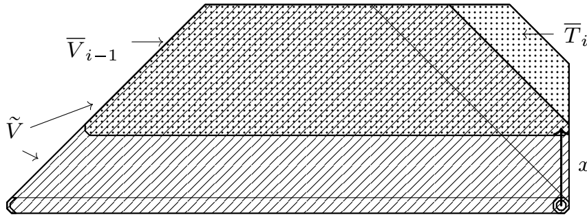
Figure 4.9 – The geometric setting of Lemma 4.3.14. The snail \tilde{V} is hatched, \bar{V} is dotted and their union is the original snail \hat{V} . The dotted-hatched region is \bar{V}_{i-1} , while the dotted trapezoid is \bar{T}_i .
