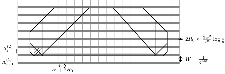
Figure 4.10 – The partition of \Lambda into strips \Lambda_i = \Lambda_i^{(1)} \cup \Lambda_i^{(2)} , i \in [M] . The hatched region represents a square Q_{i,j} , which we would like to resample. The thick polygon is the snail V with its trapezoids. Note that its base B does not intersect Q_{i,j} and (almost) spans the squares Q_{i,j+1}, \dots, Q_{i,j+\lambda} .
