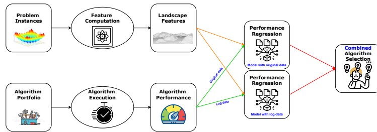
Figure 2.1: High-level schematic representation of the structure of our novel combined landscape-aware algorithm selection pipeline.
