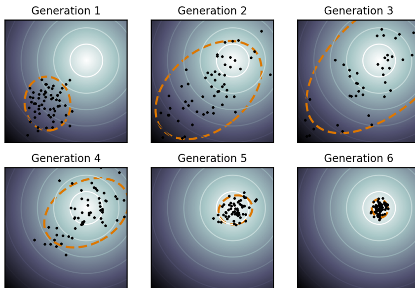
Figure 3.1: Illustration of the CMA-ES algorithm. Taken from Wikimedia Commons [Com08].
