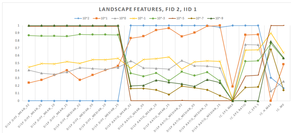
Figure 9.1: Normalized feature values for the Dispersion and Information Content feature sets for the first instance of the BBOB function F2 (ellipsoid function).
