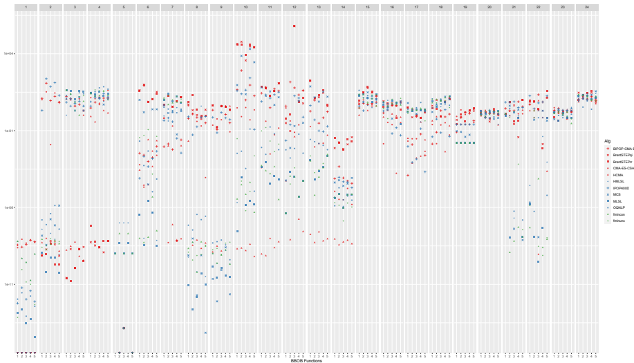
Figure 7.1: Single-run performances (measured by the target precision) of the 12 algorithms on the first five instances of 24 BBOB functions. They represent our portfolio from which we want to select the best-performing algorithm for an unseen problem instance.
