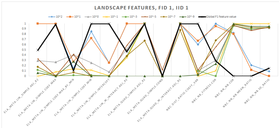
Figure 9.2: Normalized feature values for the Meta-model and Nearest-Better Clustering feature sets for the first instance of the BBOB function F1 (sphere function).
