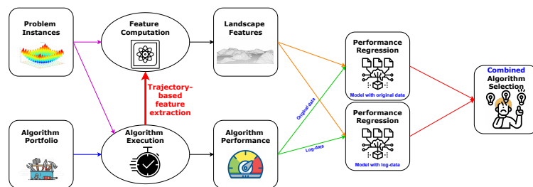
Figure 2.2: High-level schematic representation of the structure of our novel trajectory-based landscape-aware algorithm selection pipeline.
