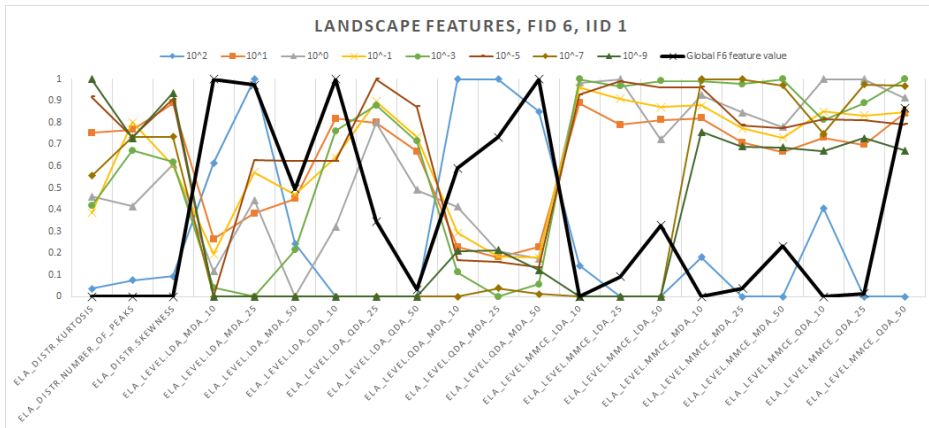
Figure 9.3: Normalized feature values for the y-Distribution and Levelset feature sets for the first instance of the BBOB function F6 (attractive sector function).
