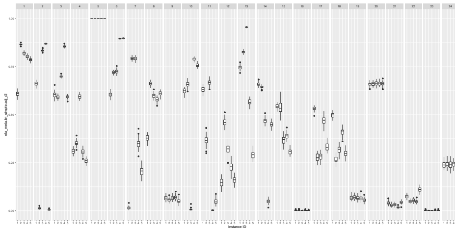
Figure 6.3: Distribution of approximated values for the ela_meta_lin_simple_adj_r2 feature for the first five instances of the 24 BBOB functions, normalized in the 0-1 range. The values are computed from 2000 samples each, and each box plot shows the distribution of 50 independent runs.
