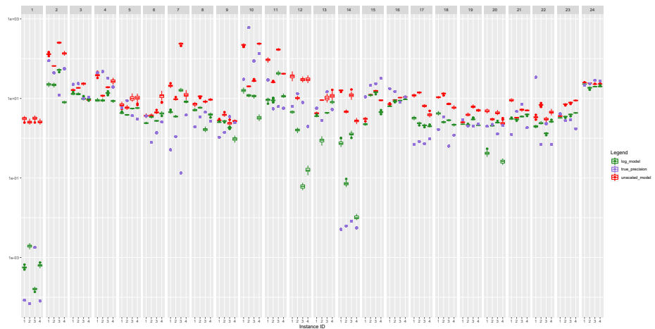
Figure 6.4: Distribution of predicted algorithm performance values by the unscaled (in red) and logarithmic regression models (in green) across 50 independent runs, with the actual algorithm performance values (in purple) as dots. The algorithm performance is measured by the target precision.
