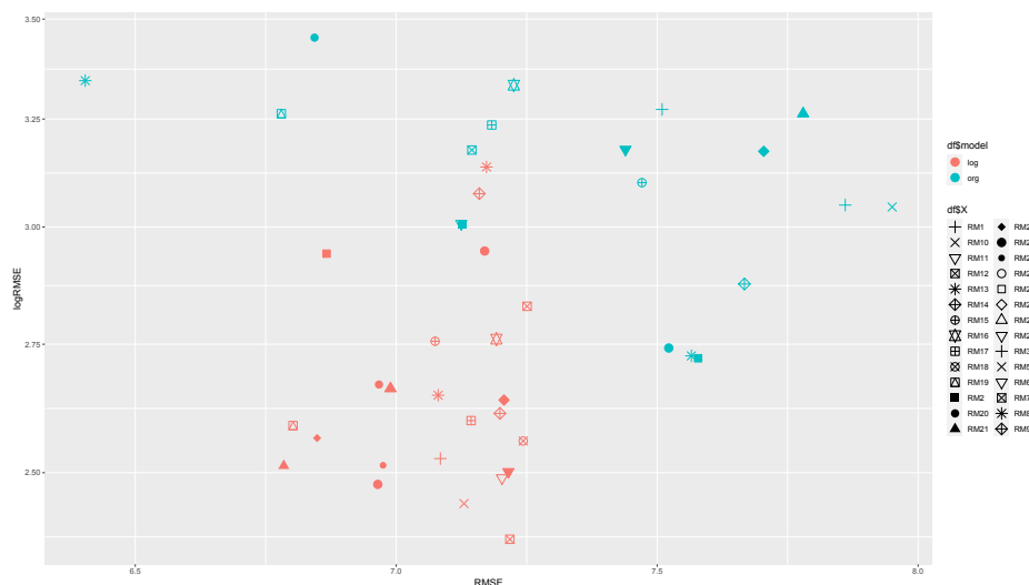
Figure 7.2: Overall prediction quality of different regression models (RMSE vs. log-RMSE), from both the unscaled (in blue) and the log-based approach (in red) on the CMA-ES-CSA algorithm, with the budget of 1000 function evaluations and 2000-sample feature size. Minimizing both error values as a Pareto front, we see that log-based regression models perform significantly better than the unscaled ones.
