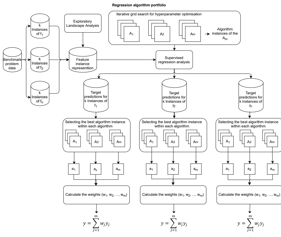
Figure 8.2: Training phase of the personalized problem ensembles.
