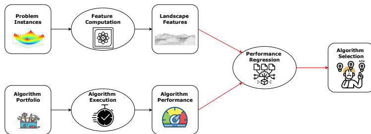
Figure 1.2: High-level schematic representation of the structure of landscape-aware algorithm selection pipeline, where the algorithm selection is based on predicted performance values .
