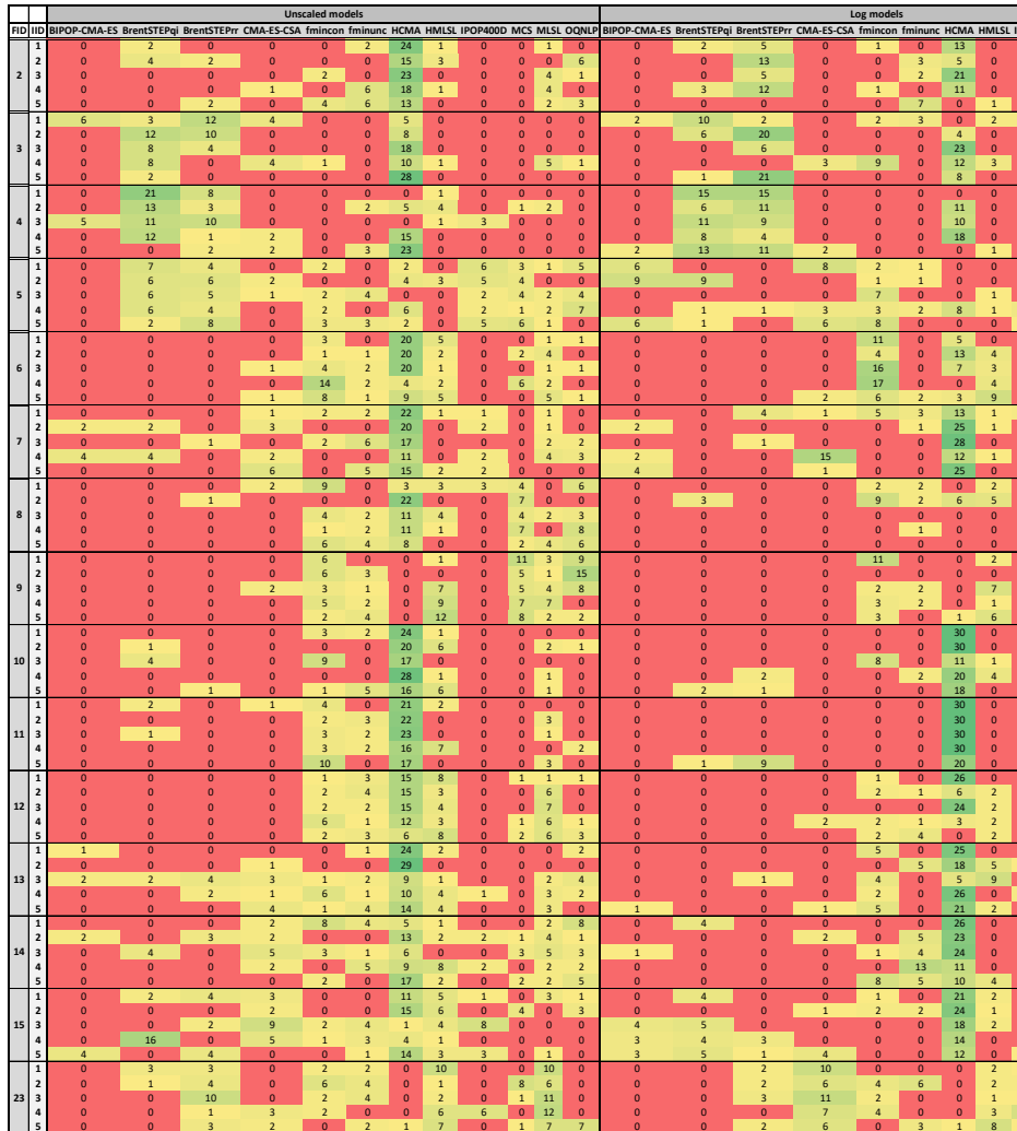
Figure 7.3: Heatmap of the selection frequency of each algorithm from the portfolio per problem instance, both for the unscaled (left) and log-based approach (right), for the budget of 1000 function evaluations and the feature size of 250 samples, showing selected functions only for reasons of space.
