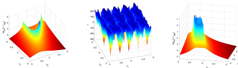
Figure 3.2: Examples of BBOB noiseless test bed function landscapes. Left: F9, the rotated Rosenbrock function (unimodal, low or moderate conditioning). Middle: F16, the Weierstrass function (multimodal, adequate global structure). Right: F20, the Schwefel function (multimodal, weak global structure). Taken from [HAF+10].
