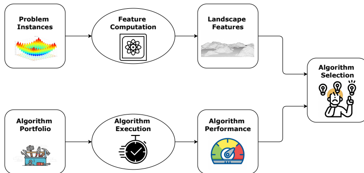
Figure 1.1: High-level schematic representation of the structure of landscape-aware algorithm selection pipeline.
