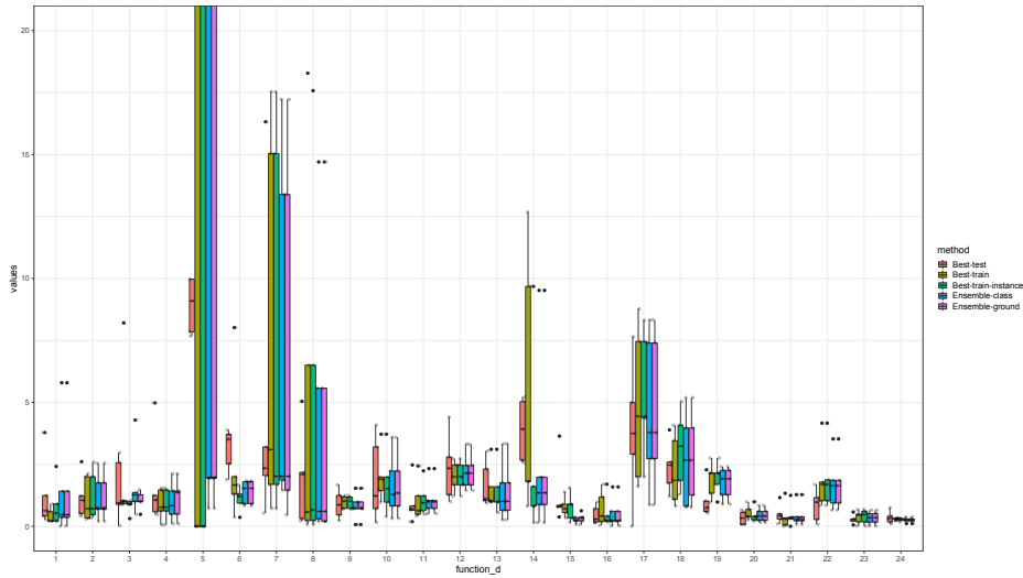
Figure 8.3: Evaluation results of the BIPOP-CMA-ES performance prediction. The y -axis corresponds to the absolute error between the ground truth and predicted target precision (i.e., the logarithm of the target precision), while the x -axis corresponds to each BBOB benchmark problem. The box plots represent the distribution of the absolute error obtained from each test fold for each problem separately in five different scenarios: a) Best-test, b) Best-train, c) Best-train-instance, d) Ensemble-class, and e) Ensemble-ground.
