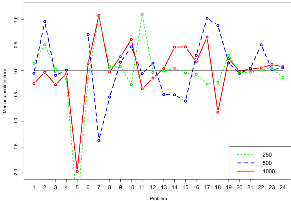
Figure 8.5: Relative advantage of the Ensemble-class model vs. the Best-train model for each of the 3 budgets (250, 500, 1000 function evaluations). The y -axis represents the difference between the median absolute errors. Positive values indicate where the Ensemble-class model outperforms the Best-train model.
