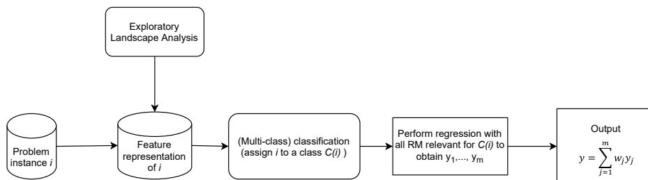
Figure 8.1: Application of the personalized machine learning models. Note that the abbreviation RM stands for regression models.
