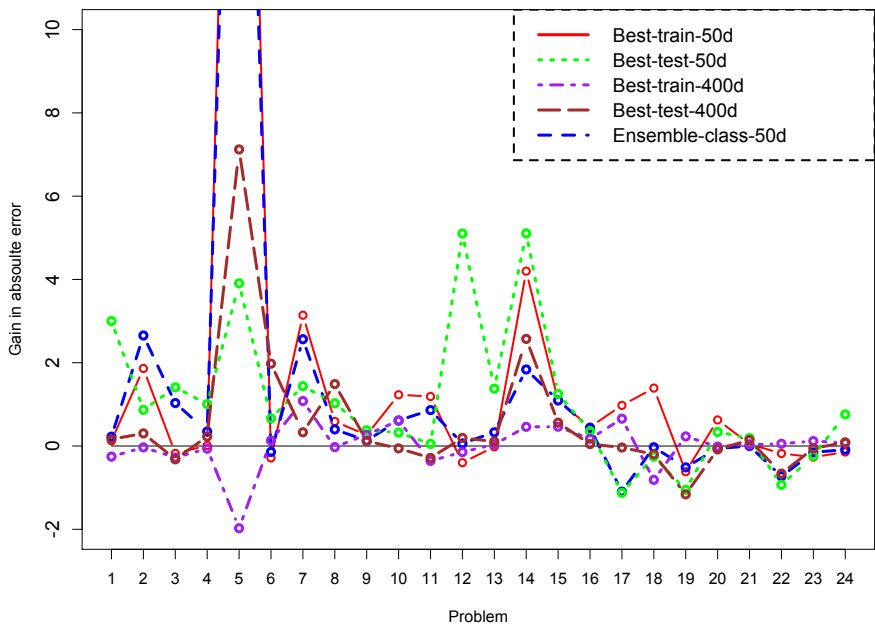
Figure 8.4: Relative advantage of the Ensemble-class-400d model vs. simple regression models (Best-train-50d, Best-test-50d, Best-train-400d, Best-test-400d, Ensemble-class-50d). The y -axis represents the difference between the median absolute errors. Positive values indicate where the Ensemble-class-400d model performs better than the other models, while negative values indicate the opposite.
