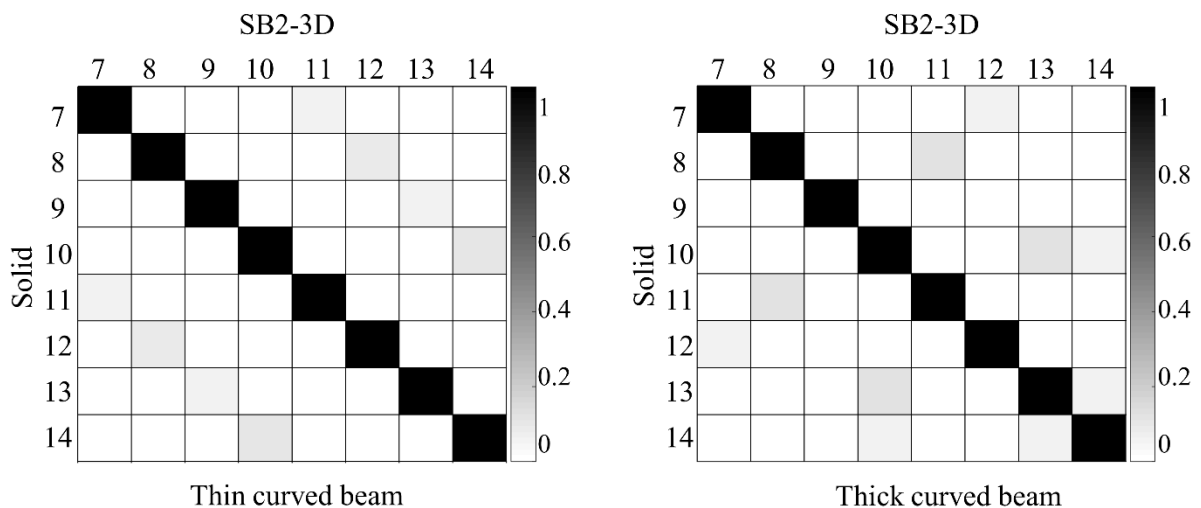
Fig. 3.29. Curved beam in free-free vibration – MAC matrix between the SB2-3D solid-beam and the reference models for the thin and thick beams.
