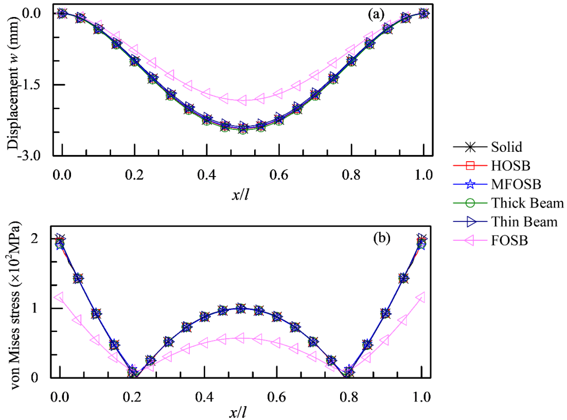
Fig. 3.10. Straight beam with square cross-section under distributed loading – Distribution of vertical displacement along the mid-axis (a) and von Mises stress along a line on the lower surface (b), in the thin case.
