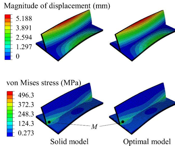
Fig. 4.19. “T” shape plates – Displacement and von Mises stress distributions for the optimal model and reference solid model.
