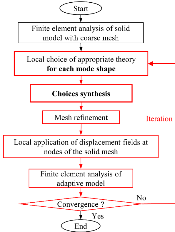
Fig. 4.6. Flowchart of adaptive modeling process for vibration analysis.
