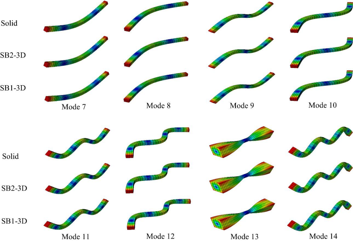
Fig. 3.22. Straight beam in free-free vibration – First eight mode shapes for the reference solid, SB2-3D, and SB1-3D models in the thin case.
