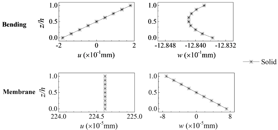
Fig. 3.1. Thin beam under bending or membrane loading – Distribution of through-the-thickness displacements.
