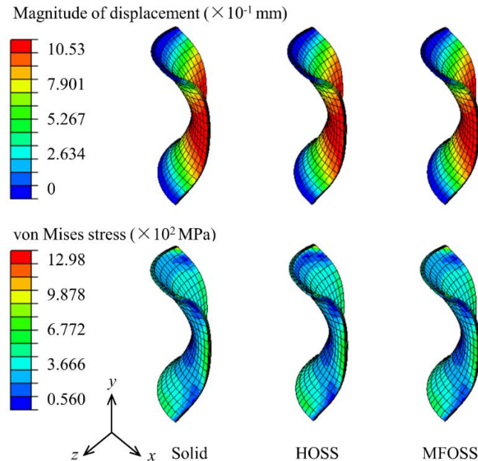
Fig. 2.18. Quarter of hyperboloid under pressure - Displacement and von Mises stress distributions in the thin shell case.
