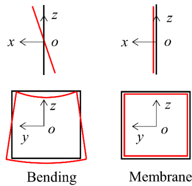
Fig. 3.2. Beam under bending or membrane loading – Deformation of a cross-section.
