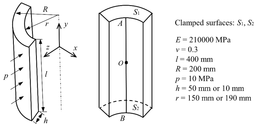
Fig. 2.12. Quarter of cylinder under pressure – Presentation of the example.
