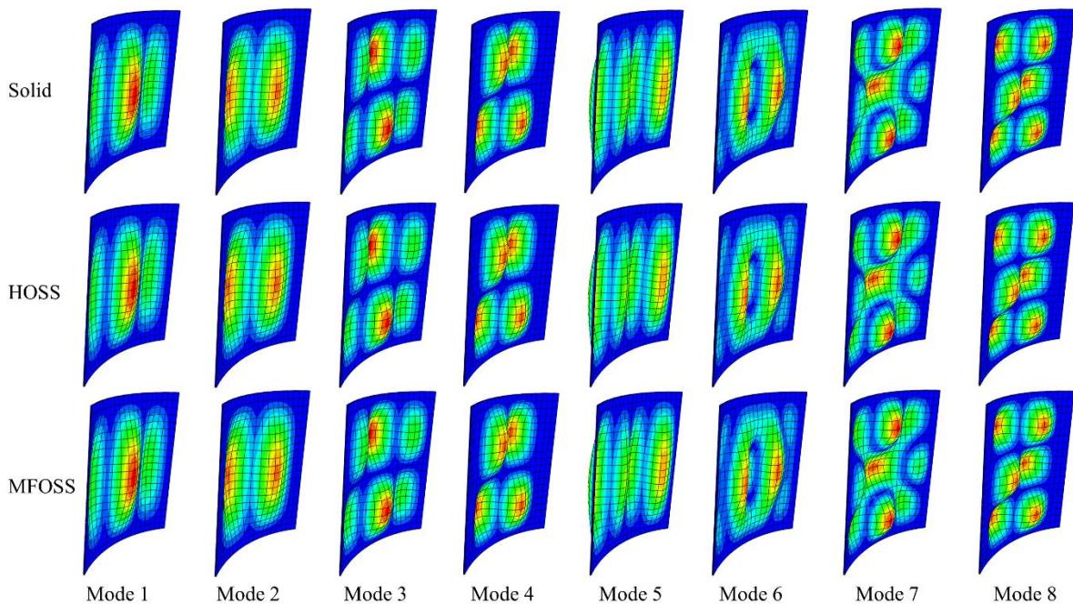
Fig. 2.28. Clamped cylindrical panel in free vibration – First eight mode shapes with the reference solid, HOSS, and MFOSS models for the thin case.
