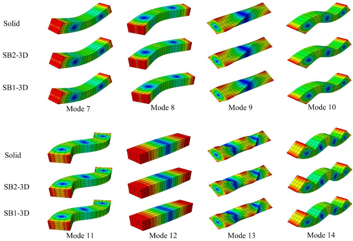
Fig. 3.23. Straight beam in free-free vibration – First eight mode shapes for the reference solid, SB2-3D, and SB1-3D models in the thick case.
