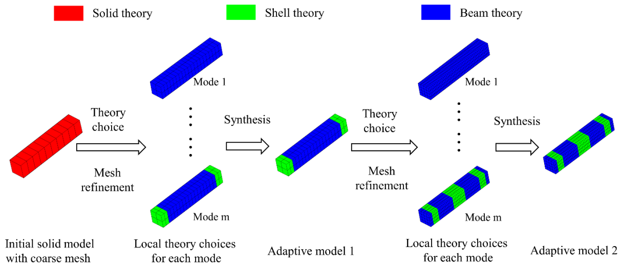
Fig. 4.7. Example of a synthesis concerning the local choice of theory for vibration analysis during the iterative process.
