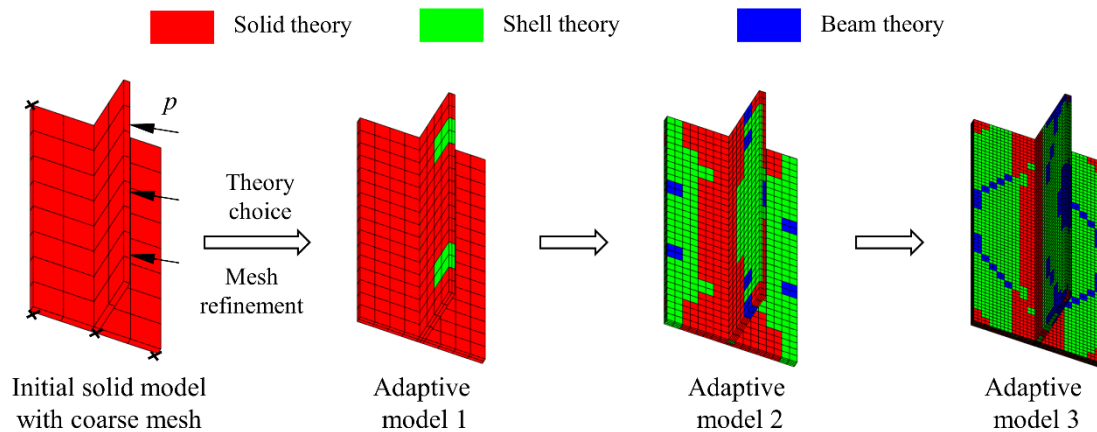
Fig. 4.21. “T” shape plates – Evolution of the choice of theory during the iterative process with the element C3D8I.
