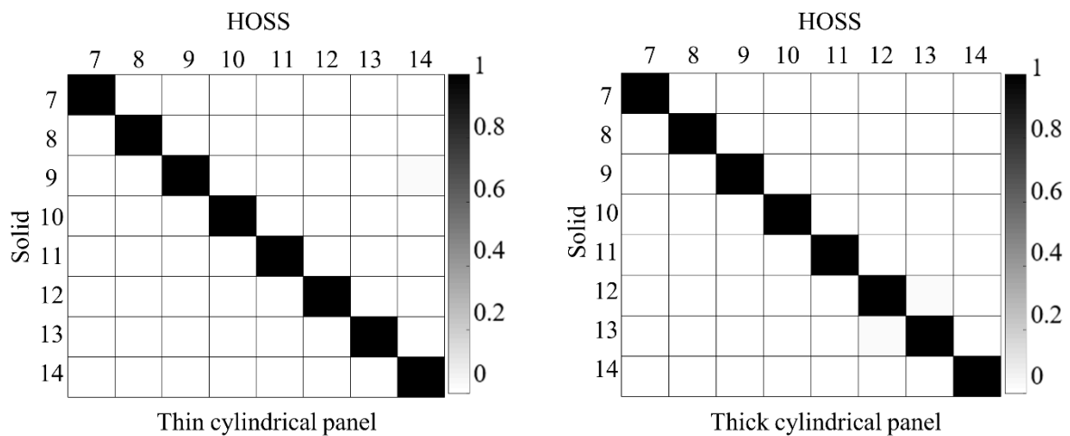
Fig. 2.30. Clamped cylindrical panel in free vibration – MAC matrix between the solid-shell and the reference models for the thin and thick panels.
