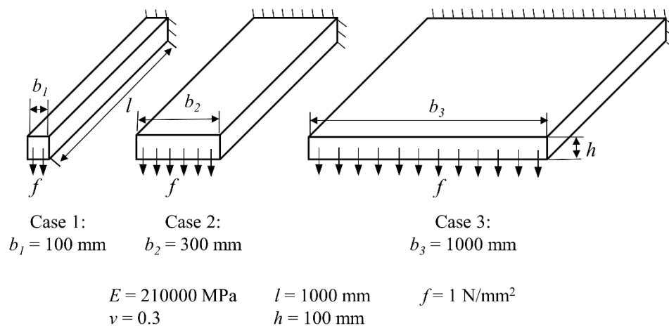
Fig. 4.8. Cantilever structures – Presentation of the example for three width/thickness ratios.
