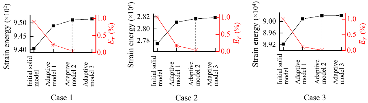
Fig. 4.10. Cantilever structures – Convergence of the methodology in the three cases.
