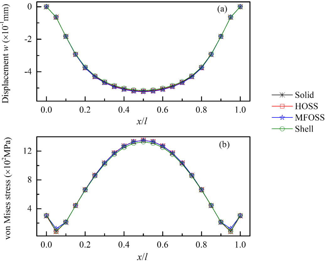
Fig. 2.14. Quarter of cylinder under pressure – Distribution of vertical displacement (a) and von Mises stress (b) along a line on the lower face, in the thin case.
