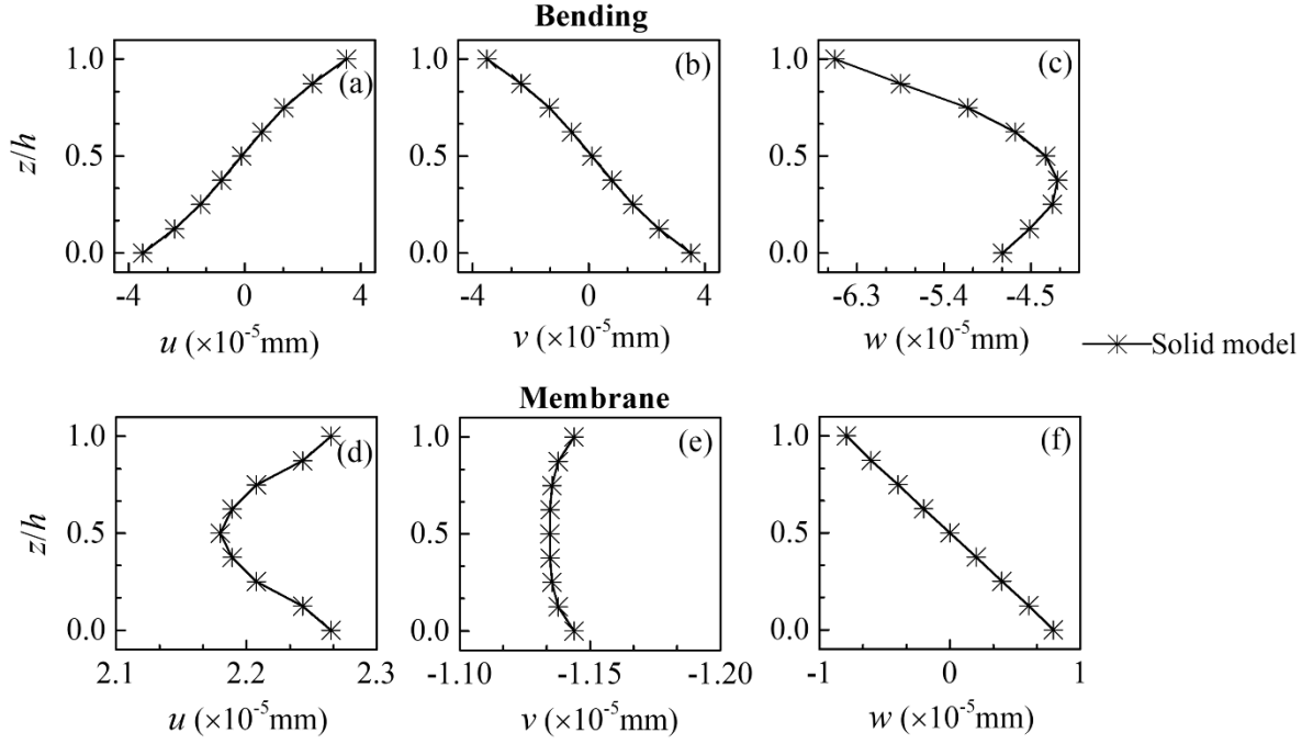
Fig. 2.2. Thick square plate under membrane or bending loading – Distribution of through-the-thickness displacements.
