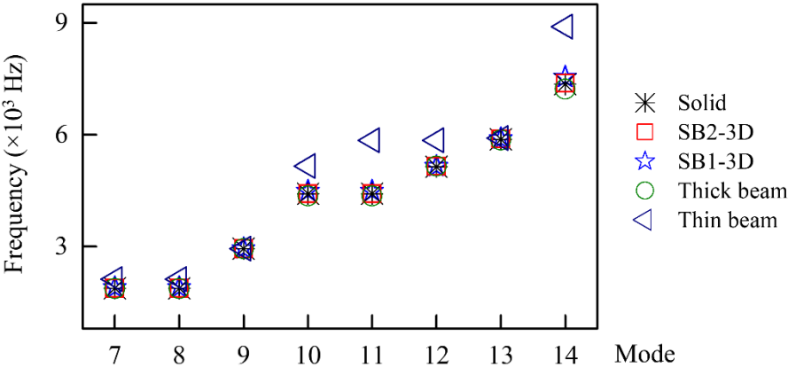
Fig. 3.26. Straight beam in free-free vibration – Natural frequencies for the reference solid model, SB2-3D model, SB1-3D model, thin and thick beam models in the thick case.
