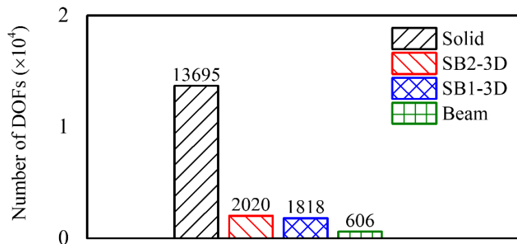
Fig. 3.32. Comparison of the number of degrees of freedom between solid, SB2-3D, SB1-3D and beam models.
