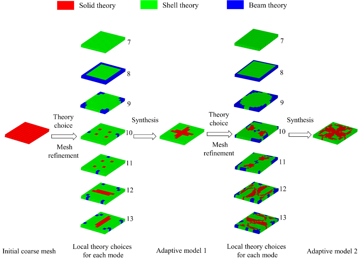
Fig. 4.30. Moderately thick structures – Theory choice for the first seven modes in case 3.
