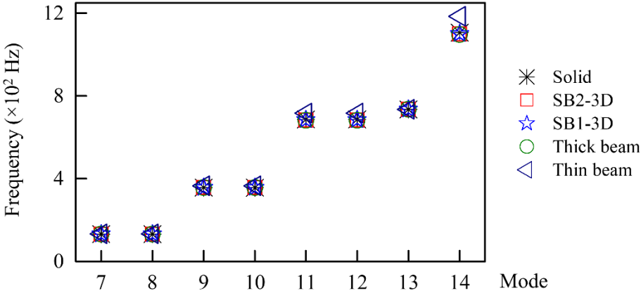
Fig. 3.25. Straight beam in free-free vibration – Natural frequencies for the reference solid model, SB2-3D model, SB1-3D model, thin and thick beam models in the thin case.
