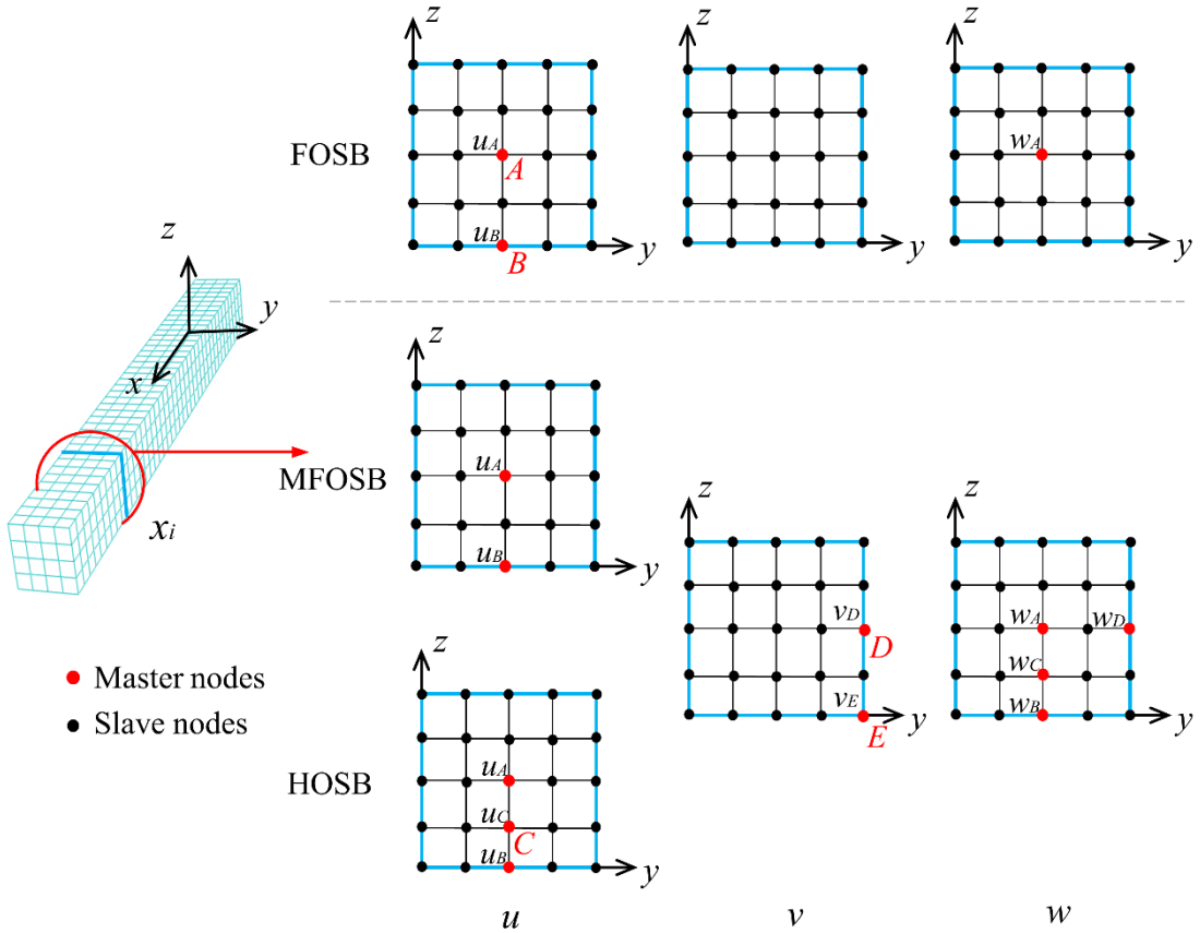
Fig. 3.6. Master nodes and slave nodes in the cross-section of a solid-beam model in a plane.
