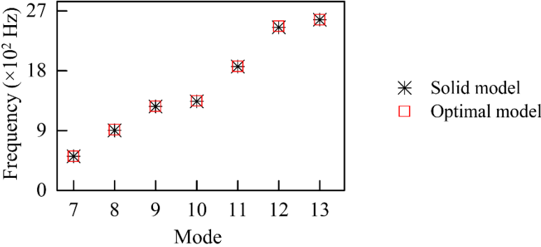
Fig. 4.28. Moderately thick structures – First seven natural frequencies for the optimal model and reference solid model in case 2.
