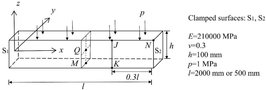
Fig. 3.8. Straight beam with square cross-section under distributed loading – Presentation of the example.
