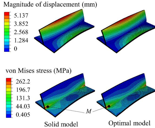
Fig. 4.22. “T” shape plates – Displacement and Von Mises stress distributions for the optimal model and reference solid model with the element C3D8I.
