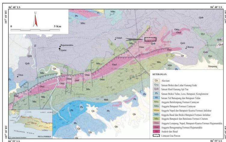
Fig. 2. B.11. Geological map of Rajamandala ridge and pawon cave (Maryanto 2009; Sudjatmiko 2003).
