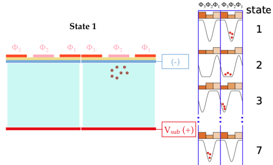
(f) Charge Movement → “Clocking”
