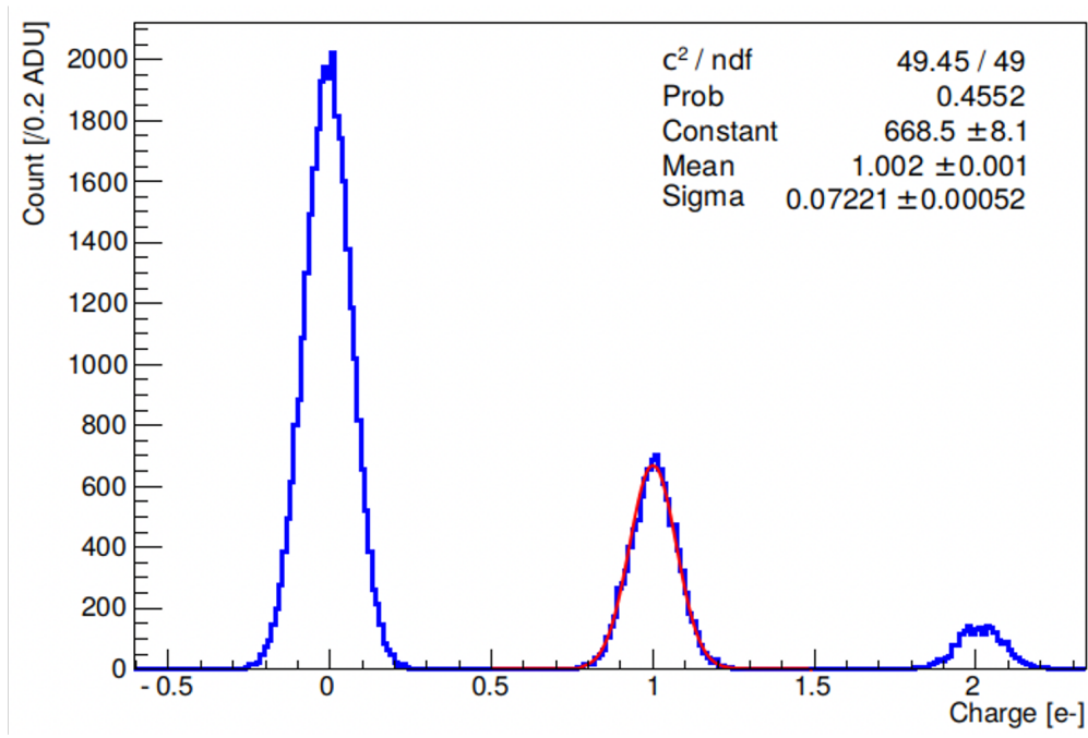
Figure 6.12: Best resolution ( \sigma_{\text{pix}} \sim 0.07 e^- at 1000 skips) yet achieved in a DAMIC-M prototype CCD.
