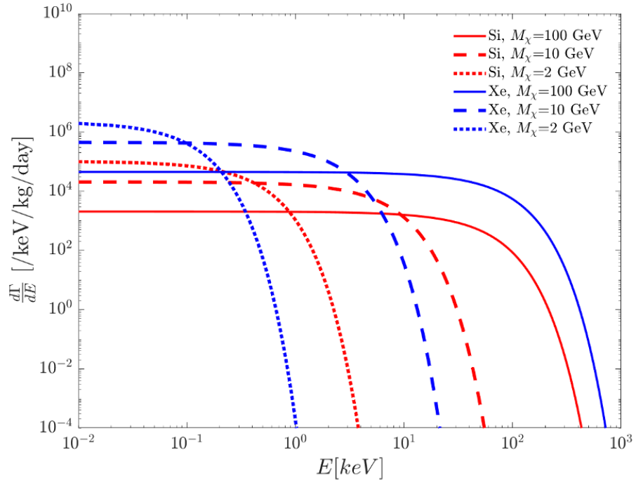
Figure 1.4: Top: WIMP velocity distribution (top) [14]. Bottom: calculated recoil spectrum for Si, Xe [51].
