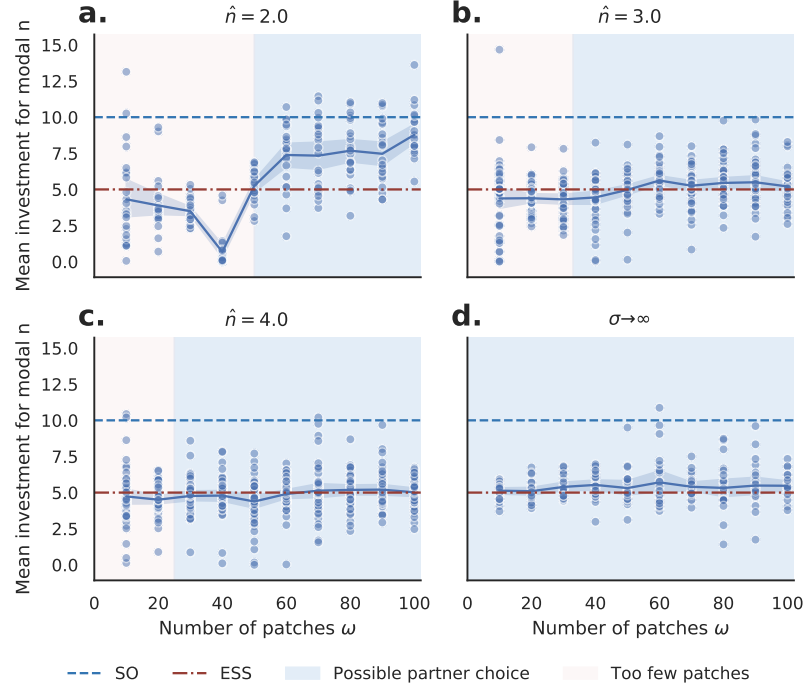
Figure 2.1: Mean investment in simulation for different numbers of opportunities \omega and a fixed population of N = 100 individuals. Results after 1500 generations. a. When \hat{n} = 2, \sigma = 1 Cooperation evolves when \omega \geq 50 . b-c. For \hat{n} \geq 3, \sigma = 1 , cooperative behaviours never evolve. d. When \sigma \rightarrow \infty , there is no pressure for individuals to attract partners and cooperative behaviours never evolve.
