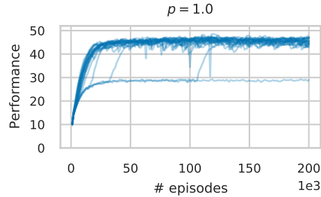
Figure 4.1: Performance of the best policy throughout learning with PPO, for each of the 24 independent runs. There are 23/24 runs that produced a policy where performance > 40 . The optimal value for a policy can be 50.
