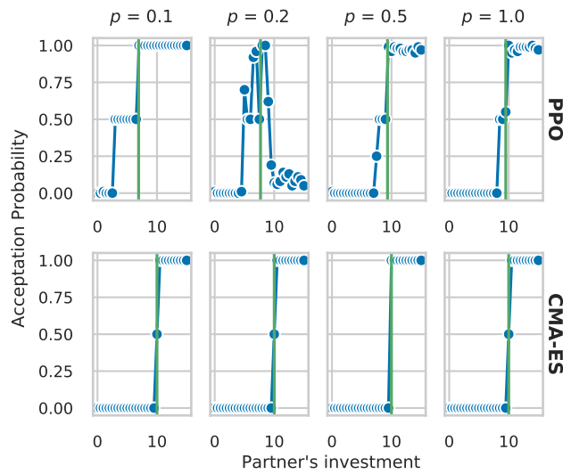
Figure 4.9: Analysis of the Partner Choice module for all conditions (by columns: p \in \{0.1, 0.2, 0.5, 1.0\} ) and all algorithms (top-line: PPO, bottom-line: CMA-ES). in the condition p = 1.0 for PPO. For each setup, only the best policy is shown. Each graph plots the probability to accept cooperation for the focal agent following the best policy (y-axis) depending on its partner's proposed investment (x-axis). Data are computed by presenting each of the 31 possible cooperative partners to the focal agent for 100 iterations as policies are stochastic. The green vertical line represent the mean investment of the focal agent.
