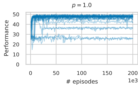
Figure 4.2: Performance of the best policy throughout learning with CMA-ES, for each of the 24 independent runs. There are 20/24 runs that produced a policy where performance > 40 . The optimal value for a policy can be 50.
