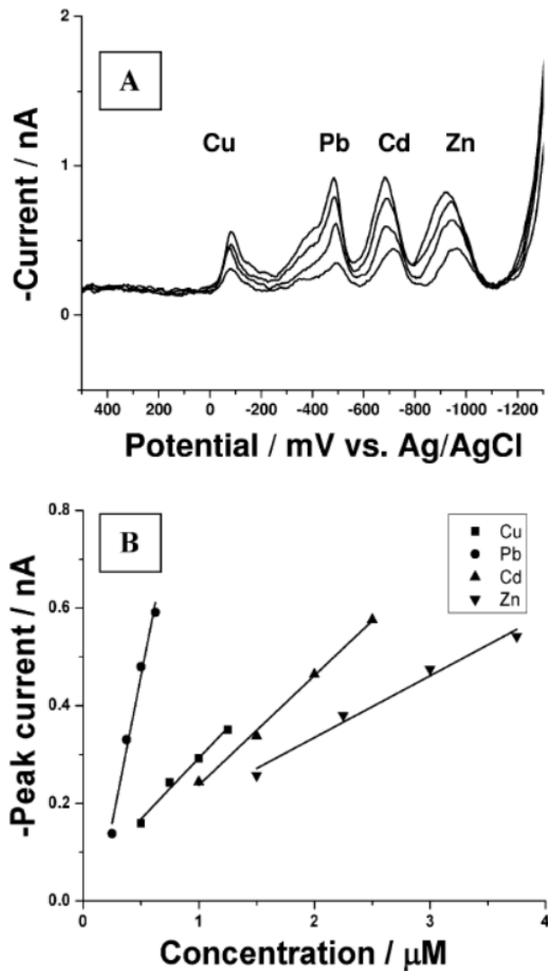
Figure 13. (A) Simultaneous detection of Cu 2+ , Pb 2+ , Cd 2+ and Zn 2+ , ion concentrations 0.5, 0.25, 1.0, 1.5 μM for Cu 2+ , Pb 2+ , Cd 2+ , Zn 2+ , respectively; and 1.5, 2, 2.5 times of above concentrations for these metals ions. (B) Calibration Curve for Cu 2+ , Pb 2+ , Cd 2+ , Zn 2+ . Accumulation time: 120 s, deposit potential: -1.5 V. Reproduced from [150].
