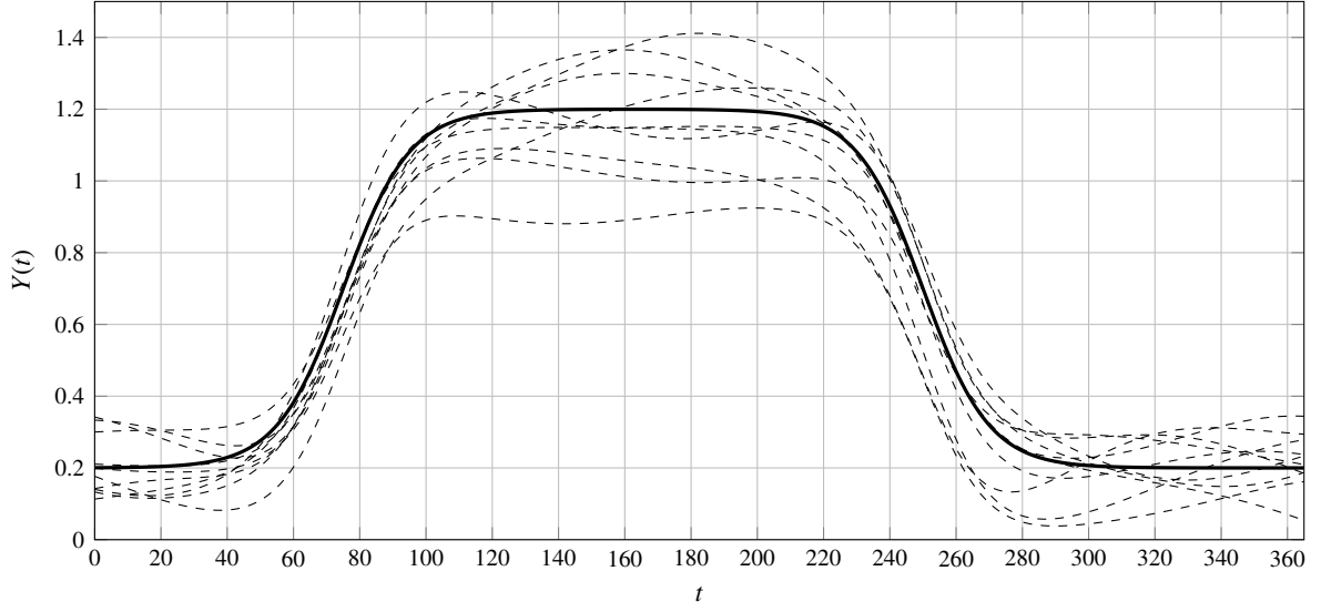
Figure 4.2: Simulated univariate Gaussian processes with squared exponential covariance function (length scale parameter set to 50). The continuous black line is the mean function and the dashed lines are the corresponding 10 realizations.
