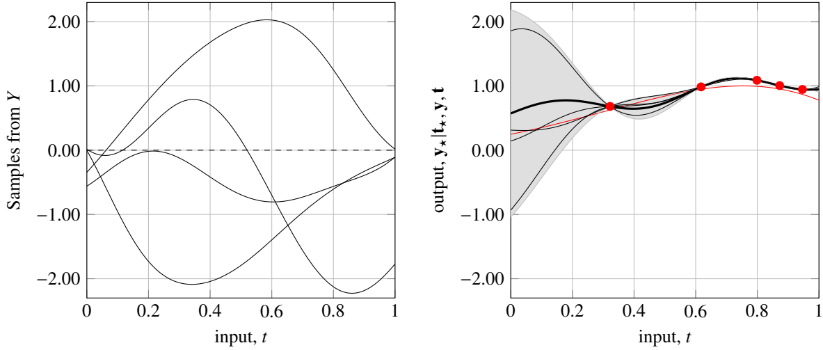
Figure 2.6: On the left: samples from a centered GP (black lines, as Figure 2.5), zero-mean is highlighted by a dashed line. On the right: mean \mathbb{E}(\mathbf{y}_\star | \mathbf{t}_\star, \mathbf{y}, \mathbf{t}) (thick black line) with 95% confidence interval conditionally (grey zone) to observed noisy samples (red dots) from a toy function (red line). Black lines are sampled from the conditional distribution (2.13).
