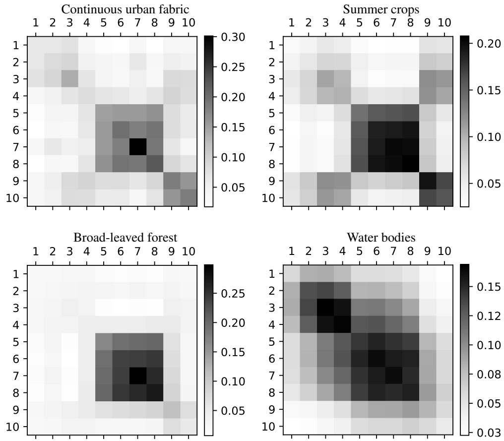
Figure 5.10: Estimated covariance matrices \mathbf{A}_c \mathbf{A}_c^\top on four land-cover classes.
