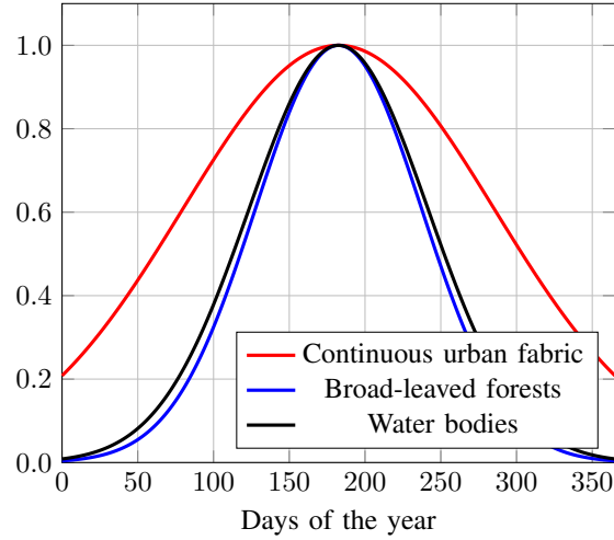
Fig. 3: Estimated RBF kernels for the IR wavelength and three different areas: artificial (continuous urban fabric), semi-natural (broad-leaved forests) and water (water bodies) areas. It shows the correlation between day of the year 180 and the other days, from day 1 to day 360.
