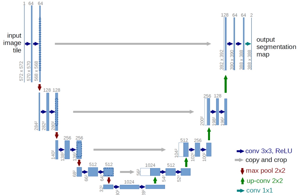
Figure 1.11: (Image from [150]). U-net architecture for pixel-wise classification.
