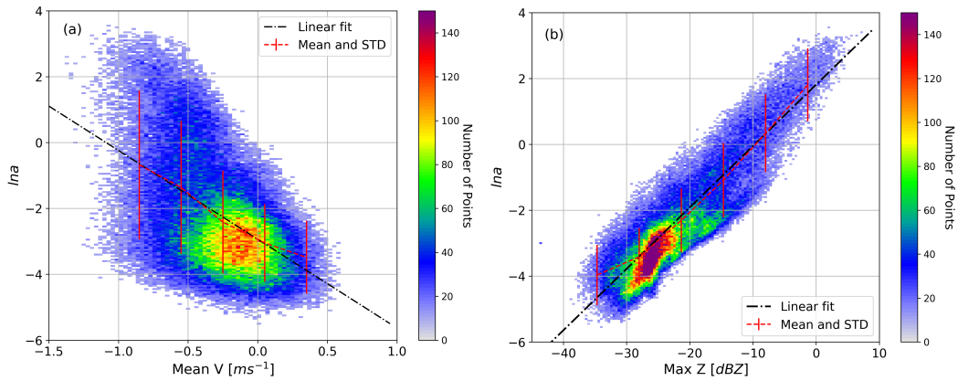
Figure 5.16: Correlation of (a) Mean velocity of the profile versus lna and (b) Maximum reflectivity of the profile versus lna for each cloud profiles, where colour bar indicates the number of profiles
