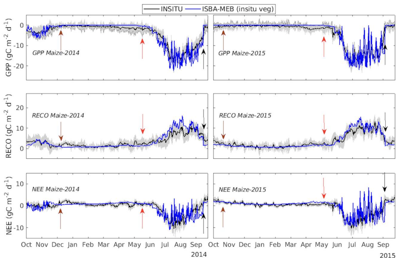
Figure 5.6c: Same as in Figure 5.4a , but for maize-2014, and maize-2015.
