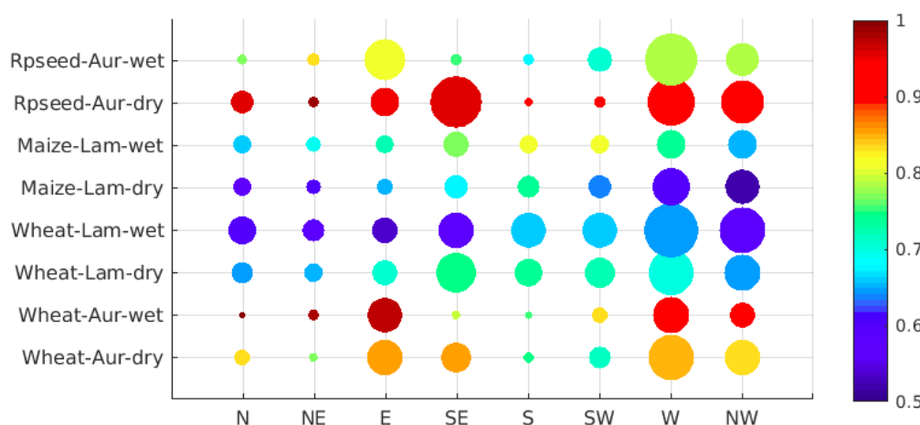
Figure 3.9: Distribution of the EBC in terms of the wind direction for the contrasting crop-seasons. High closure of 1 is presented in red, while blue indicates weak closure. The dot size represents the number of data points.
