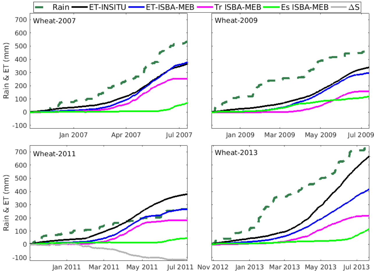
Figure 4.12: Comparing the cumulated rainfall with evapotranspiration ( ET ) from field measurements and ISBA-MEB estimates with plant transpiration ( Tr ), and soil evaporation ( Es ), for wheat at FR-Lam taken between the sowing and harvest dates.
