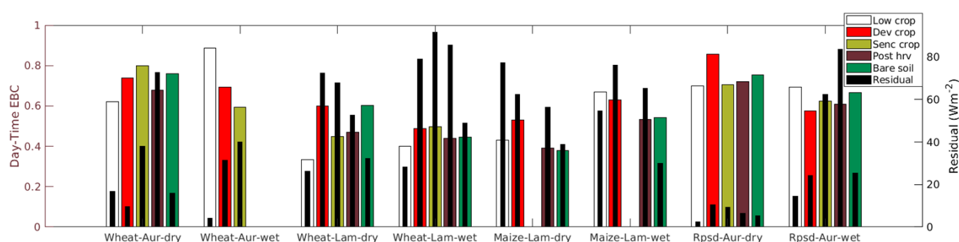
Figure 3.13: Daytime EBC (colored bars) and the corresponding residual (black bars) for the crop stages of the contrasting years. The colored bars also represent the different surface states: white corresponds to crops at the beginning of their development (Low crop), red to well-developed crops (Dev. crop), yellow corresponds to the senescent phase of the crop (Senc. crop), while brown and green stands for the post-harvest (post-hrv) and bare soil (Bare soil) periods respectively. Finally, the residual is to be read on the right-hand axis.
