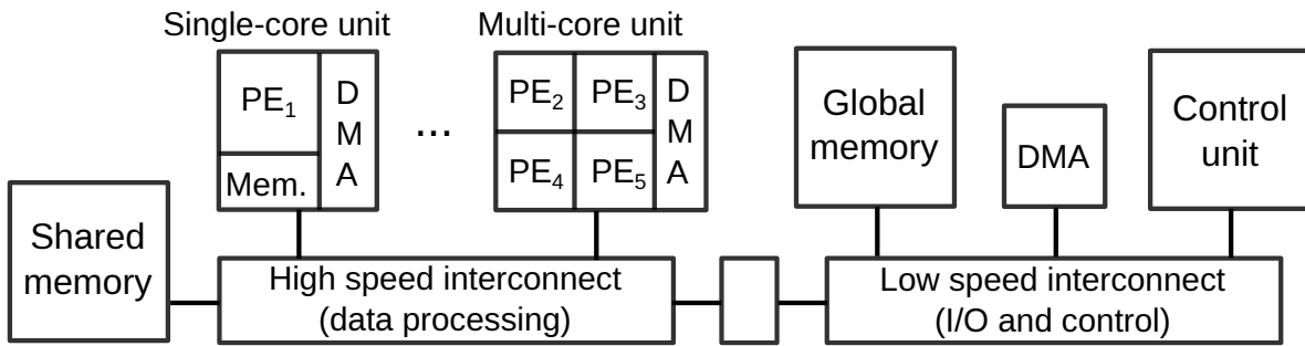
Figure 4.2: Target architecture
