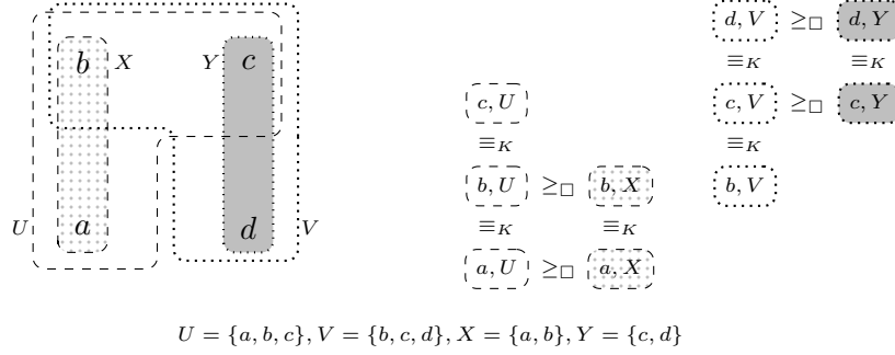
Figure 4.1: Example of a subset space (left) and its associated subset space frame (right).
