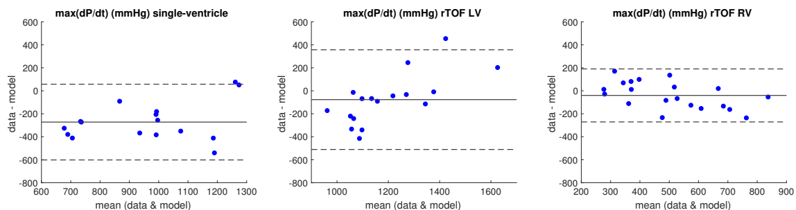
Figure 4.4: Bland-Altman plots for the difference between data- and model-derived \max(dP/dt) in single-ventricle (left), rTOF left (middle) and right ventricle (right) patients. Solid horizontal line is the mean of the difference between data- and model-derived \max(dP/dt) . Top and bottom dashed horizontal lines are the 95 % prediction interval ( \pm 1.96 standard deviation). LV: left ventricle; RV: right ventricle.
