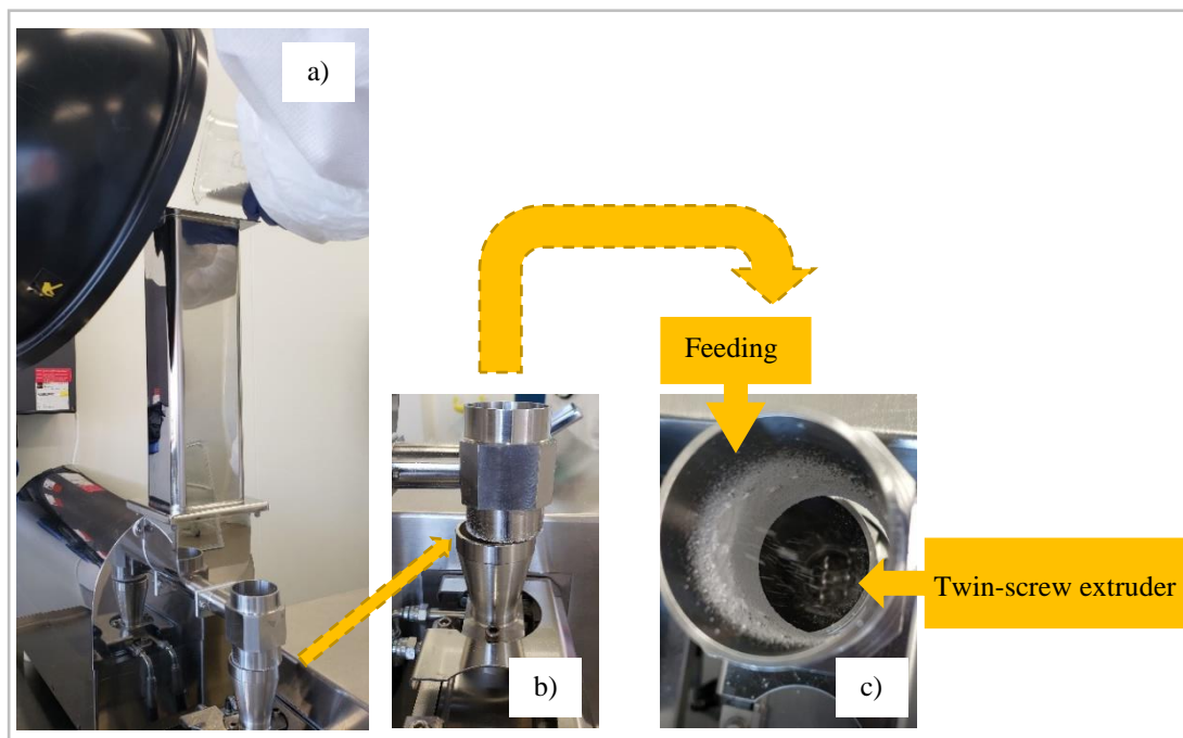
Figure 68. a) Gravimetric feeder; b) extruder feed hopper and, c) top view - mixing input into the extruder. Source: Author.
