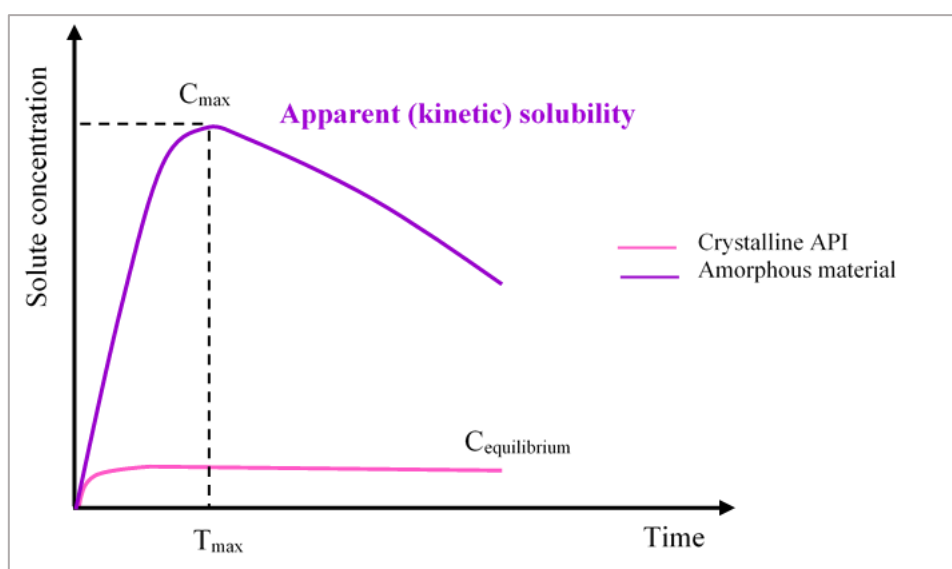
Figure 22. Schematic representation of kinetic solubility for amorphous and crystalline materials. Adapted from [184].
