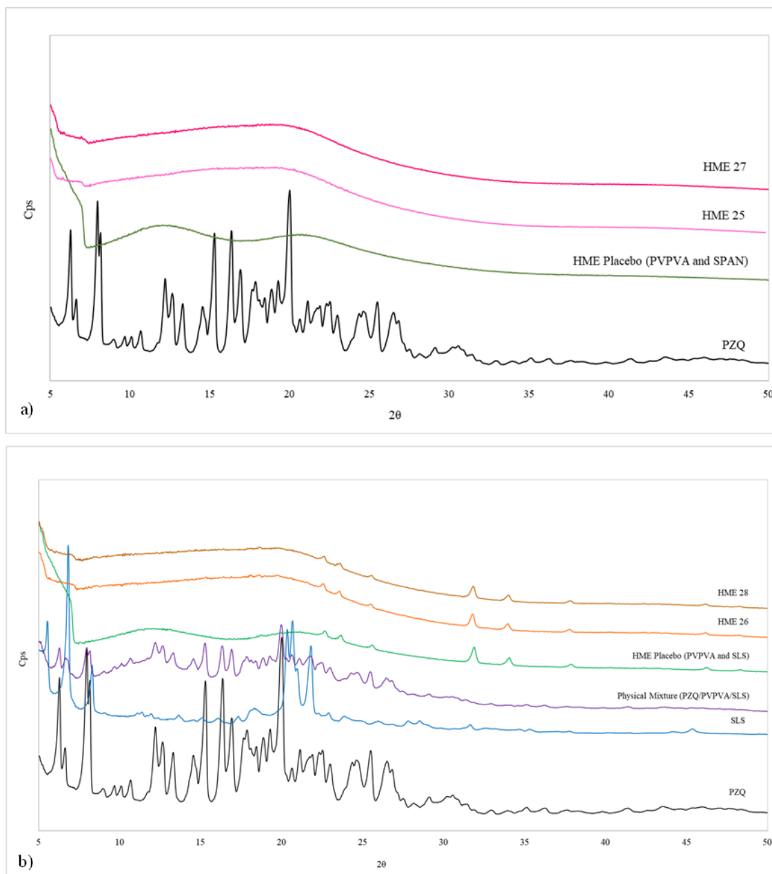
Figure 131. PXRD diffractograms for a) HME 25 and HME 27 (with SPAN 20) and the corresponding placebos, and b) HME 26 and HME 28 (with SLS), and corresponding physical mixture and placebo. Crystalline raw materials as given as references.
