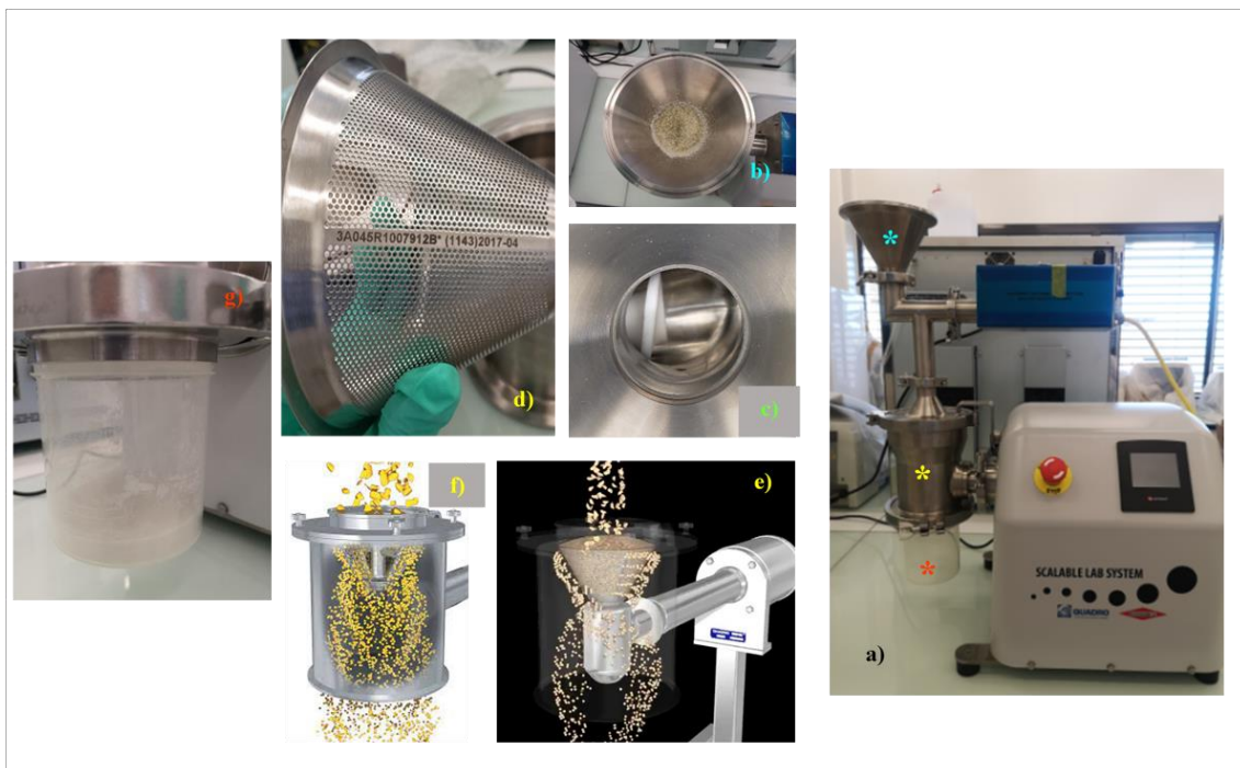
Figure 127. a) General view of Quadro® Comill with HE High energy Mill, b) material feed, c) feed screw, d) grinder, e, and f) different view of particle grinding, and g) collector. Source: Author and from [349].
