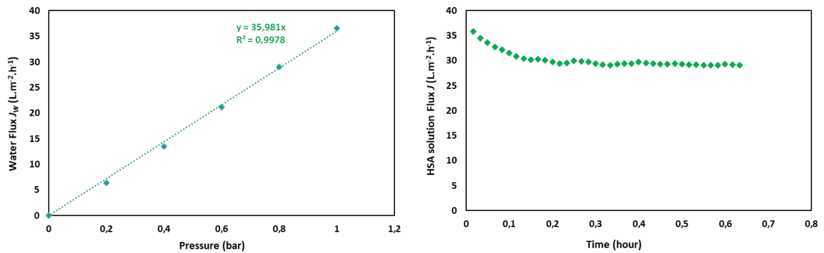
Figure 4. 15. Plot of the water flux versus pressure from which the permeability was calculated for membranes coated with PS 100 -b-PAA 107 and evolution of HSA solution flux versus time during HSA filtration (pH=5) through this same membrane.
