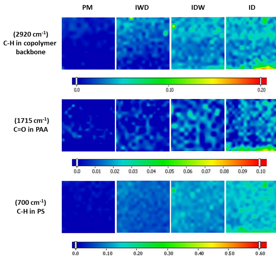
Figure 3. 14. FTIR maps obtained for three functional groups of the PS 30 -b-PAA 8 coated on PVDF membranes using different processes (IWD, IDW and ID), 2 hours of coating time and a copolymer concentration of 5 mg·mL -1 .
