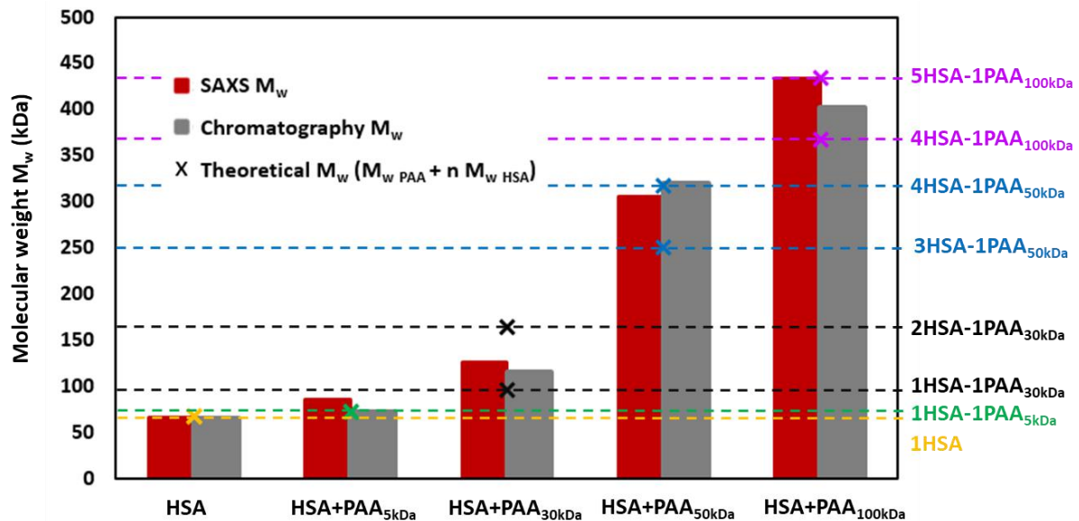
Figure 2. 32. Comparison on the HSA-PAA complex molecular weight estimated from SAXS data and from chromatography data to the theoretical M_w calculate from the stoichiometry of complexation (PAA-nHSA) for each size of PAA.
