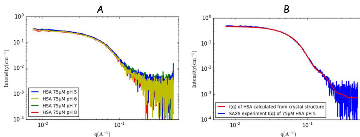
Figure 2. 20. A/ Scattering intensities of 75 \mu M HSA at different pH (5, 6, 7 and 8). B/ Scattering pattern of 75 \mu M HSA at pH 5 compared to theoretical pattern calculated from the crystal structure.
