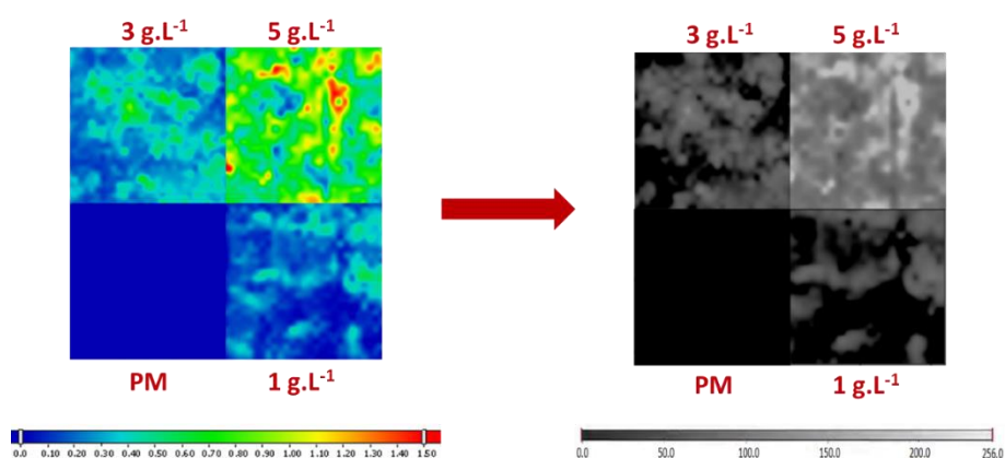
Figure 3. 12. Example of the conversion of a color-coded map generated for the peak at 700\text{ cm}^{-1} for the coating of \text{PS}_{30}\text{-b-PAA}_2 at different concentrations in solution as compared to a pristine membrane (PM), to a map coded with a grey scale.
