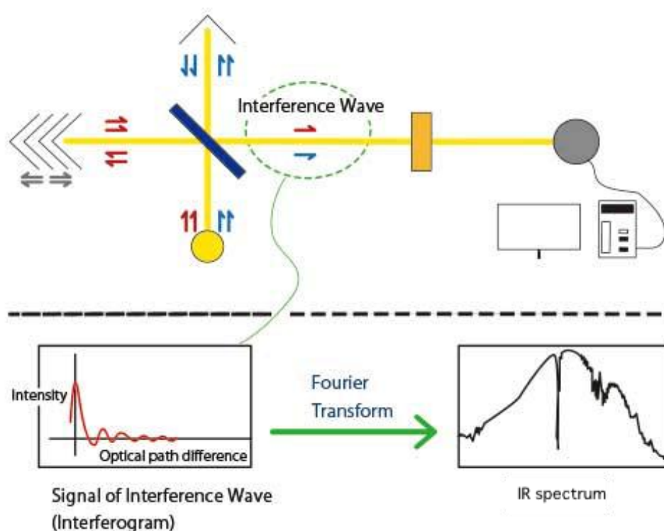
Figure 3. 9. Illustration of operating steps of the FTIR spectrometer to get to the sample spectrum.
