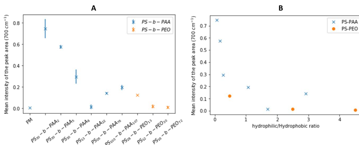
Figure 3. 21. The intensity average of the peak area at 700 cm -1 as shown A/ for the coating of different PS-b-PAA and PS-b-PEO using ID process, 2 hours of immersion time and a copolymer concentration of 5 mg·mL -1 and B/ the intensity as a function of the hydrophilic/hydrophobic ratio.
