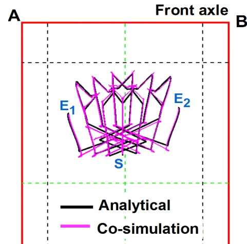
Figure 5.36: ZMP estimation through analytical and co-simulation
