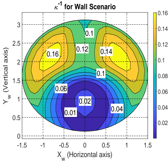
Figure 5.28: Inverse of condition number ( \kappa^{-1} ) for wall scenario
