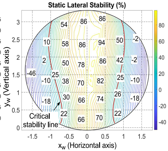
Figure 5.6: Contour: Static lateral stability - Wall scenario
