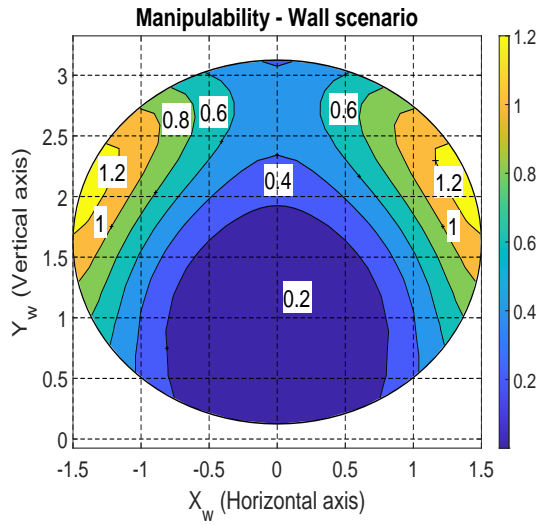
Figure 5.29: Manipulability ( w ) for wall scenario
