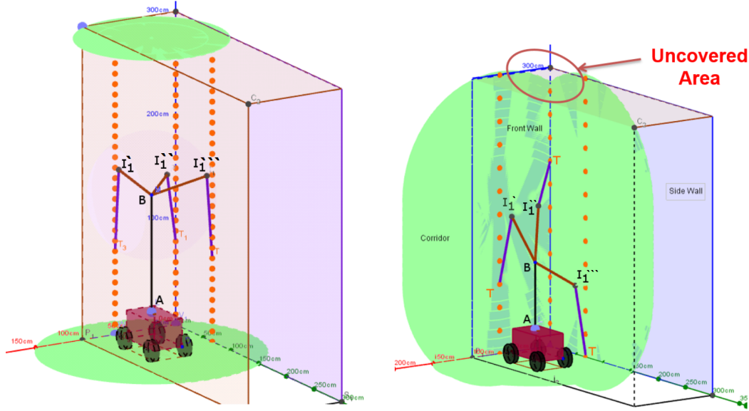
(a) Three arm positions to show accessibility to front wall, lateral wall and the corner
