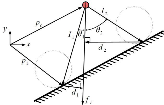
Figure 2.9: Concept of force angle stability margin [Papadopoulus and Rey, 1996]
