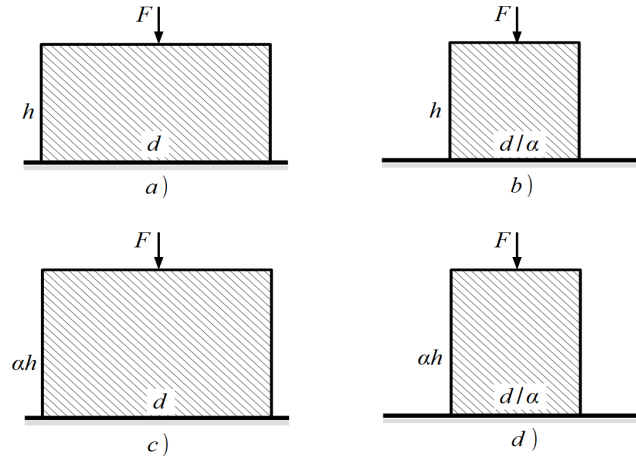
Figure 2.13: Effect of top-heaviness on stability [Mahdi and Nestinger, 2012]
