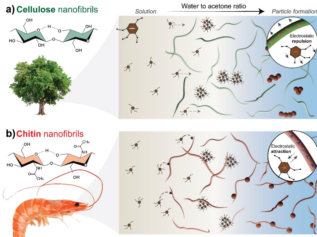
Figure III.10. Schematic illustration of the solvent exchange process that leads to the nucleation and growth of lignin nanoparticles in the presence of a. cellulose and b. chitin nanofibers, both of which acted as templating supports. From an increased water-to-acetone ratio, lignin nanoparticles (LPs) were formed with a morphology that is controlled by the surface chemistry of the nanofibers. As such, LPs are formed loosely in suspension with non-interacting cellulosic templates. Conversely, strongly anchored LPs were formed on the surface of the chitin nanofibers, via electrostatic effect.
