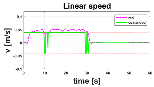
(b) Game termination
