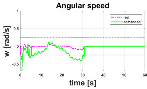
(c) Pursuer's strategy
