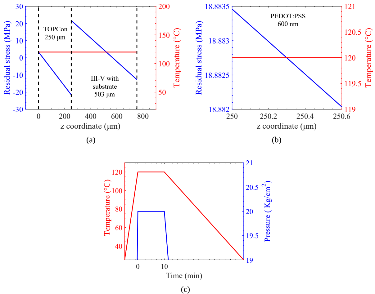
FIGURE 5.25 Temperature profile and thermal residual stress after cooling to room temperature ( T = 25^\circ\text{C} ) in the III-V/PEDOT:PSS/Si stack under a uniform gluing temperature of 120^\circ\text{C} (a) in the whole system, (b) in the PEDOT:PSS layer. (c) The evolution of temperature and pressure over time during the lamination step.
