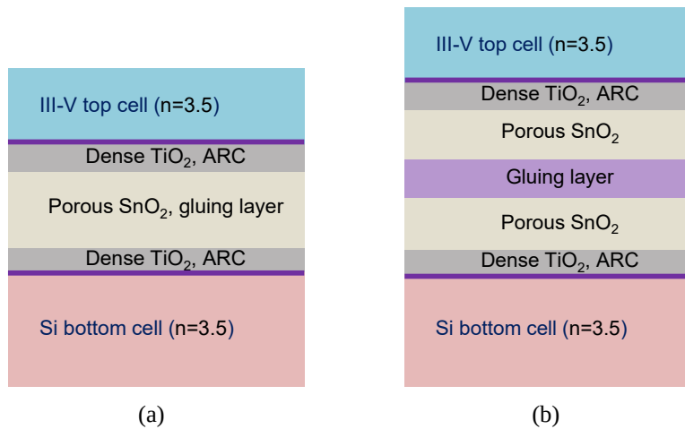
FIGURE 3.17 Sketch of possible TCL stacks using SnO 2 film.
