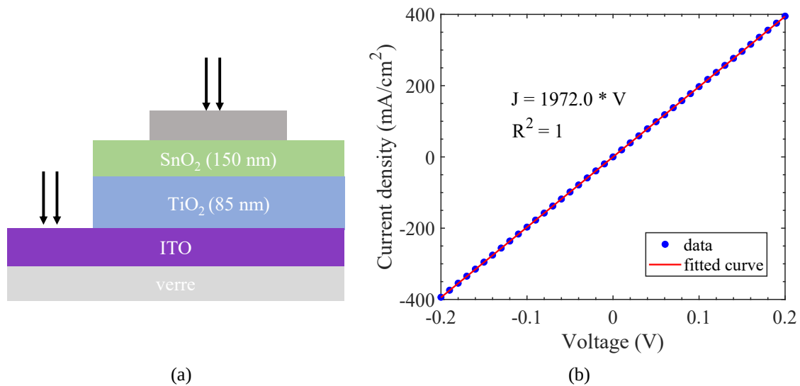
FIGURE 3.18 (a) Sketch of the sample used for electrical evaluation between SnO 2 and TiO 2 fabricated with our process and (b) Resulting JV curve of the complete stack measurement, showing perfect ohmic contact with low resistivity.
