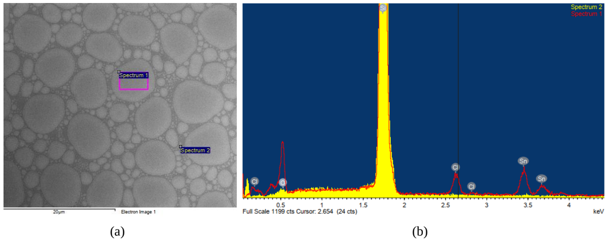
FIGURE 3.16 (a) SEM image of a fume deposition, coming from a spin-coated \text{SnO}_2 film at 400^\circ\text{C} , on a silicon substrate, (b) EDX spectra: spectrum 1: red line for the area inside a spot of deposited materials and spectrum 2: yellow filled curve for the region without deposited materials.
