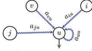
Figure 5.3: Example of the message-passing.
