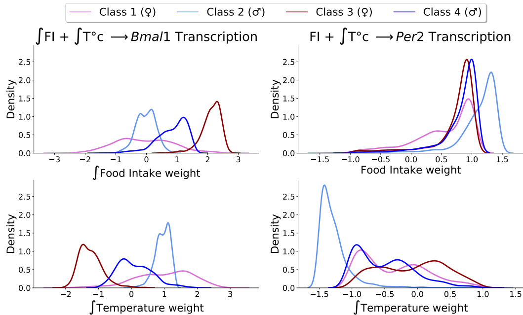
Figure 4.8: Density plot of the coefficients of the best 2-term model for Bmal1 and Per2 , computed across residual trajectories for each mouse class. FI: Food Intake, T°C: Temperature.
