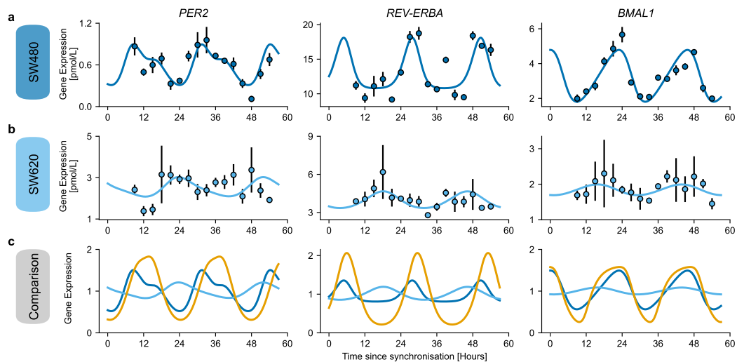
Figure 3.3: Comparison of the core-clock models fitted to healthy mouse liver or human cancer cell lines. Best fit of the quantitative core-clock model to (a) the SW480 cell line and (b) the SW620 cell line. Model simulation (line) against the RT-qPCR data used for calibration (dots), depicted as mean values ( n = 3 ) \pm SEM. c Comparison of the model fit for liver (orange), SW480 (dark blue) and SW620 (sky blue). Bmal1 circadian phases were aligned for mouse liver and SW480 cell line and all gene expression profiles were normalized to the mesor to allow for comparison. See Fig. 2.S2 for the other genes of the core clock model.
