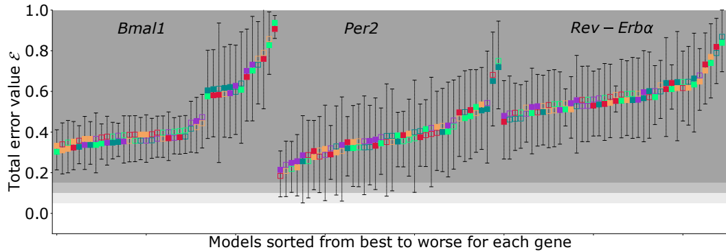
Figure 4.S4: Total error for each of the 40 2-terms models, for all genes. Mean and standard deviation were computed across residual trajectories under (H2-H3) . Colored squares at the mean describe the regulators involved for each model, with the top square referring to the dominant regulator. Areas defined by different shades of gray refer to thresholds of total error equal to 0.05, 0.1 and 0.15.
