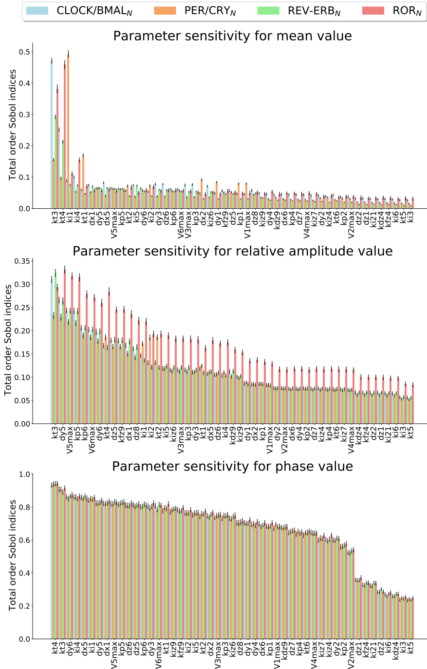
Figure 4.S1: Sensibility analysis performed on the mean, relative amplitude and phase of the modulatory variables of the in vitro circadian clock model. Total order sobol indices plotted, with estimated standard deviations. Parameter definitions provided in Supplementary Section S2-1.2.
