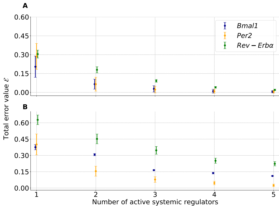
Figure 4.6: For each gene, the total error of the best-fitting model depending on its number of nonzero terms is reported for Transcription (A) and Degradation (B). Standard deviations are taken across residual trajectories.
