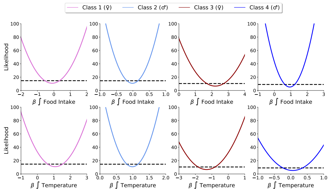
Figure 4.S5: Profile likelihood obtained for Bmal1 best 2-term model under (H1-H3) . Black dashed lines delimit the 95% confidence interval in which the parameters are identifiable.
