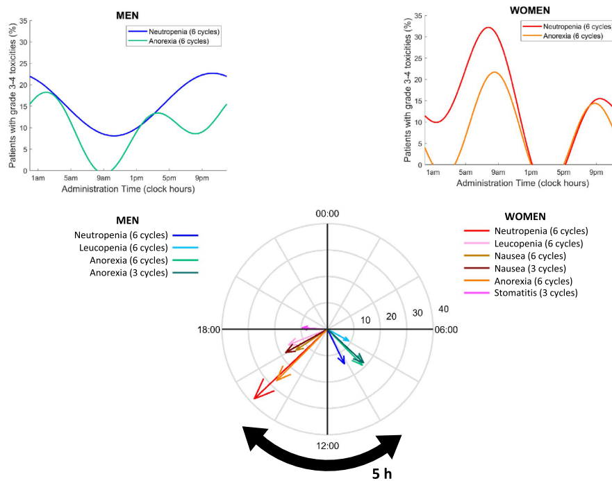
Figure 2.10: Main chronotoxicities according to irinotecan timing and sex. Top: best fit cosine curves for percentages of men and women with grade 3–4 neutropenia or anorexia over six cycles with respect to irinotecan timing. Bottom: polar plots highlighting the sex-specific clock hours associated with minimum incidence of toxicities. For each toxicity, the arrow's length and angle represent amplitude and clock time of minimum value of the best-fit cosine, respectively. Only toxicities with significant cosinor tests are displayed ( P < 0.05 ). From (Innominato et al., 2020a). CC BY 4.0 Licence
