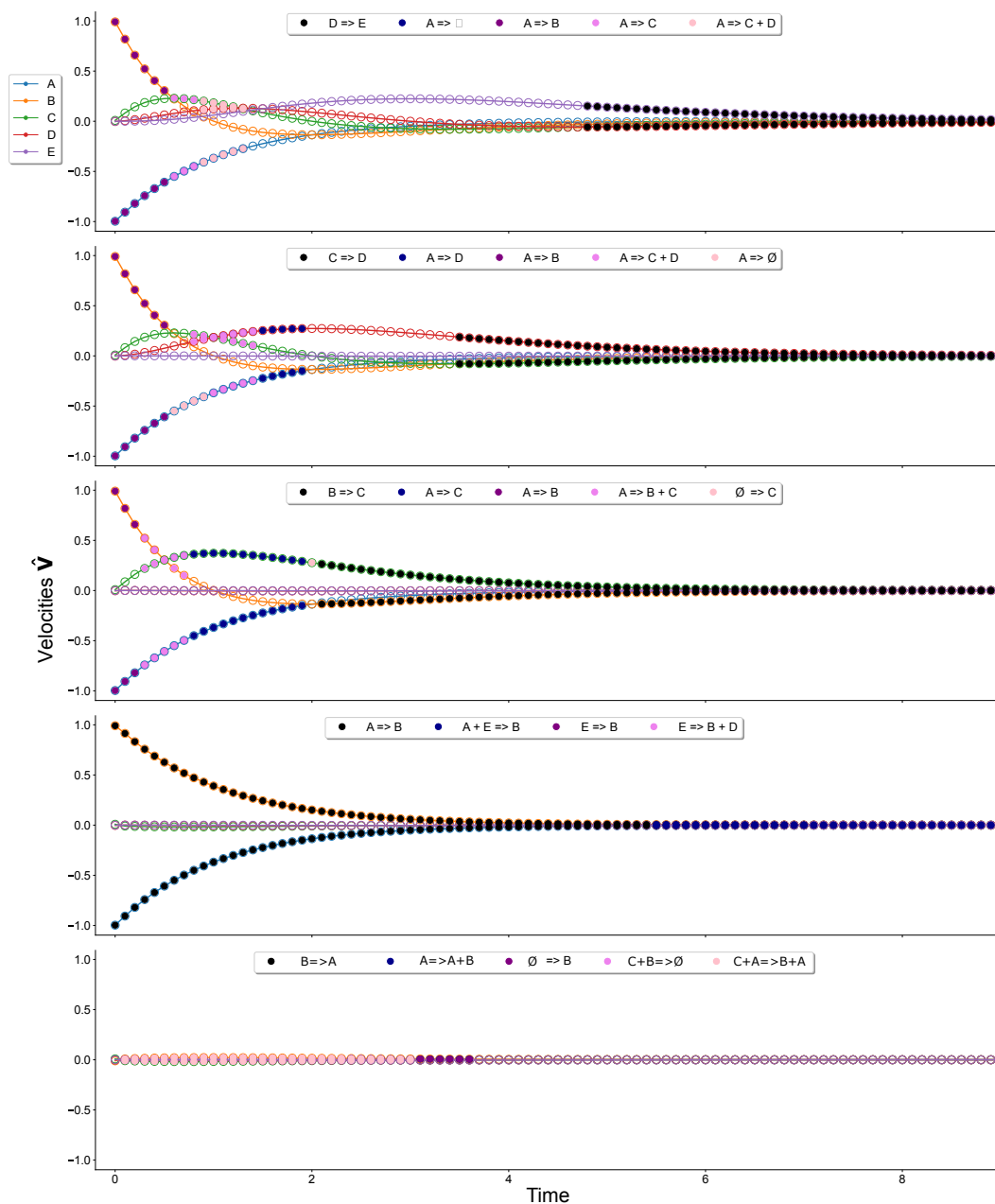
Figure 5.2: Plot of the support of inferred reactions for the chain CRN A \xrightarrow{1} B \xrightarrow{1} C \xrightarrow{1} D \xrightarrow{1} E . Each row represents the velocities \hat{V} after the effect of a reaction is removed, except for the first row. At each step, the 5 top ranked reactions (from left to right in the legend) in terms of loss value are printed on top. For each time point, the color filling the dot associated to a species velocity reveals what reaction was considered. For this example, Reactmine parameters were set to \alpha = 0.25 , \lambda = 0.7 , \delta_{\max} = 3 .
