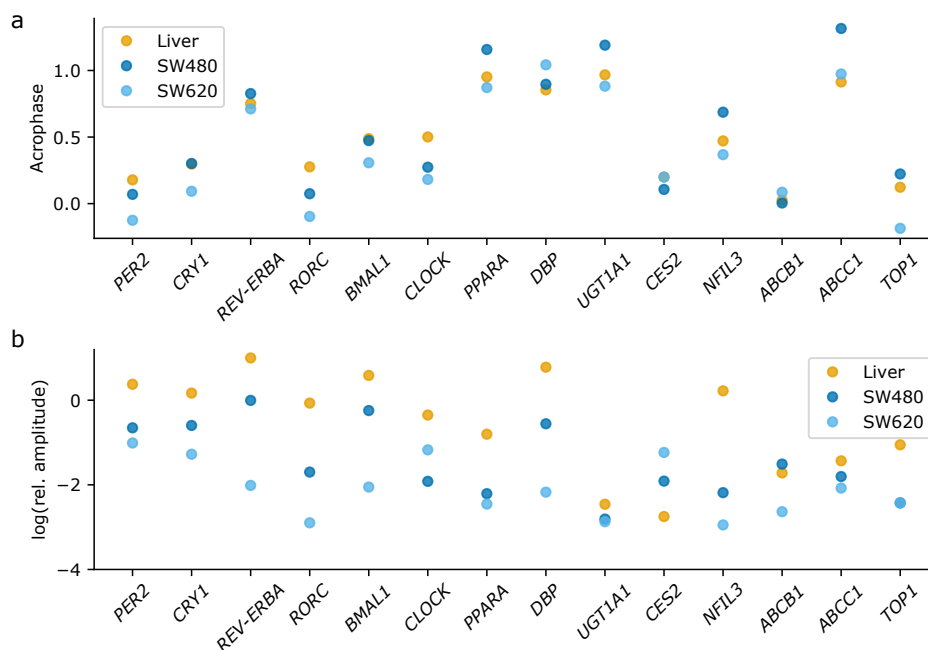
Figure 2.S5: Oscillation comparison for different model fits. Comparison between liver, SW480 and SW620 regarding (a) acrophase (rescaled to the interval from zero to one, values below zero and above one are for visualization and represent the phase modulo one) and (b) relative amplitude.
