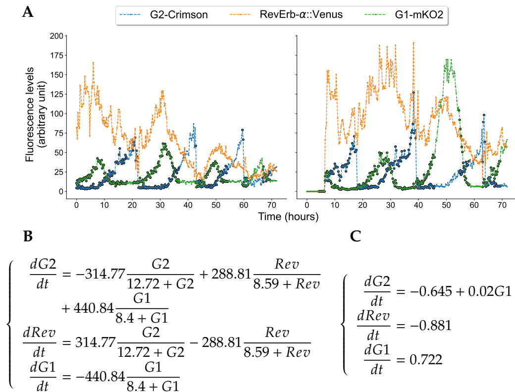
Figure 5.7: Inference results on the videomicroscopy data. (A) Plots of fluorescence levels reported in two cells among the 91 of the dataset. Black-circled data points corresponds to points where the reaction G1 \Rightarrow G2 was inferred by Reactmine. (B) ODEs representation of the CRN inferred by Reactmine. Parameters of the algorithm were set to \delta_{\max} = 3 , \alpha = 6.5 , \lambda = 0.7 . (C) System of ODEs learned by SINDy with \lambda = 0.04 .
