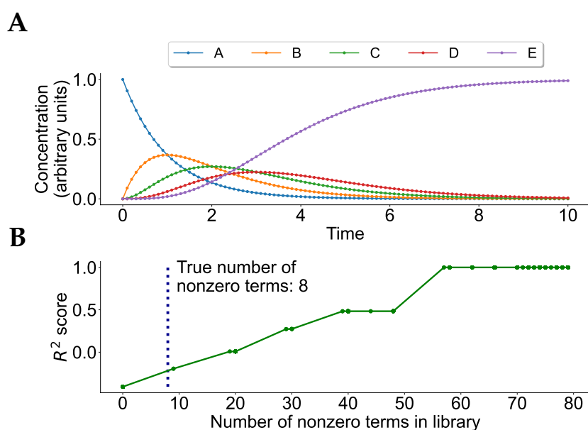
Figure 2.5: (A) Numerical simulation of a linear chain of reactions (Equation (2.3)) A \Rightarrow B \Rightarrow C \Rightarrow D \Rightarrow E , each reaction with mass action law coefficient set to 1. (B) R^2 score provided by SINDy as a function of the number of terms included in ODEs system, which is directly related to the choice of \lambda in Equation (2.13).
