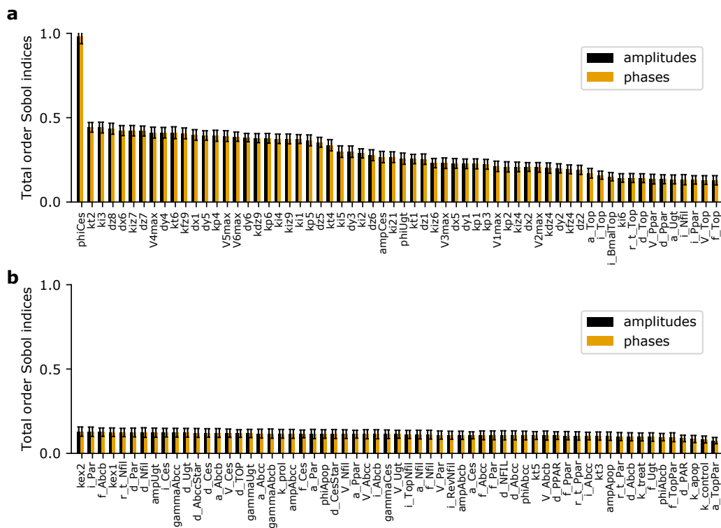
Figure 2.S9: Sensitivity analysis of the full clock-PK-PD model. Total order Sobol indices estimated for the clock-irinotecan model with respect to phase and amplitude of irinotecan circadian toxicity profile, for details see Section S2-1.4. Transcription fold changes and Hill coefficient were excluded to reduce the number of parameters. For the circadian degradation associated with the dynamical variables CES, UGT, ABCB and ABCC, phi plus variable name denotes the phase, amp plus variable name denotes the amplitude, and gamma plus variable name denotes the mesor of the degradation oscillation. 10 000 simulations of the model were used for the estimation. a Parameters with high sensitivity (more sensitive half). b Parameters with low sensitivity (less sensitive half).
