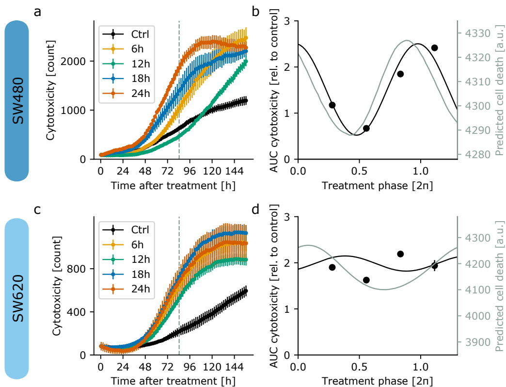
Figure 2.S7: Predictions of the original PK-PD model. a Cytotoxicity measured as the number of dead cells, counted as number of red objects in the experimental setup, for the full duration of the experiment. For the analysis, the time till 84.5 hours (grey dashed line) is used to prevent saturation effects. b Area under the curve of the experimental data (till 84.5 hours) and the harmonic regression line predicted by cosinor analysis (black line) compared with the model predictions using the model from Dulong et al. (2015) with replace protein dynamics, adapted to CRC cells as described in Section S2-3.2 . The predicted phase of maximal toxicity (grey line) fits for the SW480 cell line, but the predicted amplitude is too low. c Cytotoxicity for the SW620 cell line. d Area under the curve for the experimental data (till 84.5 hours) for SW620 cell line compared to model predictions. Harmonic regression showed no significant result for the SW620 cell line.
