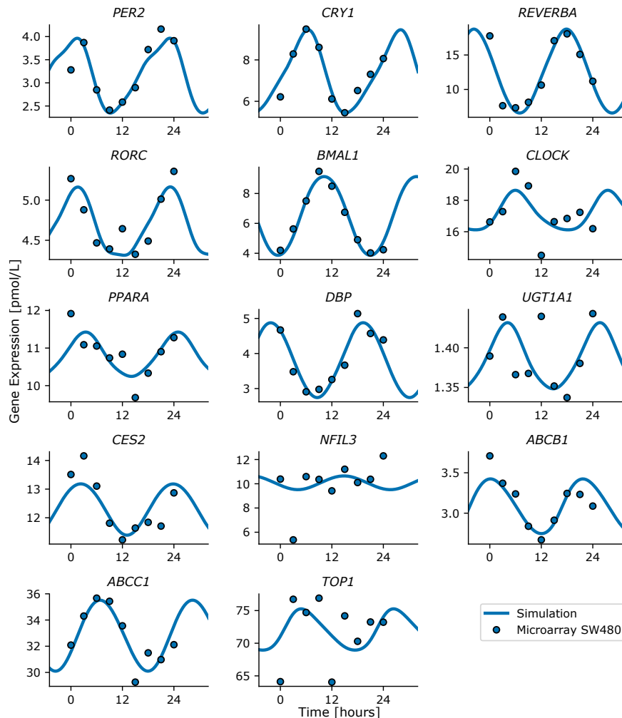
Figure 2.S4: Example of a full model fit. Model fit (line) of the mRNA expression data (dots) for the SW480 cell line.
