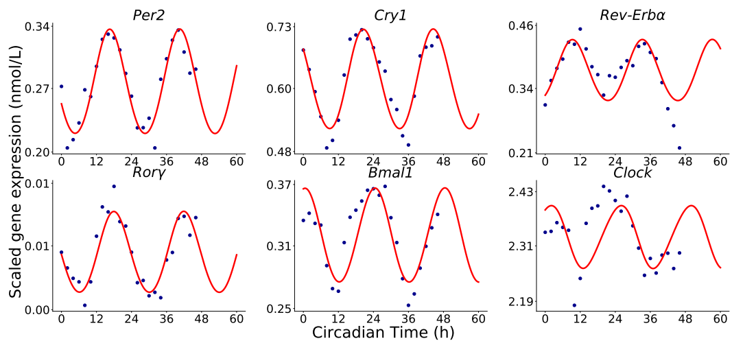
Figure 4.3: Best-fit of the in vitro cellular clock model (red curves) to mRNA levels of six clock genes measured in MMH-D3 cell culture (blue dots)
