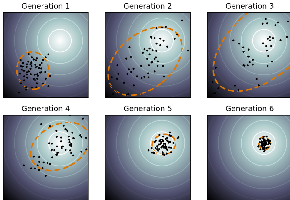
Figure 2.2: Illustration taken from Wikipedia, of an optimization run using CMA-ES on a simple two-dimensional minimization problem. The spherical optimization landscape is depicted with solid lines of equal function values. The population (dots) shows how the multi-variate normal distribution of the population (dotted line) changes during the optimization.
