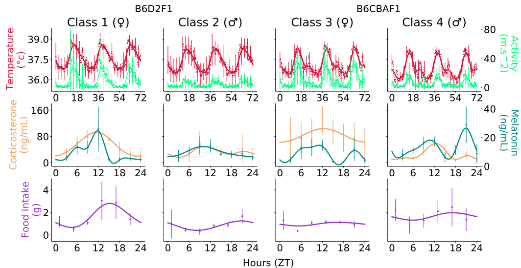
Figure 4.2: Circadian biomarkers in four mouse classes. Raw data are represented with dots (average) and error bars (standard deviations). For the sake of readability, error bars were only displayed every 2.5 hours for the first line. Solid lines stand for the mean function obtained by fitting a Gaussian Process.
