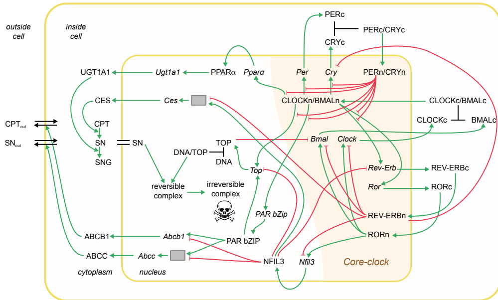
Figure 3.4: Model of the interplay between irinotecan PK-PD and the core clock. Irinotecan treatment is simulated by a transcriptional-translational network that comprises the core clock, irinotecan-relevant genes, and the PK-PD of irinotecan. Different types of interactions are represented among the elements of the network: inhibition (red arrows with flat arrowhead) and activation interactions (green arrows); complex formation (black lines). Grey boxes represent post-transcriptional sub-networks necessary for a model fit to the data. The double black line indicates equal concentrations between nucleus and cytoplasm, the double black line with arrowheads indicates CPT-11 and SN-38 cellular transport inside and outside of the cell. All indicated molecular interactions are based on experimental evidence from a number of different sources and corresponding references are provided in Table 2.S3.
