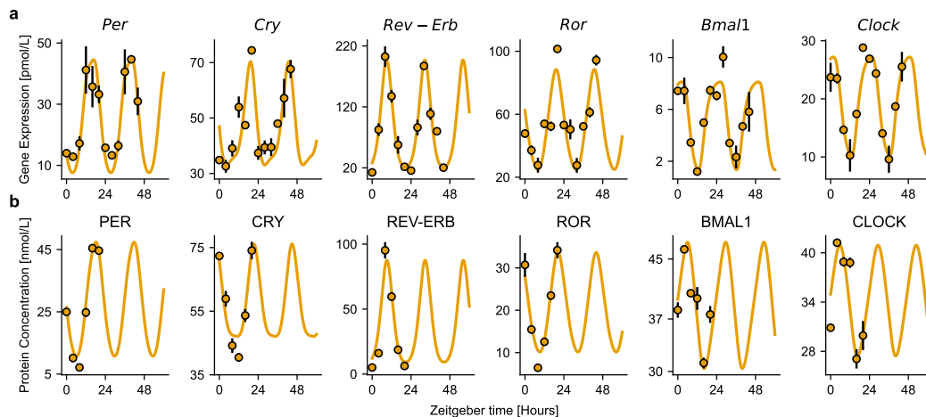
Figure 3.2: Best fit of the quantitative core-clock model to mRNA and protein circadian datasets in the mouse liver. a mRNA expression for core-clock elements in pmol/L. b Protein levels for core-clock elements in pmol/L. Model simulation (orange lines), experimental data used for calibration (black circles). Depicted are mean values ( n = 2 biological replicates) \pm SEM.
