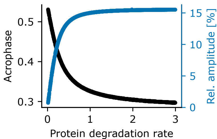
Figure 2.S6: Translation parameters of the irinotecan-relevant proteins CES2, UGT1A1A, ABCB and ABCC. Scanning the range of possible translation parameters shows that only the protein degradation rate changes acrophase and relative amplitude significantly. Compromising between a large oscillation amplitude and a phase delay of at least around 4 hours between mRNA and protein peak, we choose a degradation rate of 1.2.
