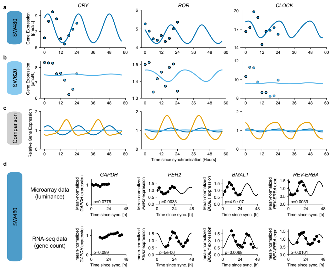
Figure 2.S2: Fit of the core-clock model to cell lines derived from human cancer. This supplements Fig. 3.3 of the main text, showing the remaining genes of the core-clock. a Fit (line) and experimental data (dots) for the SW480 cell line and (b) the SW620 cell line. c Comparison of the model fit for liver (orange), SW480 (dark blue) and SW620 (sky blue). Bmal1 circadian phases were aligned for mouse liver and SW480 cell line and all gene expression were normalized to the mesor to allow for comparison. d Comparison of microarray and RNA-seq time series data for the reference gene GAPDH and the core-clock genes measured for the RT-qPCR data of the SW480 and SW620 cell lines. GAPDH is particularly well suited as reference gene as it is expressed at a much higher abundance compared to core-clock genes, and it does not show circadian oscillations, as confirmed by a cosinor analysis with non-significant p-values for GAPDH. Experimental mean-normalized measures (dots) with the result from a harmonic regression (lines), using a p-value threshold of p=0.05 .
