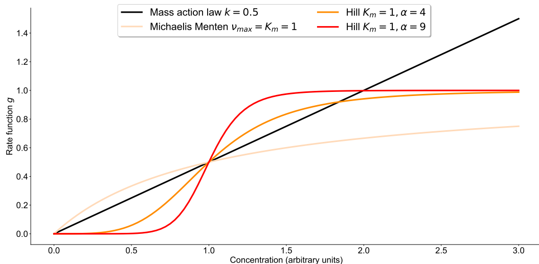
Figure 2.1: Several rate functions plotted against reactant concentration.
