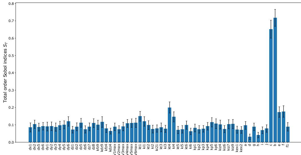
Figure 2.S1: Total order Sobol indices. 100 000 simulations of the model were used for the estimation.
