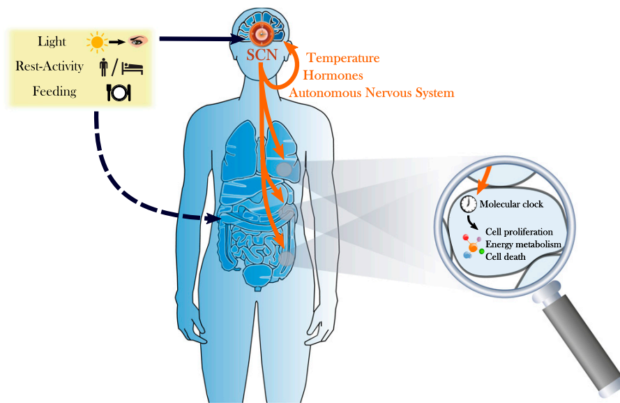
Figure 2.7: The Circadian Timing System. Figure taken from (Ballesta et al., 2017). CC BY 4.0 Licence
