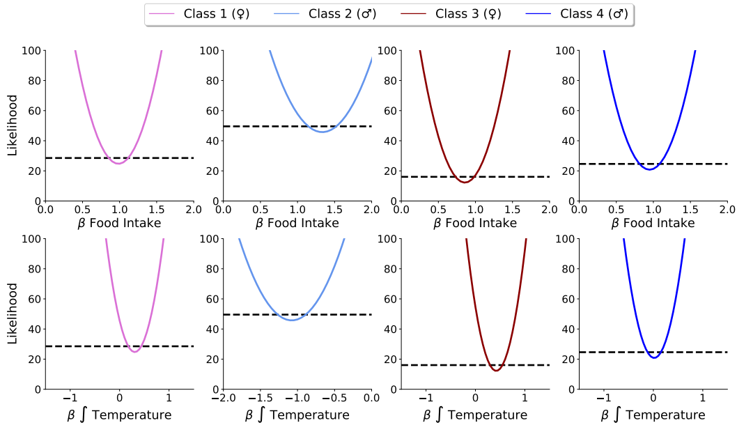
Figure 4.S6: Profile likelihood obtained for Per2 best 2-term model under (H1-H3). Black dashed lines delimit the 95% confidence interval in which the parameters are identifiable.
