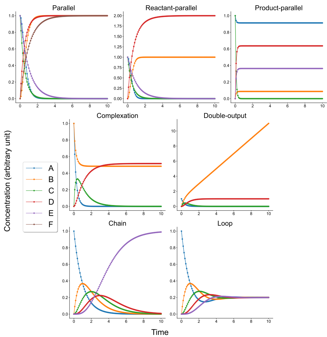
Figure 5.S1: Numerical simulation of the toy CRNs.
