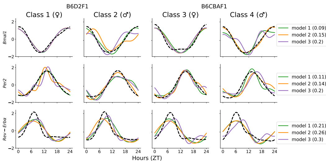
Figure 4.S3: Fit of one residual trajectory (dashed black curves) for each gene and each class. 3 different models (solid colored curves) are used for the sake of error visualization.
