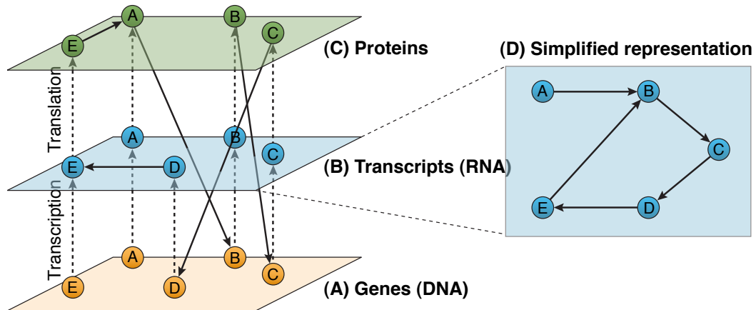
Figure 2.4: Illustrative example of a gene regulatory network. From Marbach (2009) .
