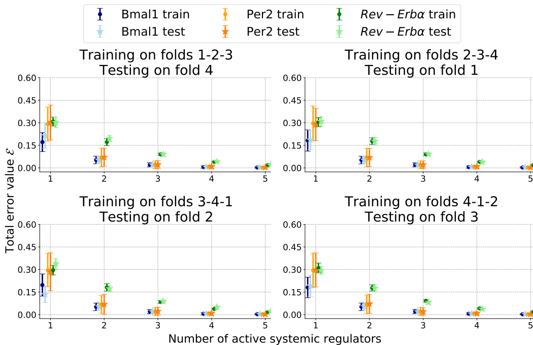
Figure 4.S2: For each gene, the total error of the best-fitting model depending on its number of nonzero terms is reported under (H1-H3) . Timepoints were shuffled and divided in 4 folds on which 4-fold cross validation was performed.
