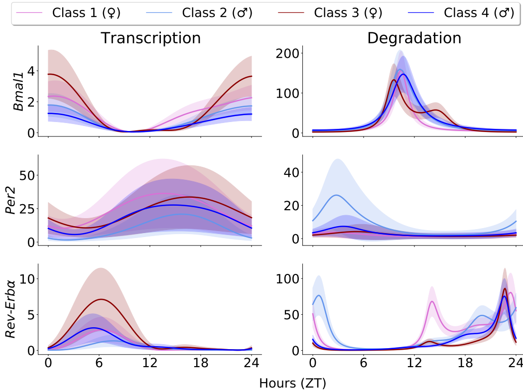
Figure 4.4: Mean and standard deviation of the selected residual trajectories obtained for each clock gene. Left (resp. right) panels under (H1-H3) (resp. (H2-H3) ).
