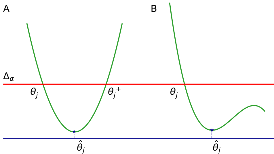
Figure 2.3: Potential likelihood profiles. Panel (A) shows an identifiable parameter \hat{\theta}_j with confidence interval [\theta_j^-, \theta_j^+] . Panel (B) shows a non practically identifiable parameter since the profile only passes the threshold once.
