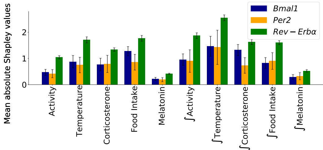
Figure 4.5: Mean absolute Shapley values for all features and each gene under (H1-H3). Standard deviations computed across residual trajectories.
