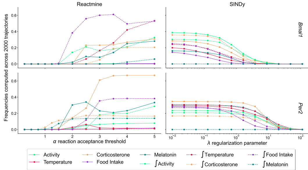
Figure 5.8: Inference of systemic drivers of clock gene transcription by Reactmine and SINDy. For Reactmine, \lambda was set at 0.7 and \delta_{\max} to 3.
