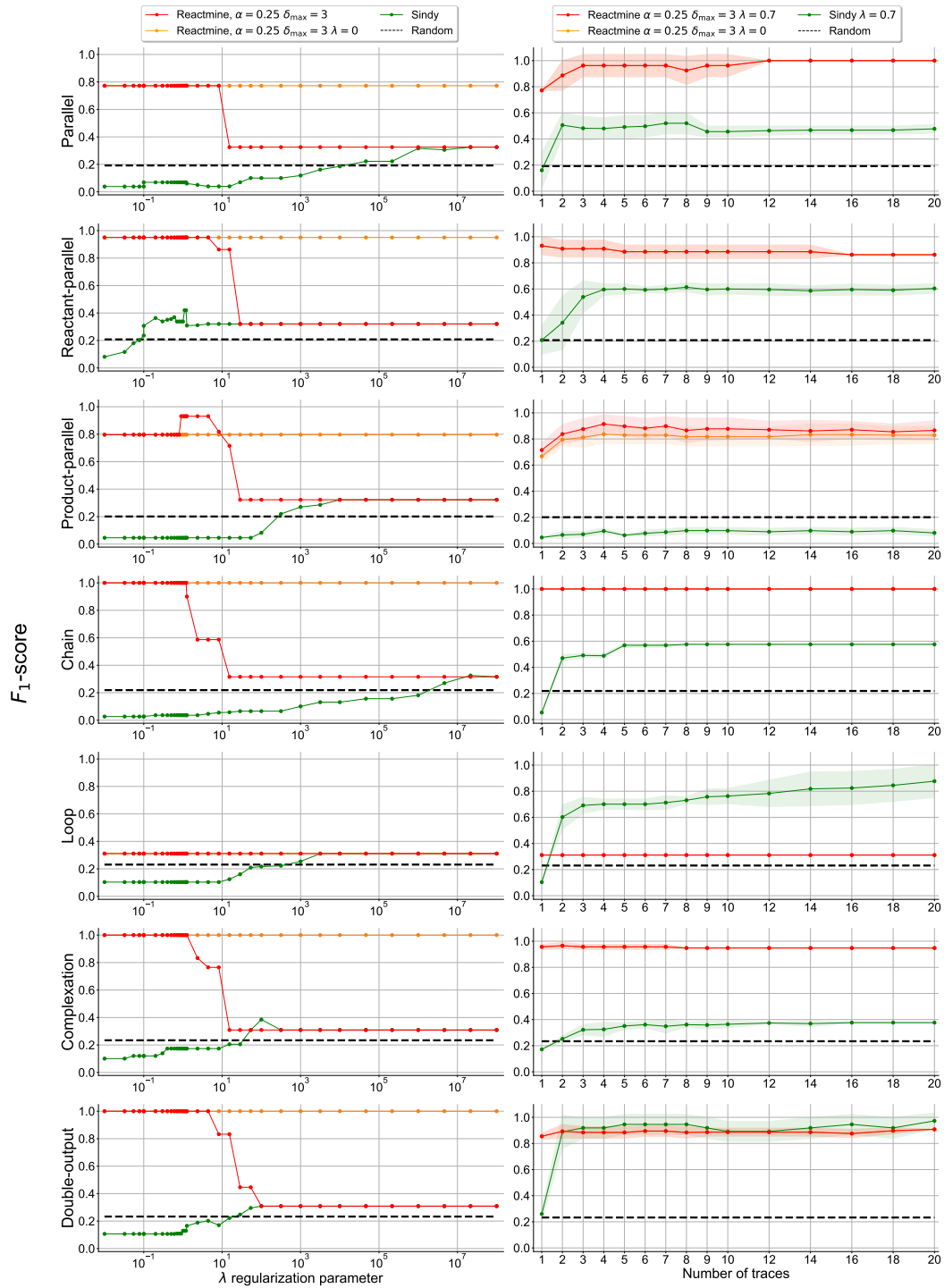
Figure 5.4: Inference results of Reactmine and Sindy for each toy CRN. The first column considers a single canonical trace and gives the performances as a function of \lambda the regularization parameter of both methods. The second considers multiple traces. Standard deviations originate from the fact that the evaluation was performed on different traces 6 different times.
