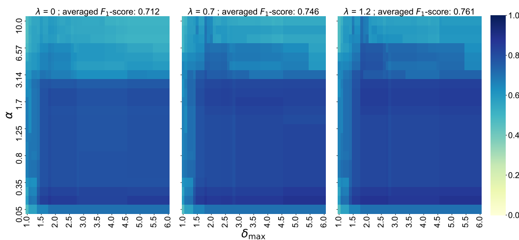
Figure 5.5: Sensitivity of Reactmine to \alpha , \delta_{\max} and \lambda parameter change. The measured output is the F_1 -score, averaged across all toy CRNs. On top of each subplot, the F_1 -score averaged across the grid of (\alpha, \delta_{\max}) values is reported.
