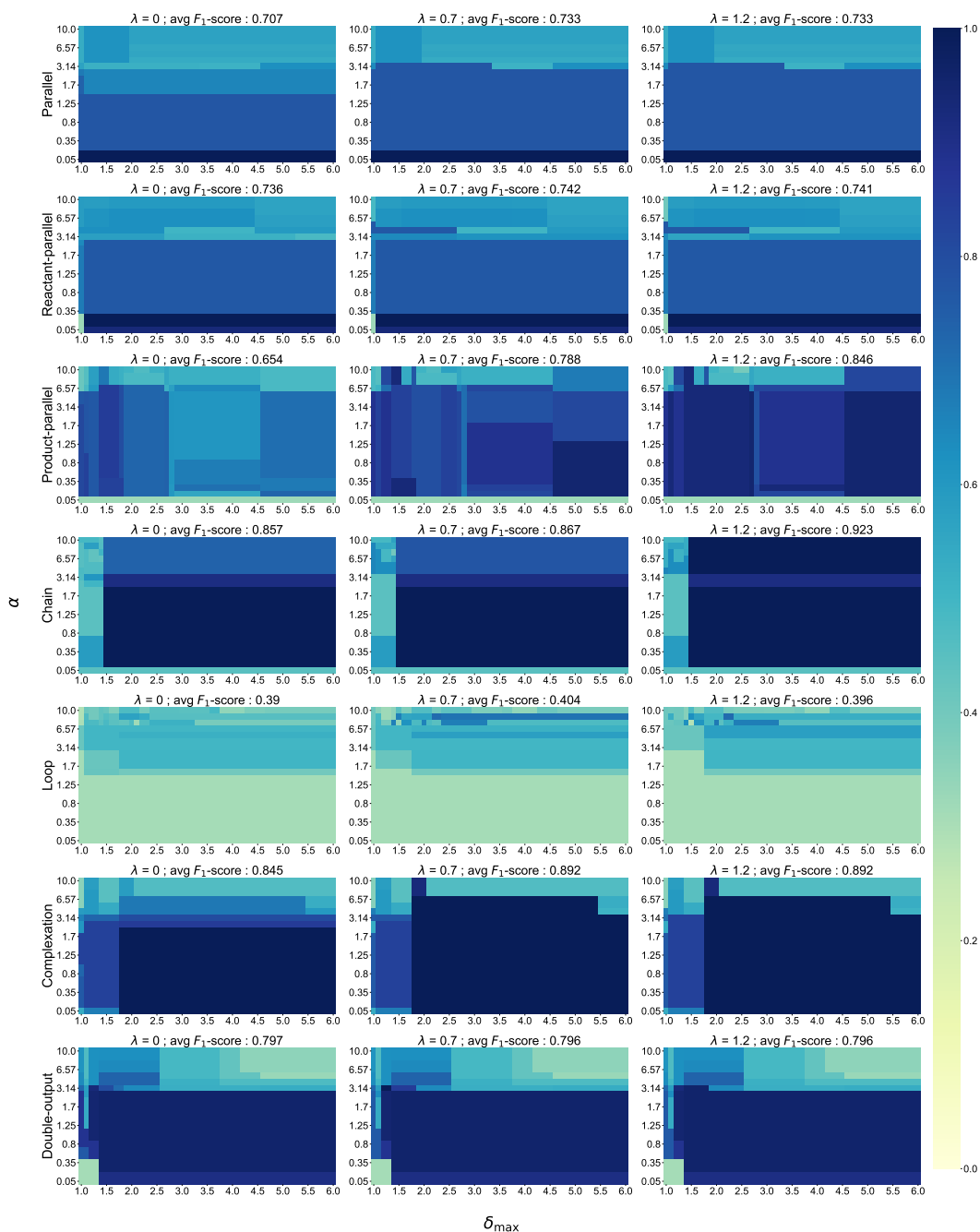
Figure 5.6: Sensitivity of Reactmine to \alpha , \delta_{\max} and \lambda parameter change, for each CRN. The measured output is the F_1 -score. On top of each subplot, the F_1 -score averaged across the grid of (\alpha, \delta_{\max}) values is reported.
