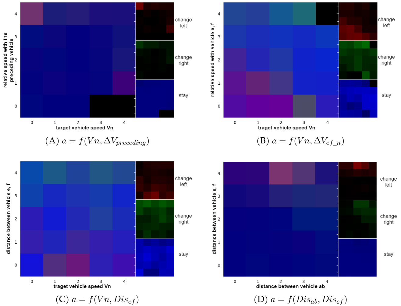
Figure 4.8 – Color maps for the learned policy. red: change left, green: change right, blue: stay in the current lane.
