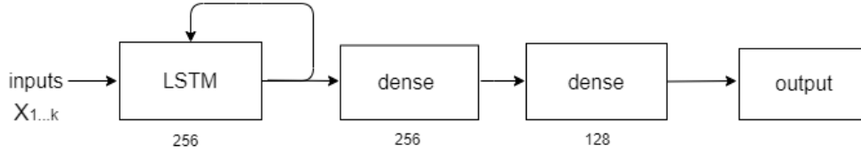
Figure 5.1 – M1: The reference architecture (Alché and La Fortelle, 2017) uses a first layer of 256 LSTM cells, followed by two dense (fully connected) hidden layers of 256 and 128 neurons respectively and a final dense output layer containing as many neurons as the number of outputs.
