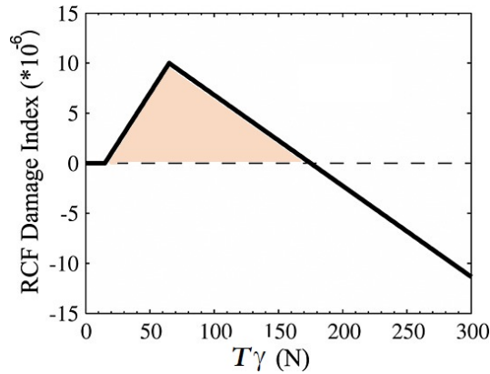
Figure 3.10: Derived RCF damage index as a function of T_\gamma . Adapted from [129]
