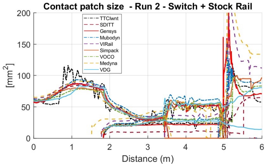
Figure 4.17: Contact patch size for the Run 2, considering the diverging route with the British S&C. From [102]
