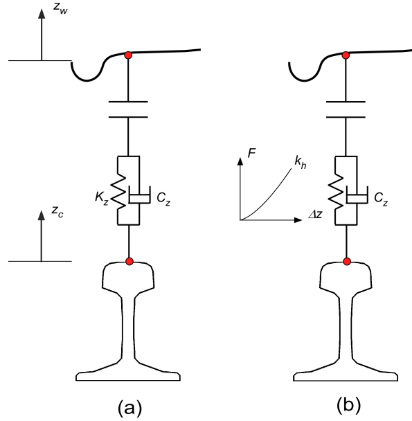
Figure 4.10: Modelling of the contact stiffness in VOCO: (a) standard model, (b) new model with Hertzian stiffness
