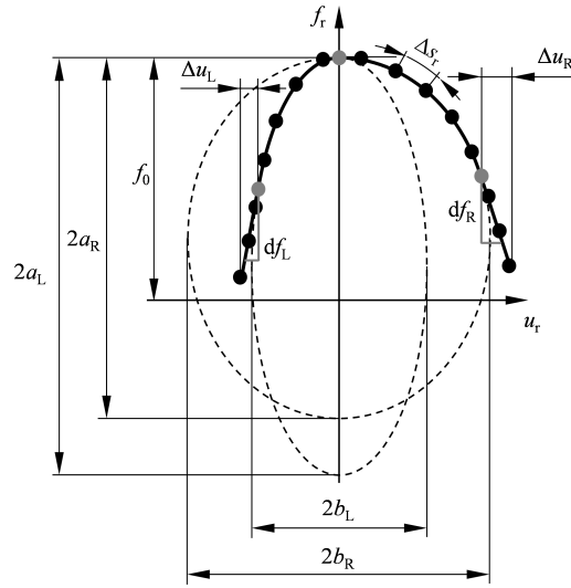
Figure E.2: Schematic representation of the rail profile parametrization. From [145]
