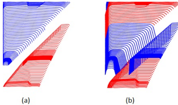
Figure 4.25: 3D geometry interpolation for variable rail profiles: (a) separation of profiles into bodies, and (b) using section breaks. Adapted from [102]
