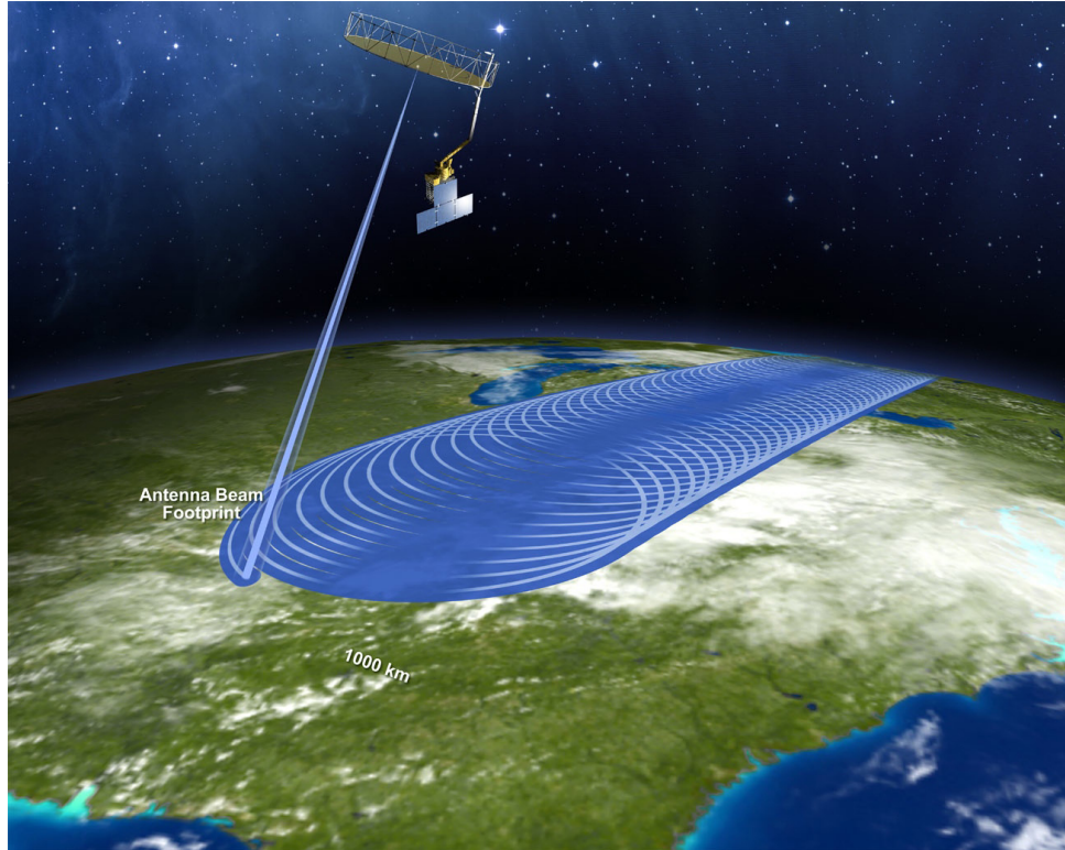
FIGURE 1.3: Artist's conception of SMAP. The SMAP spacecraft has a 1000 km swath width providing a radiometer footprint of about \sim 36 km with 3-day revisit time.
