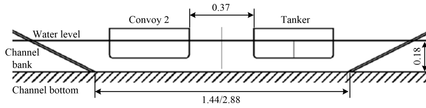
Figure 5.17: Channel dimension and water depth setups for the head-on encounter.
