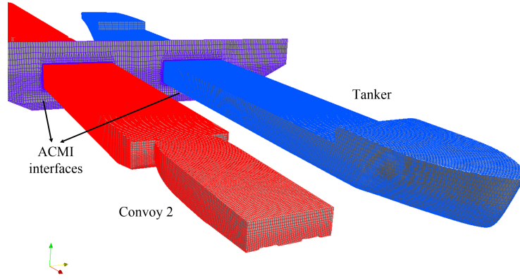
Figure 5.19: Computational mesh and ACMI positions.
