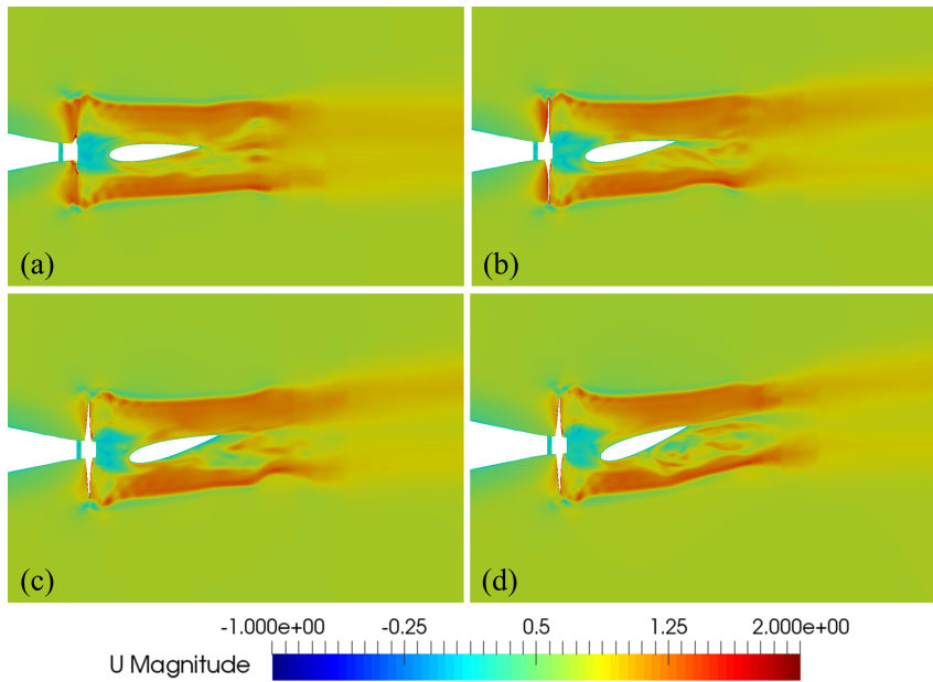
Figure 6.14: Velocity contours at the propeller position in the rudder force tests. The rudder angle (a) \delta = 5^\circ ; (b) \delta = 10^\circ ; (c) \delta = 15^\circ ; (d) \delta = 20^\circ .
