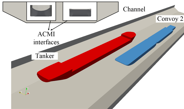
Figure 5.18: Computational domain and ACMI positions for the head-on encounter case between two inland vessels.
