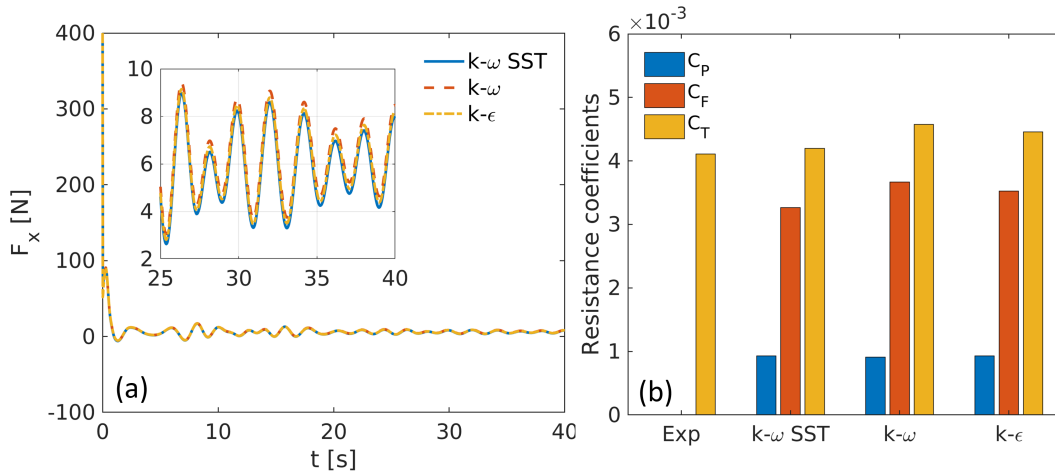
Figure 4.14: (a) Convergence histories of the drag ( F_x ) and (b) comparison of resistance coefficients with different turbulence models. C_T, C_F, C_P are the total, frictional and pressure resistance coefficients respectively. The experimental data can be found in Pereira et al. (2007).
