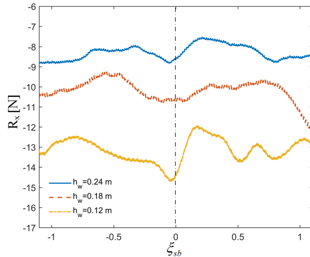
Figure 5.36: Ship resistance ( R_x ) with the relative position ( \xi_{sb} ) under different water depths ( h_w ). The velocity and draught of the convoy 2 are 0.91\text{ m/s} and 0.04\text{ m} respectively. The pile distance is 0.8\text{ m} .
