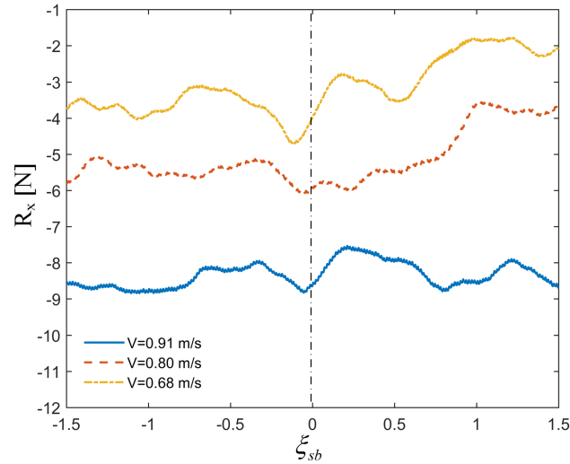
Figure 5.35: Ship resistance ( R_x ) with the relative position ( \xi_{sb} ) under different vessel speeds ( V ). The draught and water depth of the convoy 2 are 0.04\text{ m} and 0.24\text{ m} respectively. The pile distance is 0.8\text{ m} .
