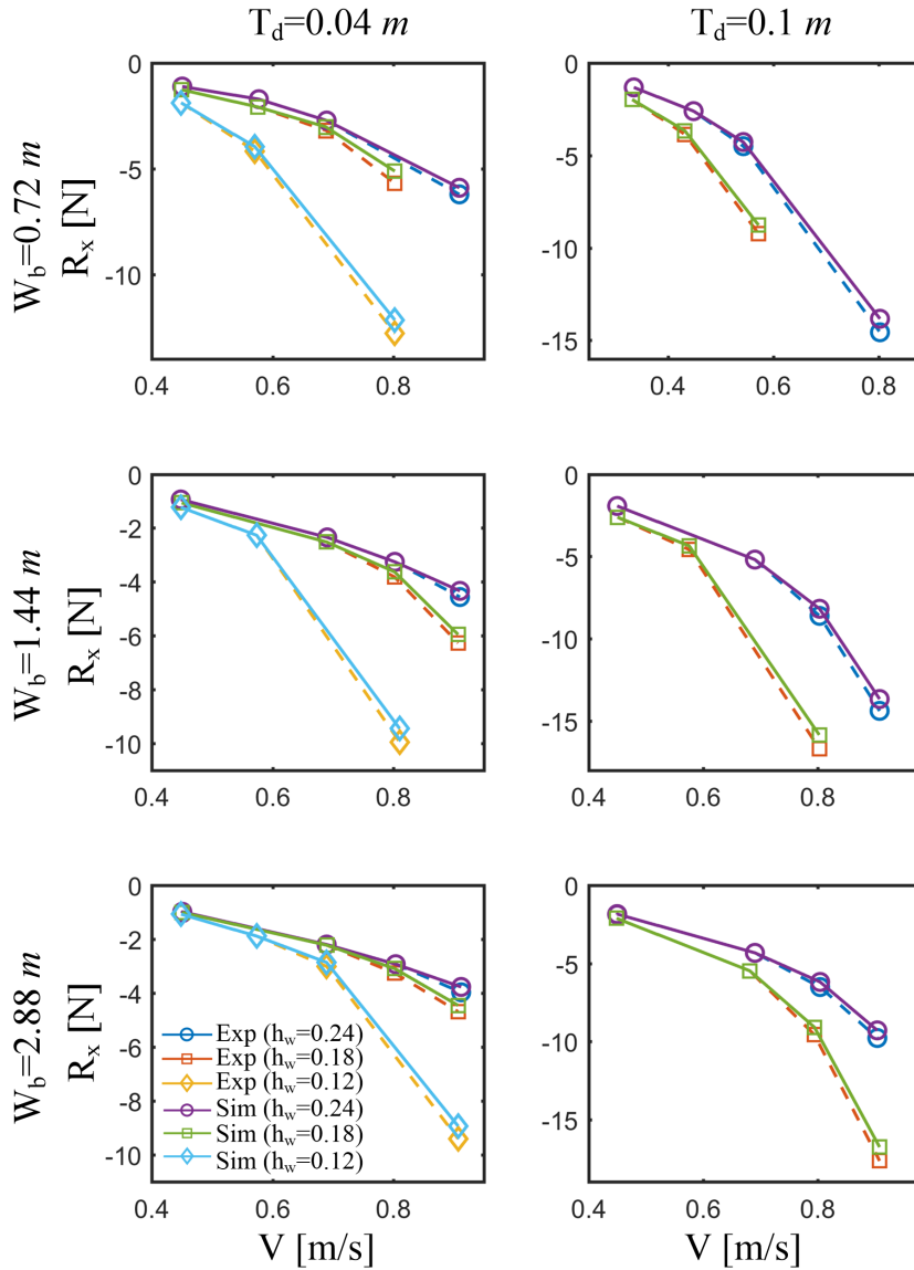
Figure 5.7: Experimental and numerical resistances of the convoy 1. T_d , W_b , R_x , h_w and V are the draught, channel bottom width, resistance, water depth and ship speed respectively.
