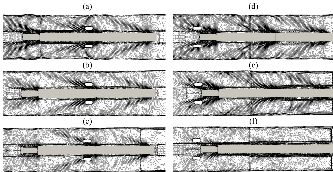
Figure 5.37: Ship-generated waves with different speeds. \xi_{sb} = 0 for (a), (b), (c). \xi_{sb} = 1 for (d), (e), (f). V = 0.907 m/s for (a), (d). V = 0.793 m/s for (b), (e). V = 0.684 m/s for (c), (f). The draught, water depth and pile distance are 0.04, 0.24 and 0.8 m respectively.
