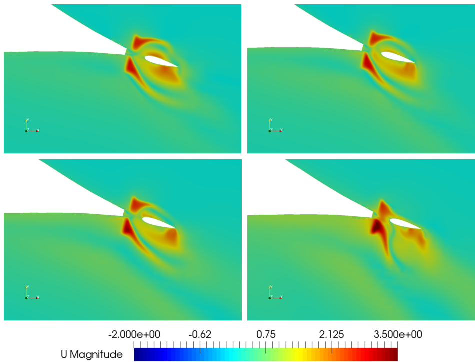
Figure 6.10: Velocity contours at the actuator disk position in CMT (Circular Motion Tests). The drift angle (a) \beta = 0^\circ ; (b) \beta = 4^\circ ; (c) \beta = 12^\circ ; (d) \beta = 20^\circ . The yaw rate r' = 0 .
