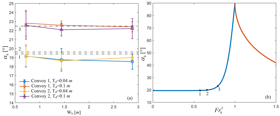
Figure 5.13: (a) Wave angles ( \alpha_k ) of the convoy 1 and convoy 2 with different draughts ( T_d ) and channel bottom widths ( W_b ). The vessel speed V = 0.91 m/s. (b) Theoretical prediction of the wave angle depending on the depth-Froude number ( Fr_h^T ). Line/point 1 is the original theoretical wave angle which is irrelevant with the draught. Lines/points 2 and 3 are the new values calculated based on the modified equation 5.3.
