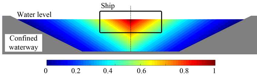
Figure 2.11: Confinement effect distribution in the cross section (Lataire et al. , 2015).
