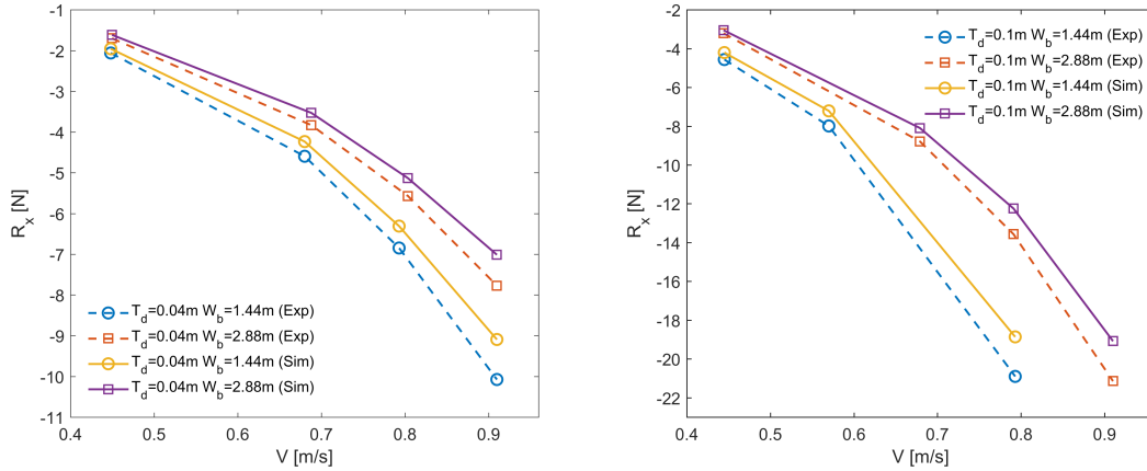
Figure 5.21: Comparison between experimental and numerical resistances of the convoy 2 during the head-on encounter. R_x, T_d, W_b, V are the ship resistance, draught, channel bottom width and speed respectively. The draught of the tanker is 0.07\text{ m} .
