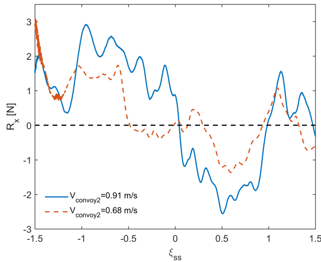
Figure 5.22: Resistance ( R_x ) of the convoy 2 with the relative position ( \xi_{ss} ) under different vessel speeds ( V_{convoy2} ). The velocity of the tanker is 0.5 m/s . The channel bottom width is 1.44 m . The draughts of the convoy 2 and the tanker are 0.04 and 0.07 m .
