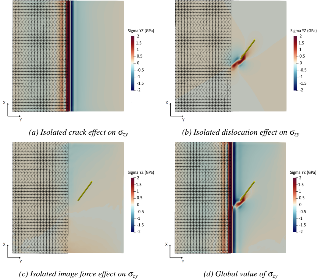
FIGURE 5.3 – Decomposition of the stresses affecting K_{II} on the crack tip. Crack surface is represented by the black wireframe, and the dislocation (Class I (CB(a)) with a Burgers vector of b = \frac{1}{2}[10\bar{1}] ) by the yellow line \varepsilon = 0.01892208
