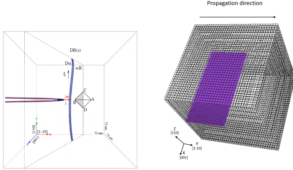
FIGURE 4.18 – (a) Atomistic mesh, the dislocation displayed is just an illustration and does correspond to the studied dislocation [16]. (b) XFEM mesh, the purple plane corresponds to the crack position
