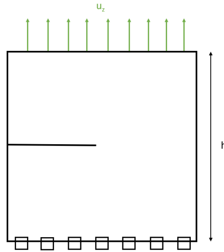
FIGURE 4.2 – Boundary conditions used for the DDD calculations. The bottom nodes are all fixed and a vertical displacement of magnitude u_k = h \times \epsilon is applied to the top nodes
