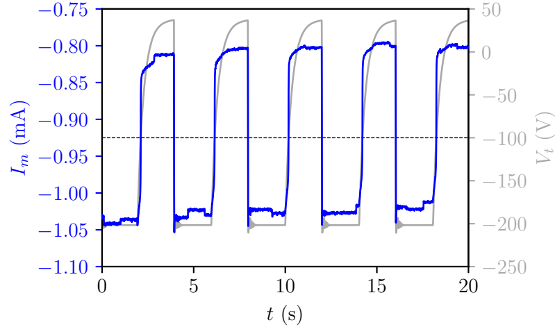
Figure 4.6: Example measurement of the temporal evolution of the current with an aluminum target bombarded by a 0.7 keV beam (blue). The target voltage, V_t , is also shown for sake of clarity (gray). The dashed line marks the grid voltage, V_g = -100 V.
