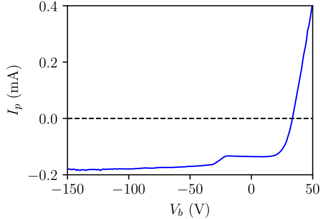
Figure 3.13: Measured IV curve for the determination of the probe bias voltage.
