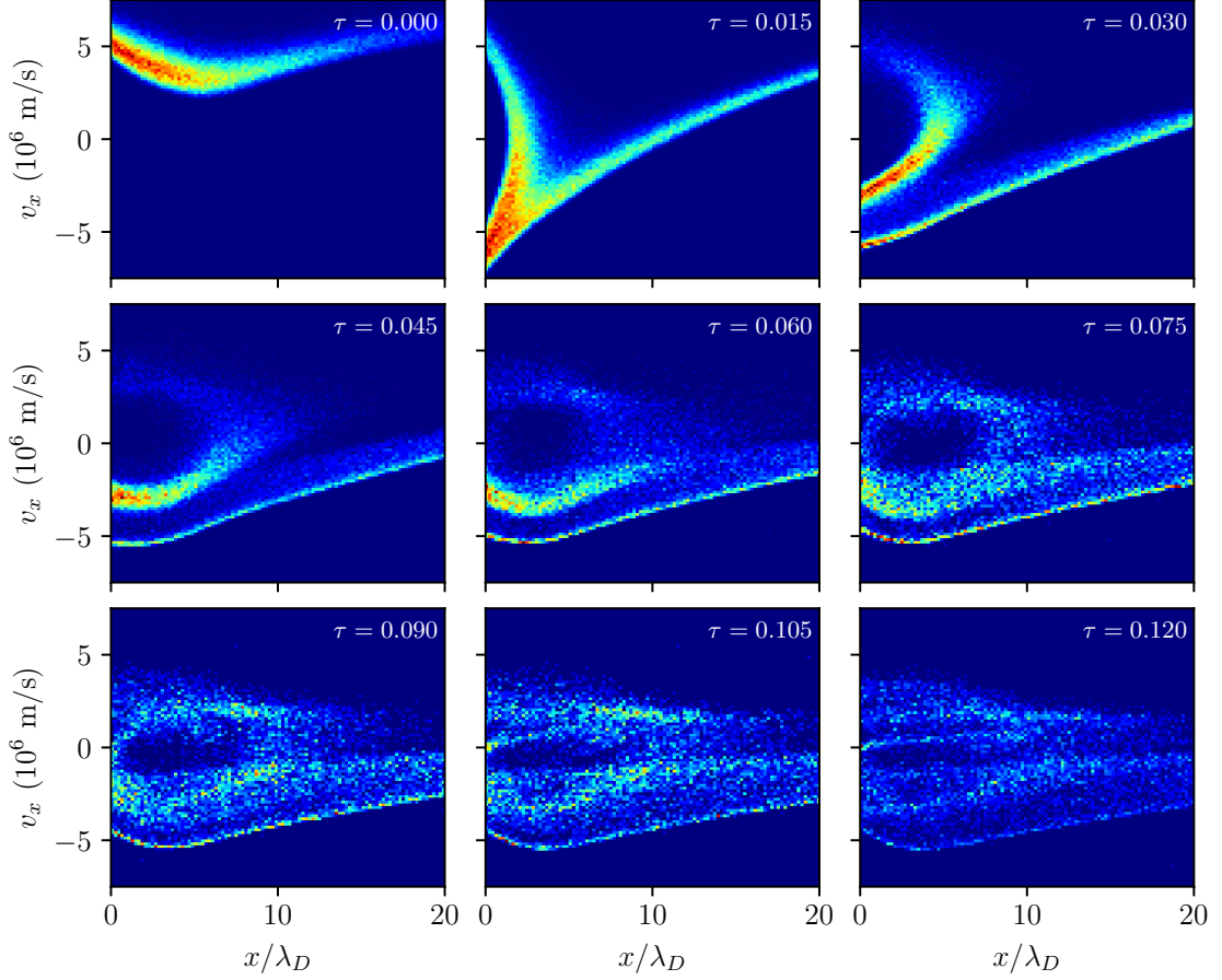
Figure 2.20: Particle density in the x - v_x phase-space during the first RF cycle of the simulation. Here \tau = (t - t_0)/T and t_0 = 25 ns.
