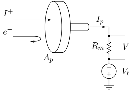
Figure 3.6: Generic schematic of a planar probe.
