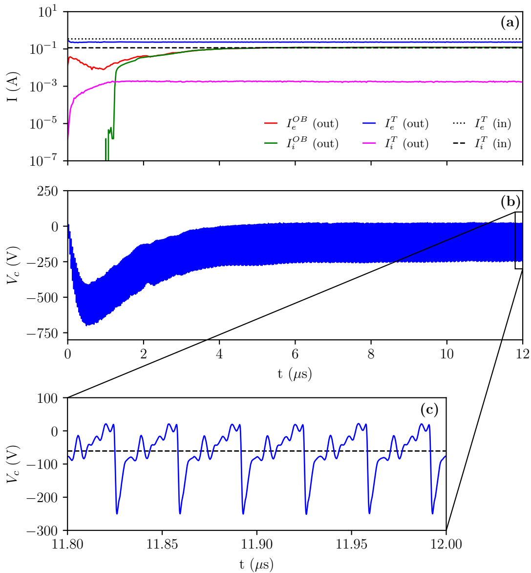
Figure 2.17: Temporal evolution of voltages and currents in the nominal RF plume simulation. (a) shows the average ion and electron current entering and leaving the domain through each boundary. The average is done over one RF cycle. Superscript OB refers to the outer boundary and T to the thruster boundary. (b) shows the capacitor voltage, V_c . (c) shows the detailed view of the voltage capacitor between 11.8 \mu\text{s} and 12 \mu\text{s} , and the dashed line marks the average capacitor voltage at steady-state \langle V_c \rangle = -60.51 V.
