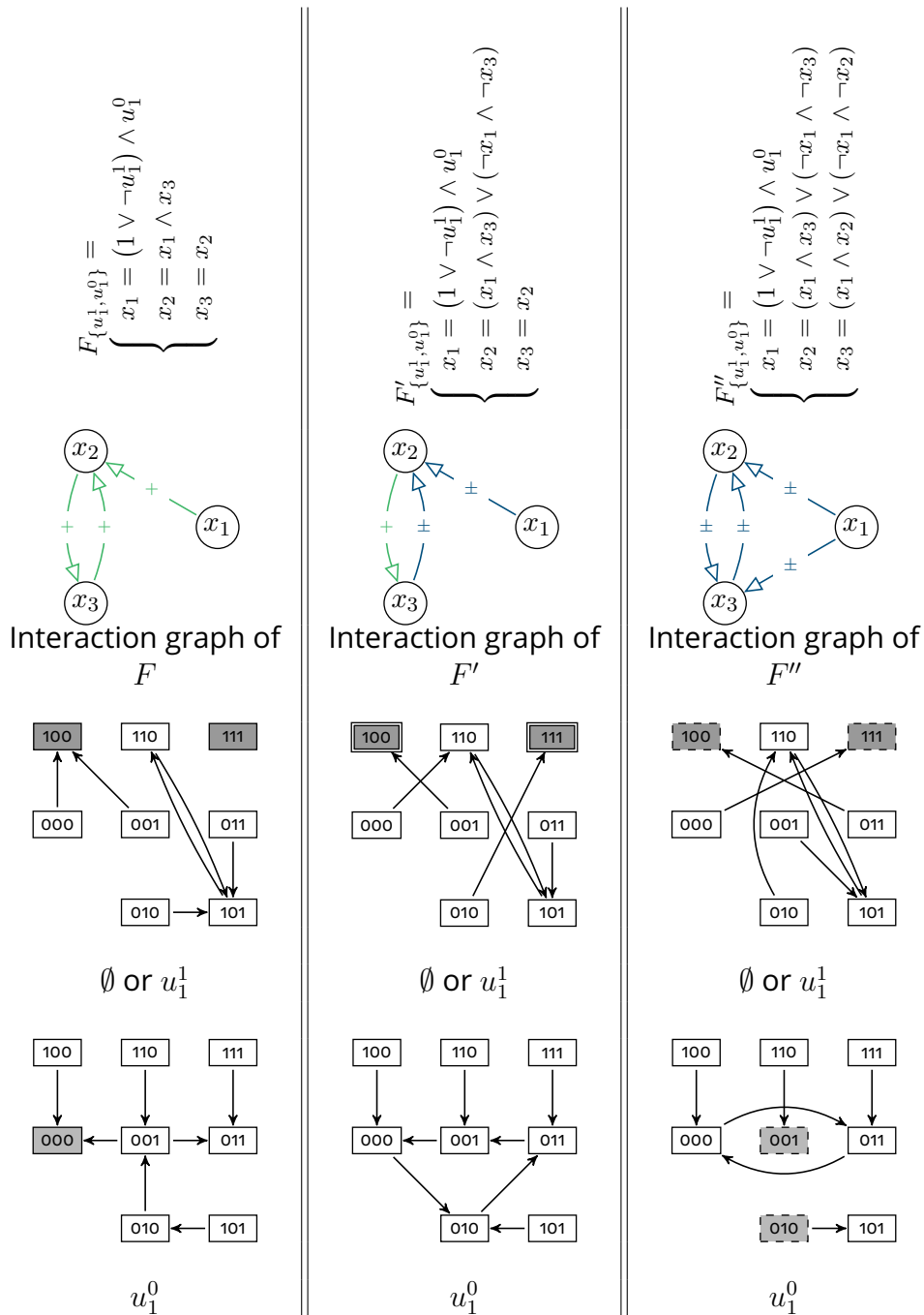
Legend: The synchronous dynamics of Boolean control networks F_{\{u_1^1, u_1^0\}} , F'_{\{u_1^1, u_1^0\}} , and F''_{\{u_1^1, u_1^0\}} . The dynamics are synchronous and the self-loops on states are not shown. The stable states of each dynamics are coloured in two shades of grey, and their contours are drawn in different styles. Each shade of grey is associated with different control input and each contour style is associated with a different Boolean network.
