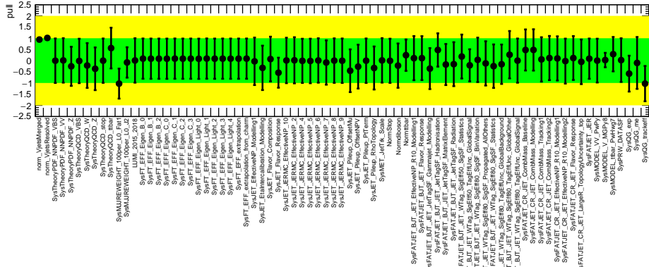
(a) Asimov
