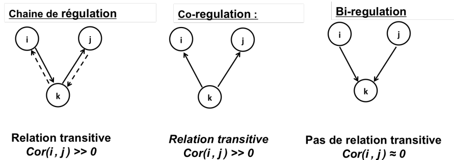
FIGURE 3.5 – Relations causales et transitives
