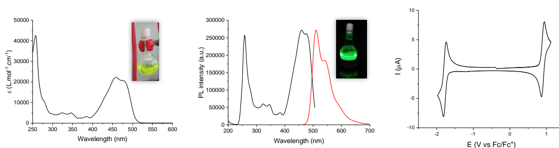
Figure 4.2. UV-Vis absorption (left) and emission (center) spectra in \text{CH}_2\text{Cl}_2 and cyclic voltammogram (right) in 0.1 \text{ M Bu}_4\text{NPF}_6/\text{CH}_2\text{Cl}_2 (100 mV/s scan rate, Pt working electrode) of BTXI .
