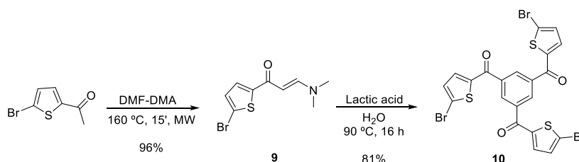
Scheme 3.4. Synthetic pathway used to obtain the tri-brominated central core 10 .
