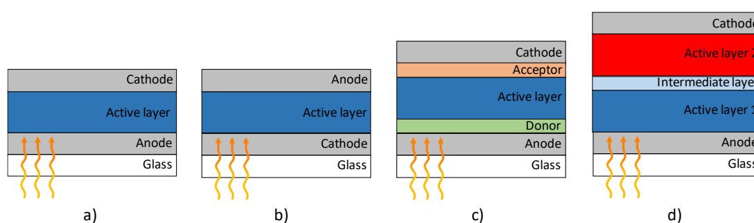
Figure 1.9. Schematic structure of direct (a), inverted (b), PMHJ (c) and multi-junction (d) devices.
