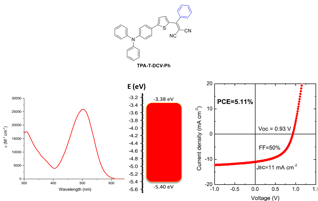
Figure 3.1. Summary of the most relevant properties of TPA-T-DCV-Ph : UV-Vis absorption spectrum in CH 2 Cl 2 (left), energetic levels obtained by CV in CH 3 CN/o-C 6 H 4 Cl 2 1:4 (center) and J-V curve and photovoltaic parameters of an ITO/MoO 3 /TPA-T-DCV-Ph:C 70 /BCP/Al device (right).
