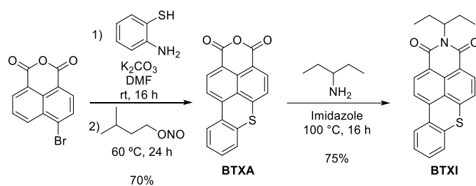
Scheme 4.1. Optimized synthetic pathway used to obtain BTXI.
